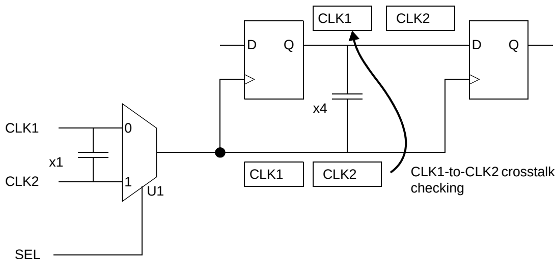
Figure 14-16 Circuit with multiplexed clocks
