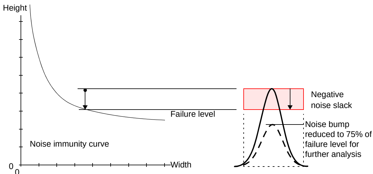
Figure 14-36 Input noise bump reduction for propagation analysis
