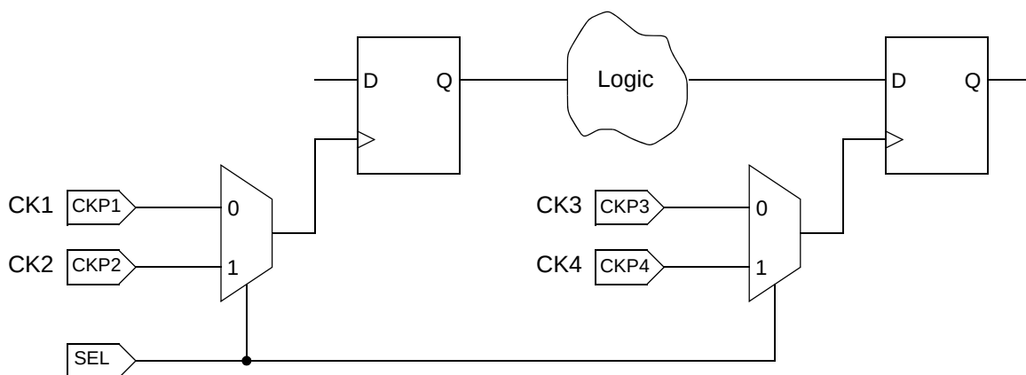
Figure 6-10 Four clocks and one selection signal
