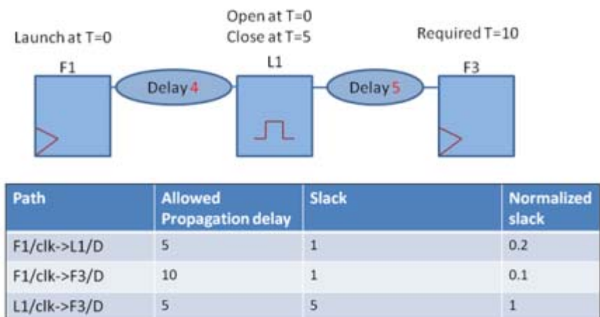
Figure 15-33 Example of normalized slack
