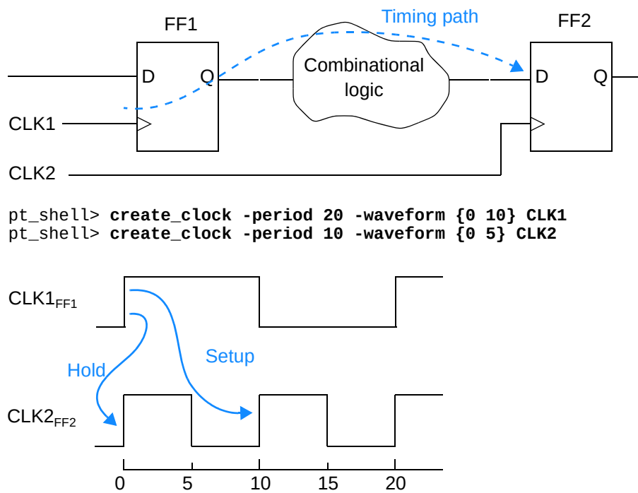
Figure 7-10 Delay requirements with 20ns/10ns clocks
