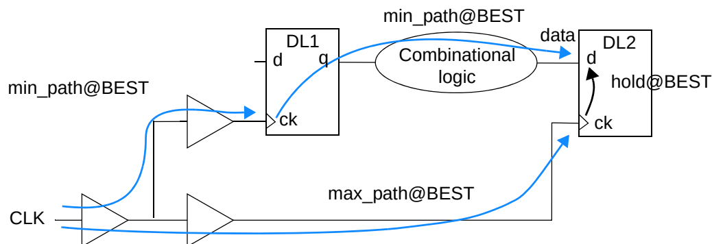
Figure 8-6 Timing path for one operating condition – best case
