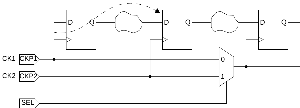
Figure 6-12 Multiplexed clocks specified with case analysis
