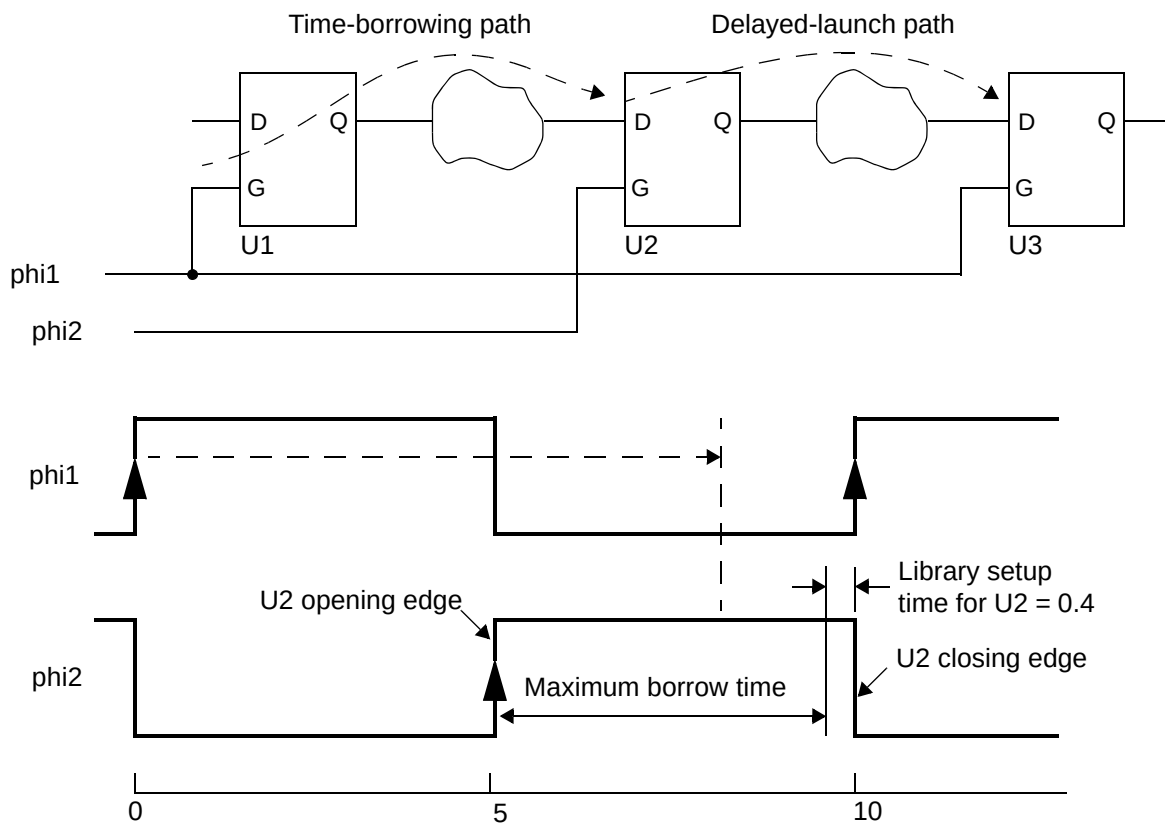
Figure 15-19 Maximum borrow time reduced by setup requirement
