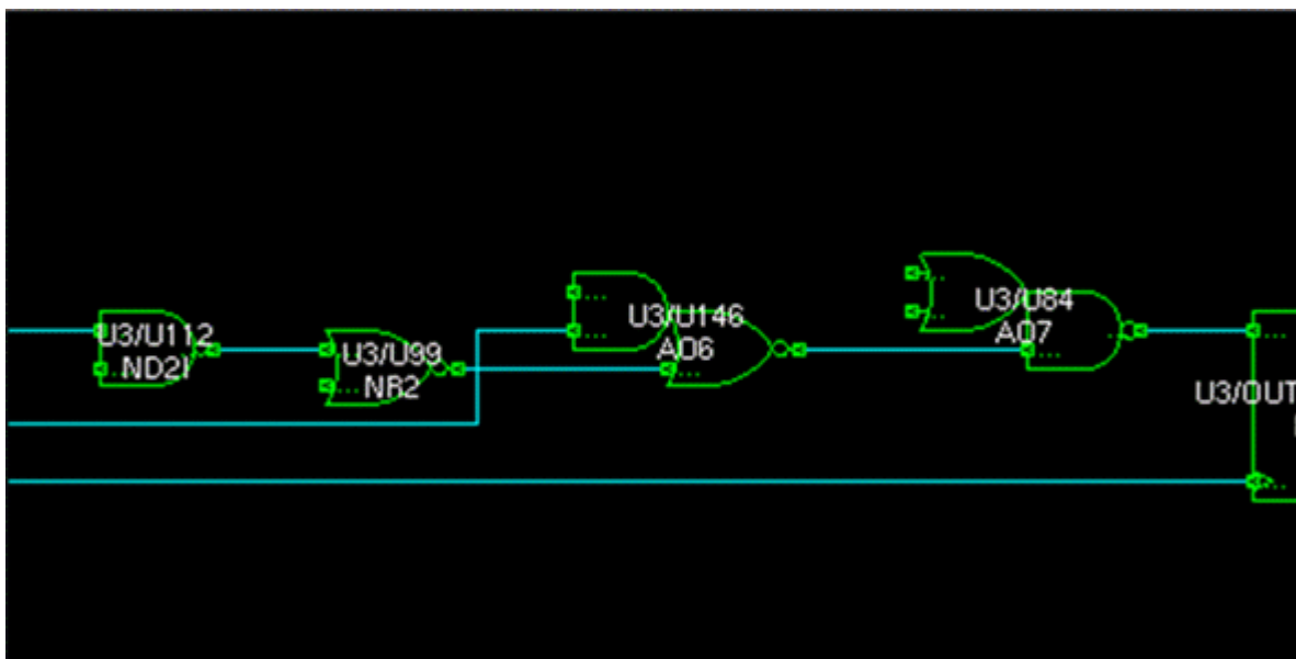
Figure 18-24 Instance Schematic
