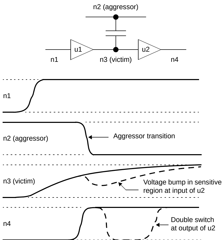
Figure 14-26 Double-switching error example
