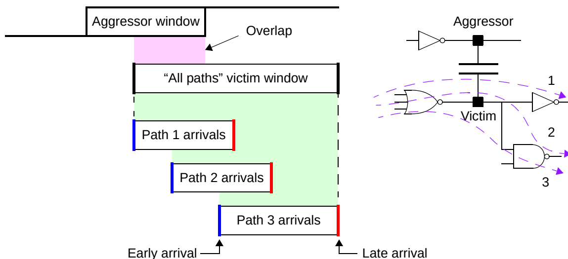
Figure 14-13 “All Paths” (Default) Window Overlap Mode
