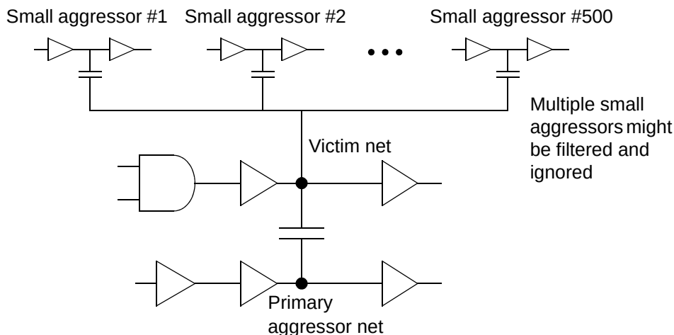
Figure 14-20 Composite aggressor mode disabled
