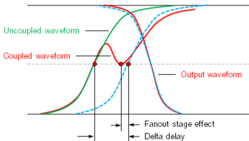
Figure 14-2 Delta delay includes the fanout stage effect
