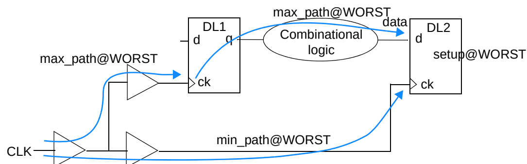
Figure 8-7 Timing path for one operating condition – worst case
