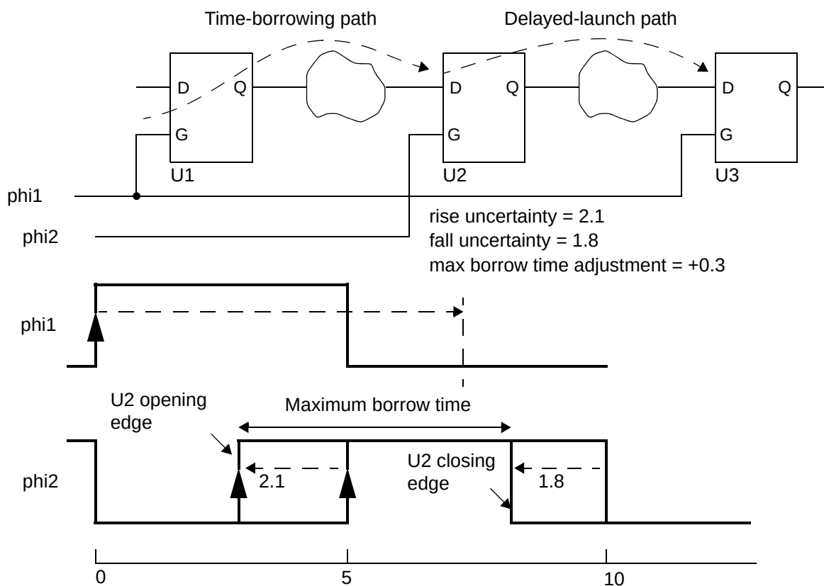
Figure 15-21 Maximum borrow time adjustment for uncertainty
