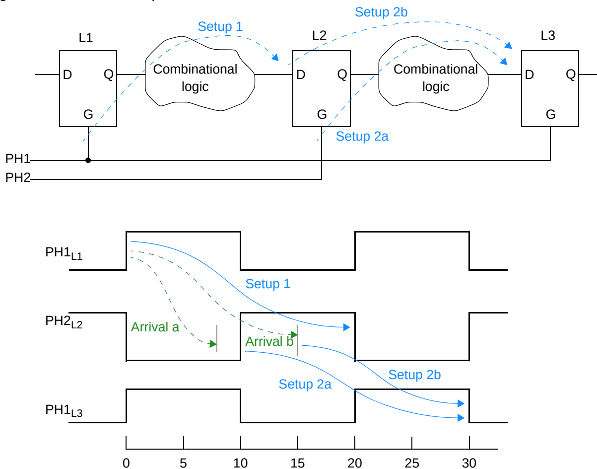
Figure 1-6 Latch-based paths
