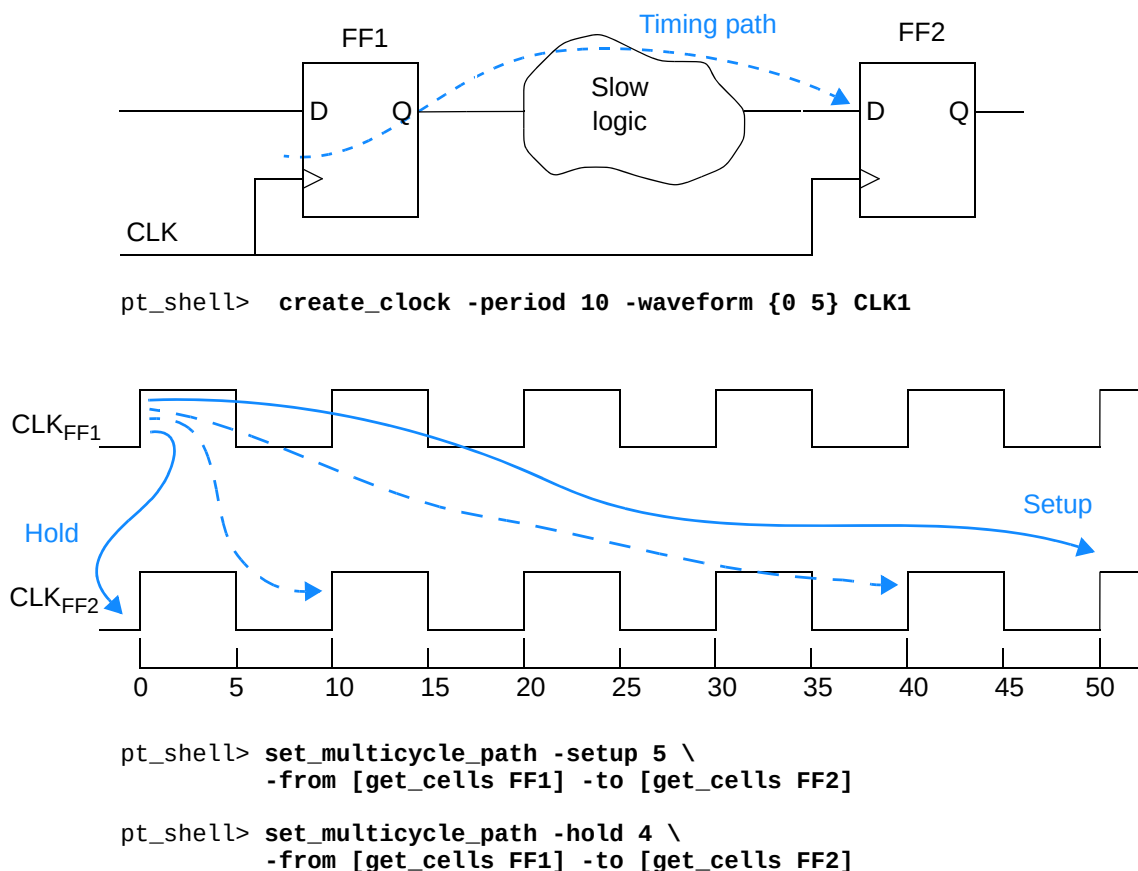
Figure 7-16 Multicycle path taking five clock cycles
