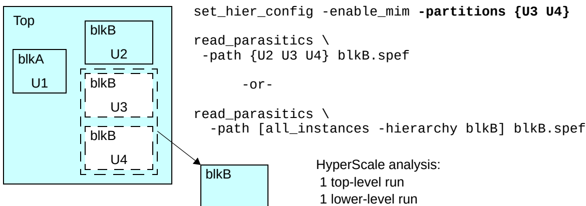
Figure 20-21 MIM Merging for Some Instances of a Block
