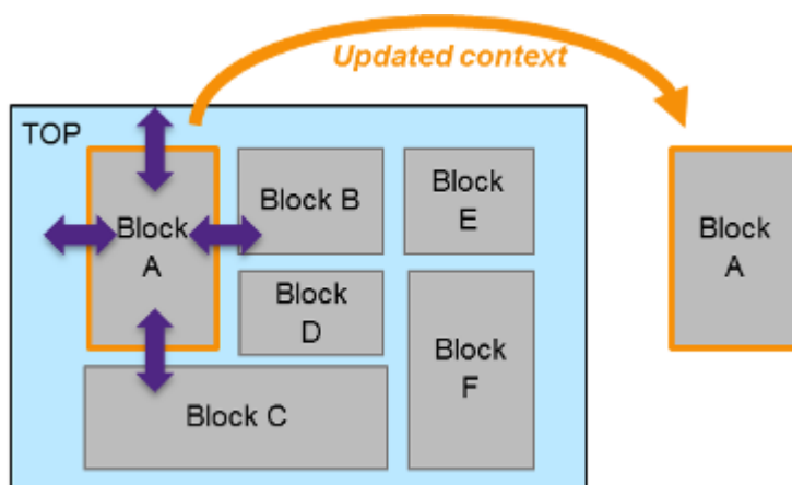
Figure 20-31 HyperScale Top Analysis Provides Updated Block Context for ECO Fixing
