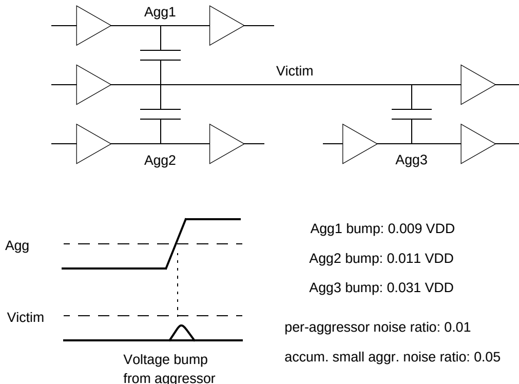
Figure 14-8 Voltage bumps from multiple aggressors
