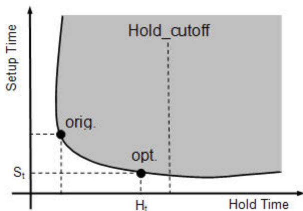
Figure 15-15 Successful setup slack improvement
