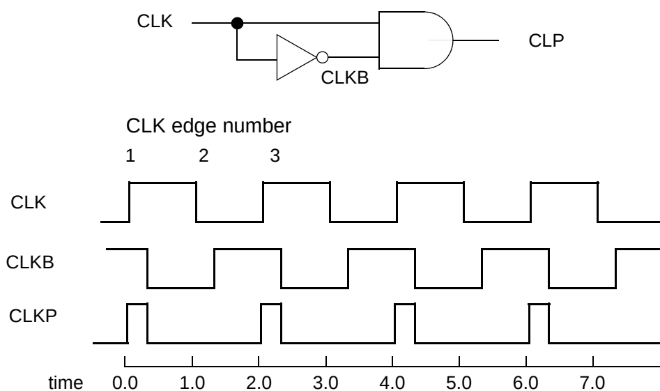
Figure 6-19 Pulse clock specified as a generated clock
