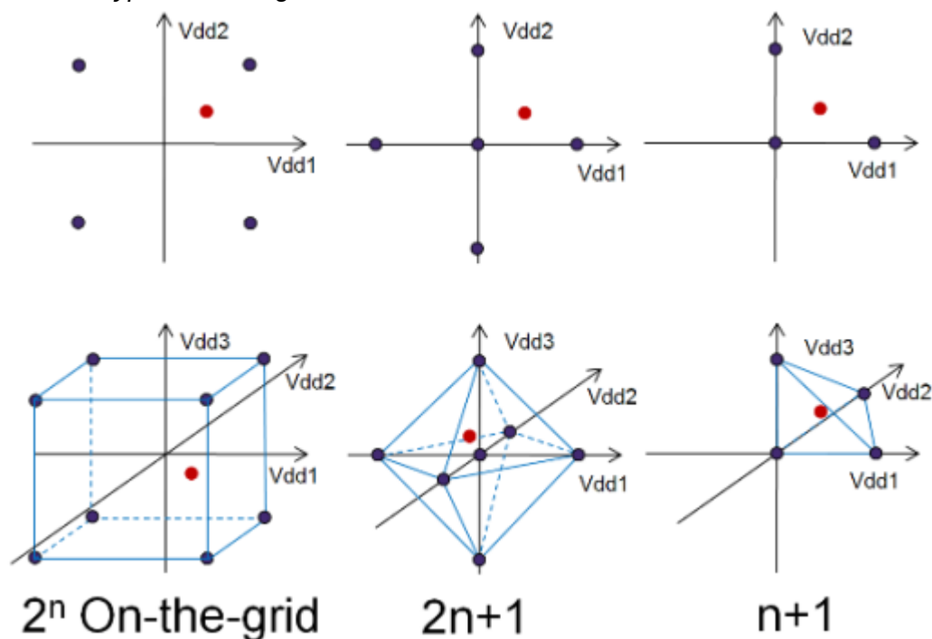
Figure 9-4 Three types of scaling formations
