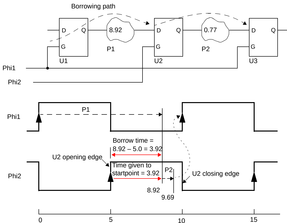
Figure 15-17 Latch-based timing paths
