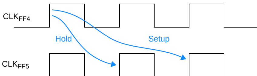
Figure 7-14 Multicycle path hold relationship based on new setup
