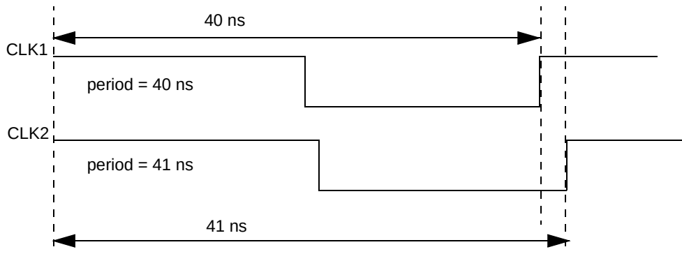
Figure 15-5 Unrelated clock waveforms
