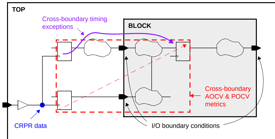
Figure 20-5 HyperScale Block Context
