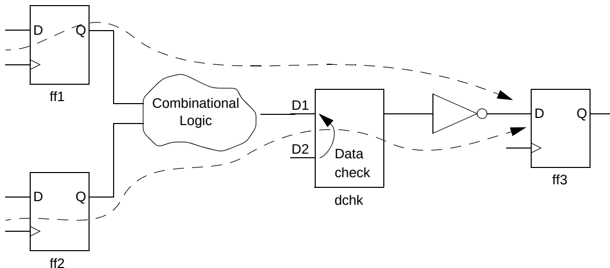
Figure 15-12 Timing paths not broken by data checks
