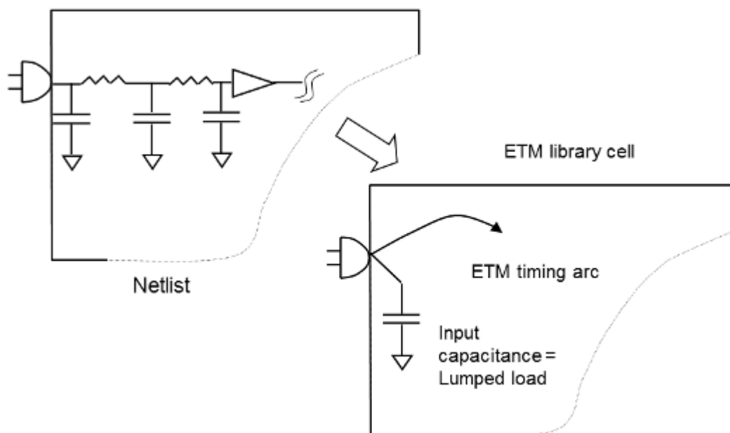
Figure 20-75 Back-Annotated Boundary Nets
