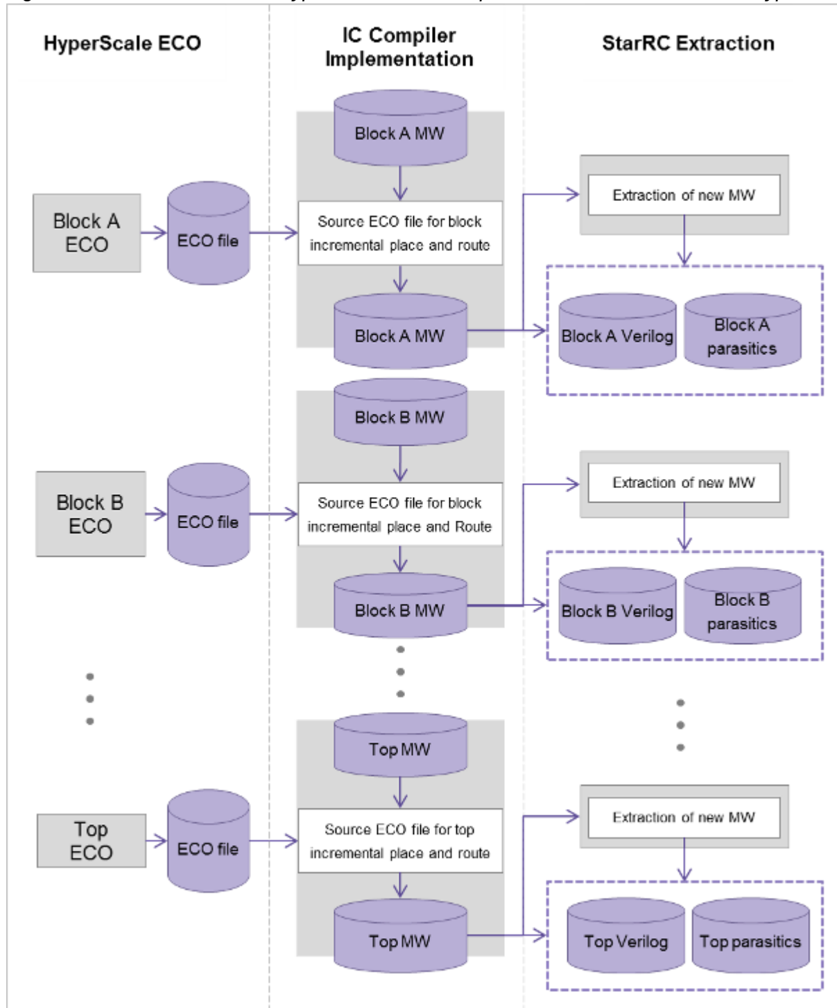
Figure 20-41 Data flow from HyperScale to IC Compiler and StarRC then back to HyperScale
