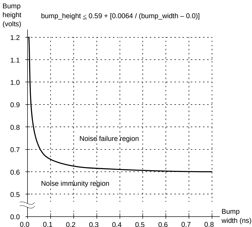
Figure 14-48 Hyperbolic noise immunity curve
