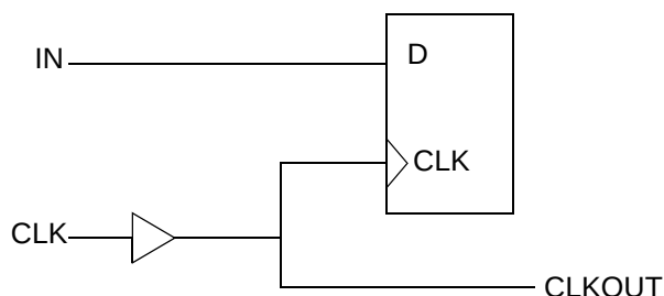
Figure 20-58 Load-dependent clock network
