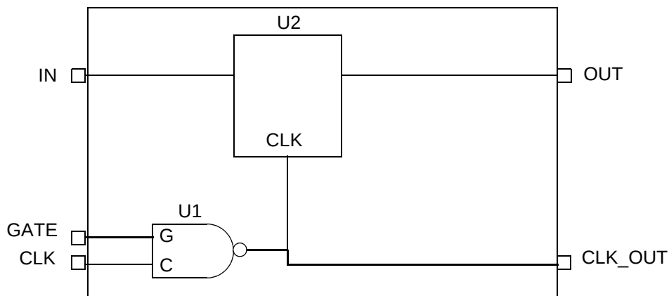
Figure 20-69 Combinational path through clock-gating logic
