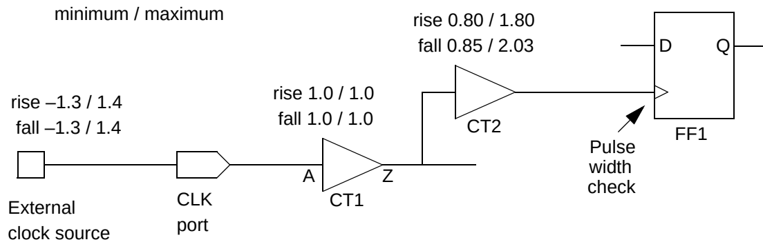
Figure 8-12 Minimum pulse width analysis
