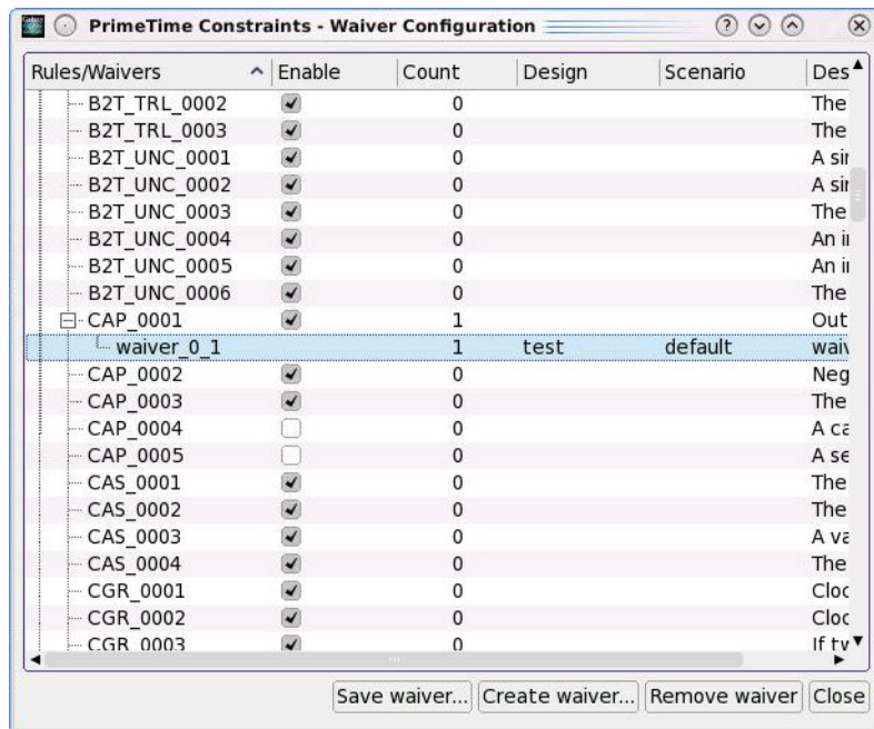
Figure 16-17 Removing a Waiver With the Waiver Configuration Dialog Box
