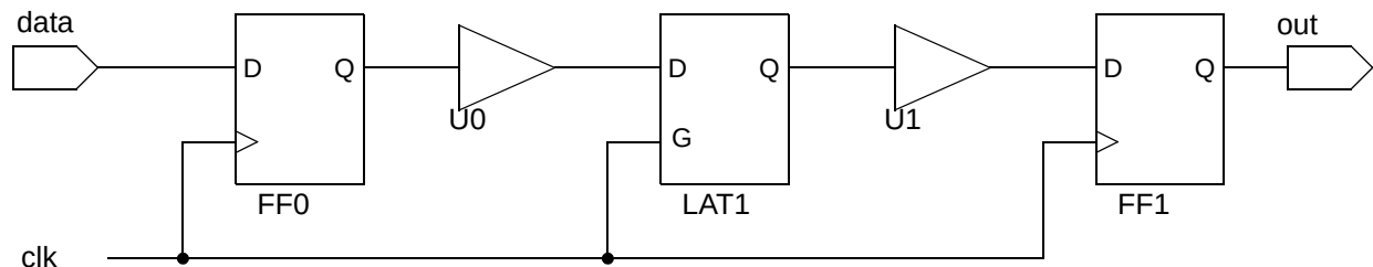
Figure 7-2 Circuit for path specification in example 4
