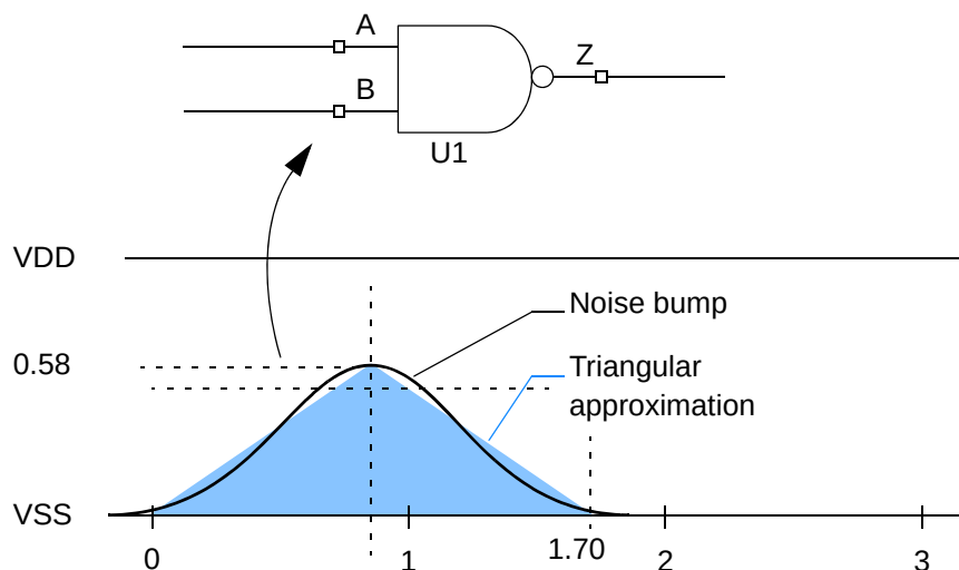
Figure 14-37 Noise bump created with the set_input_noise command
