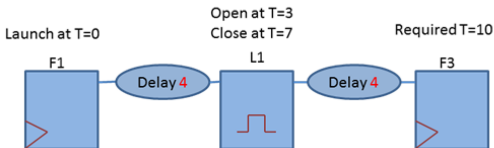
Figure 15-30 Slack example with borrowing
