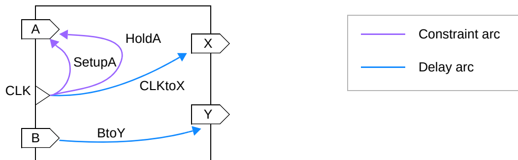
Figure 20-76 Quick Timing Model Representation of a Block
