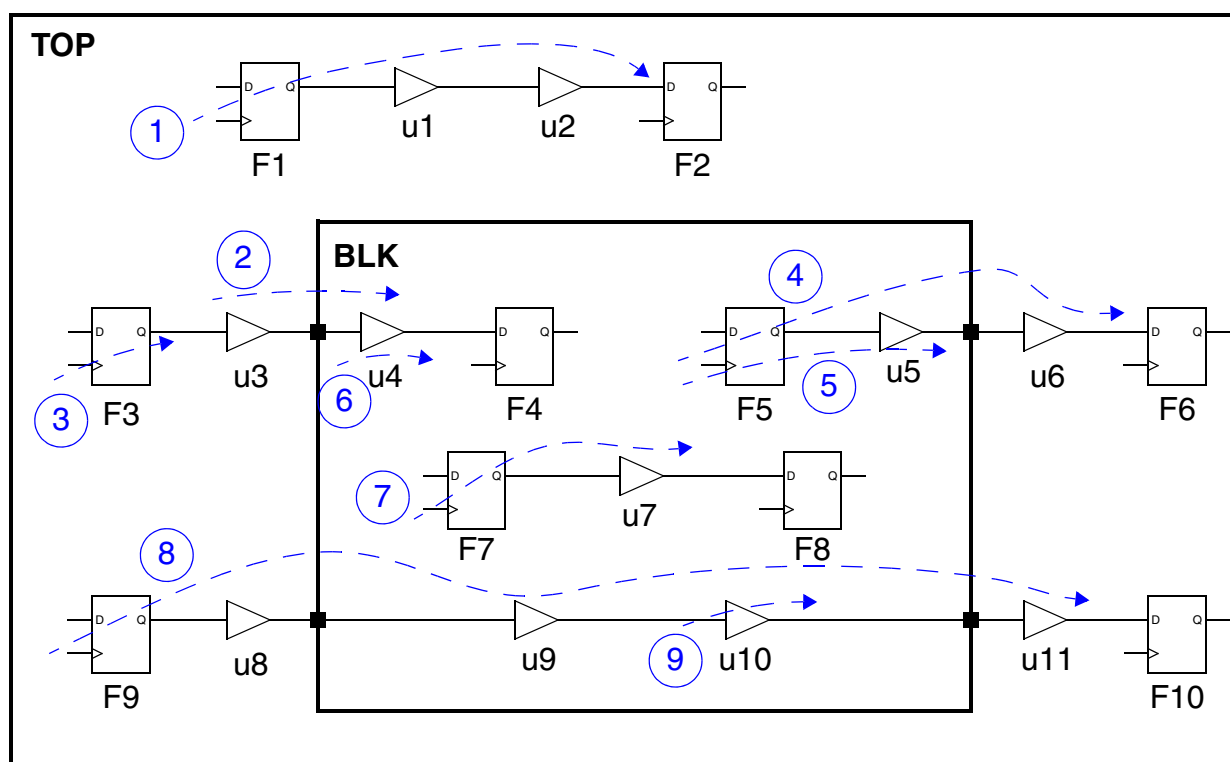
Figure 20-50 Top-Level, Block-Level, and Cross-Boundary Paths
