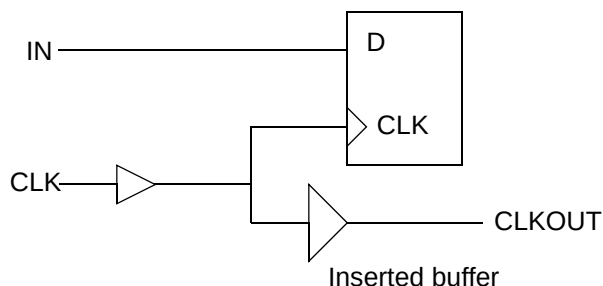
Figure 20-59 Isolating the delay of the clock network
