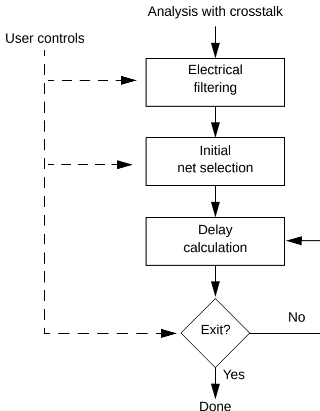
Figure 14-6 PrimeTime SI crosstalk analysis flow
