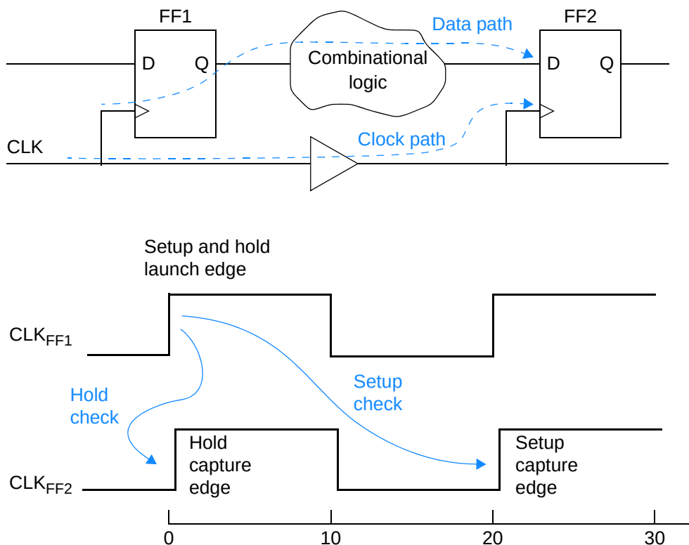
Figure 1-5 Setup and hold checks
