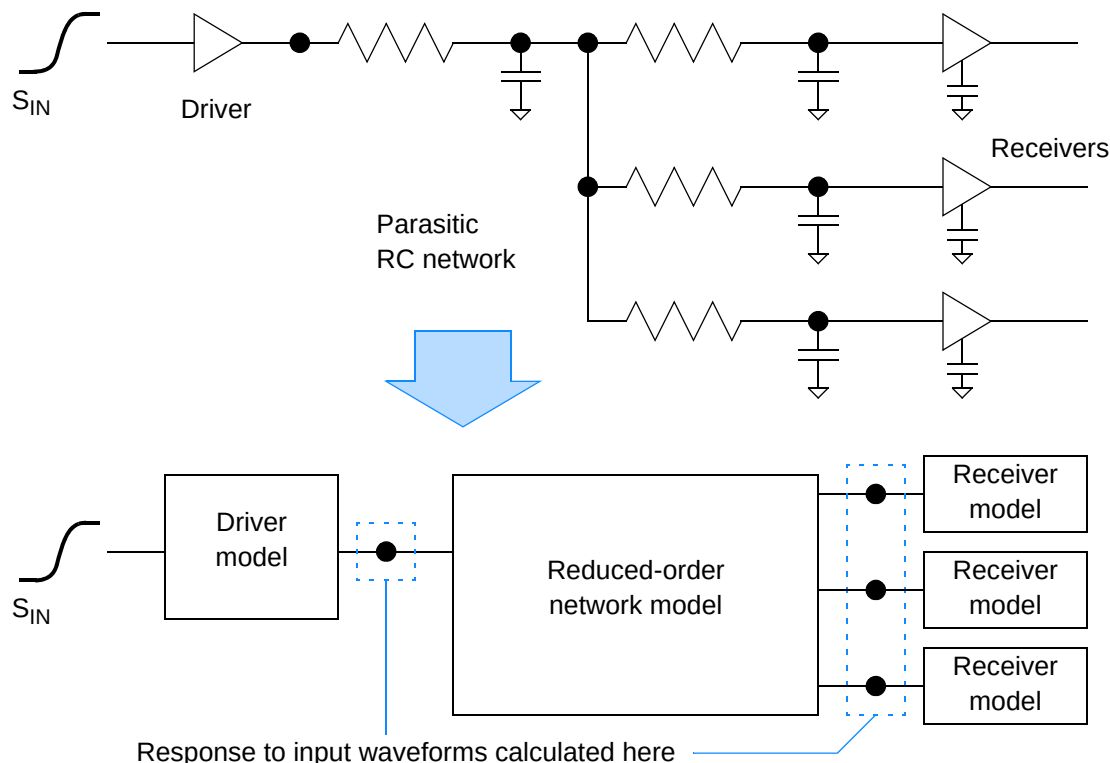
Figure 9-1 Models used to calculate stage delays and slews
