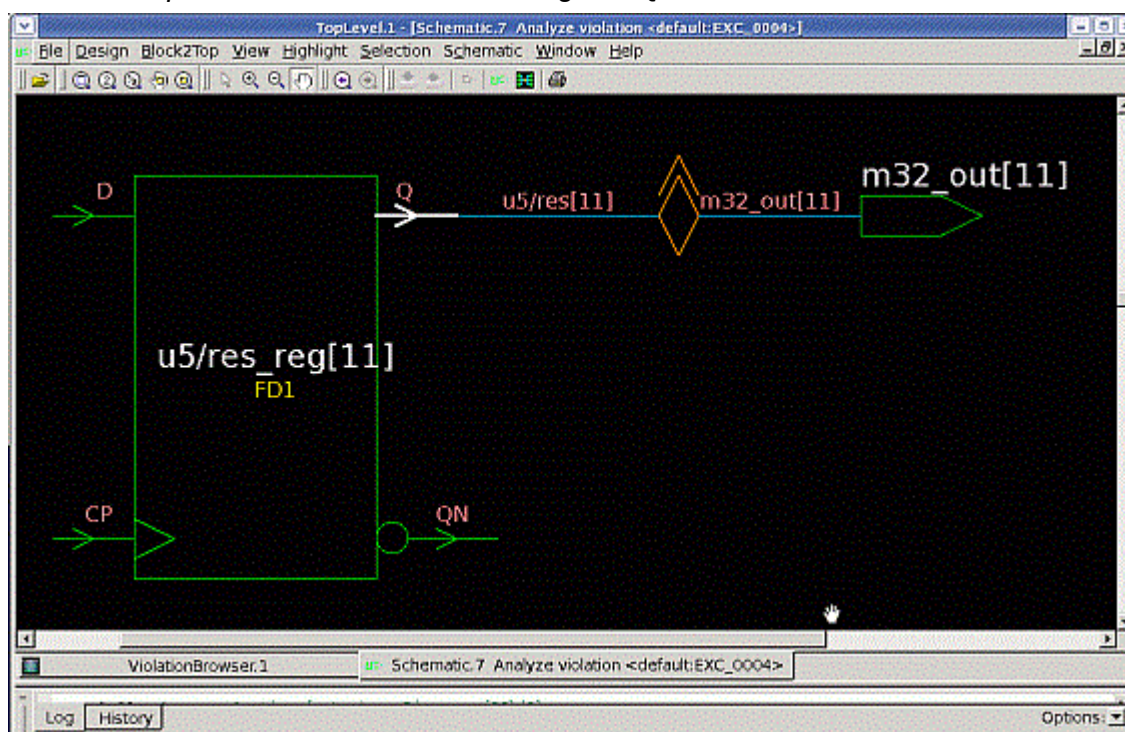
Figure 16-64 Expanded Schematic View of Register Q Pin
