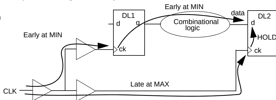
Figure 8-8 Timing path reported during OCV analysis
