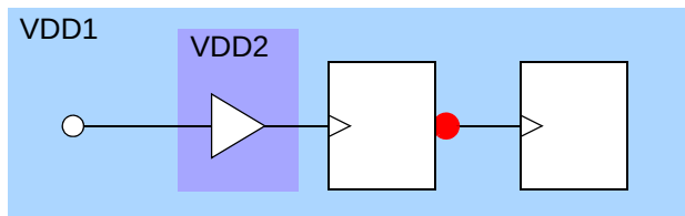
Figure 13-8 Sequential clock network crosses power domains
