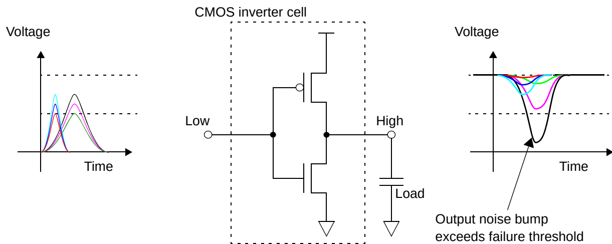
Figure 14-46 Noise immunity characterization of input
