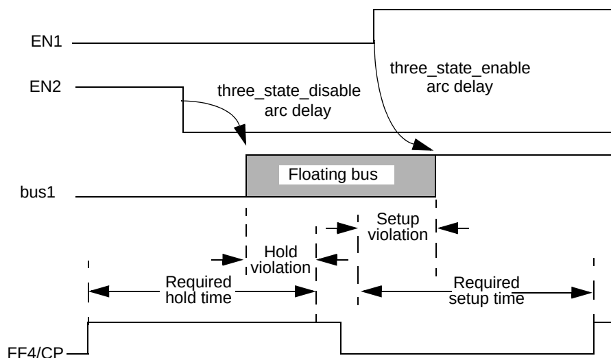
Figure 15-8 Floating bus contention check
