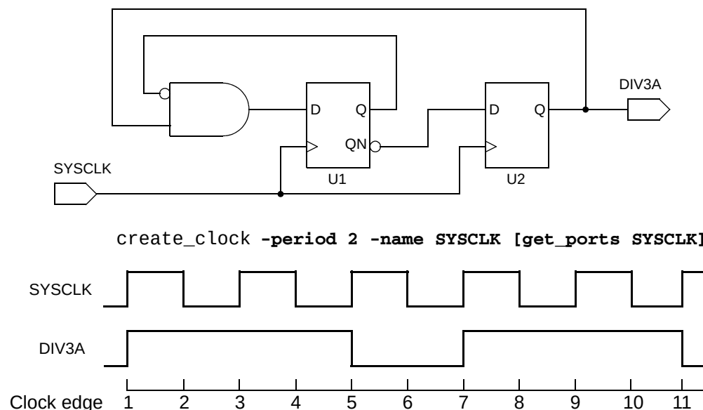
Figure 6-25 Divide-by-3 clock generator
