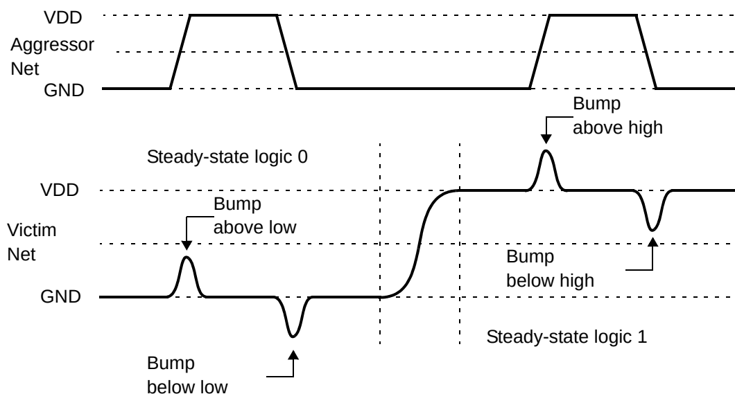
Figure 14-30 Noise bump types
