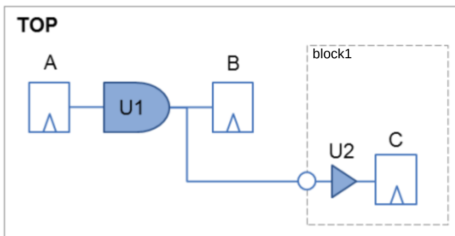
Figure 20-36 Top-level path ECO fixing
