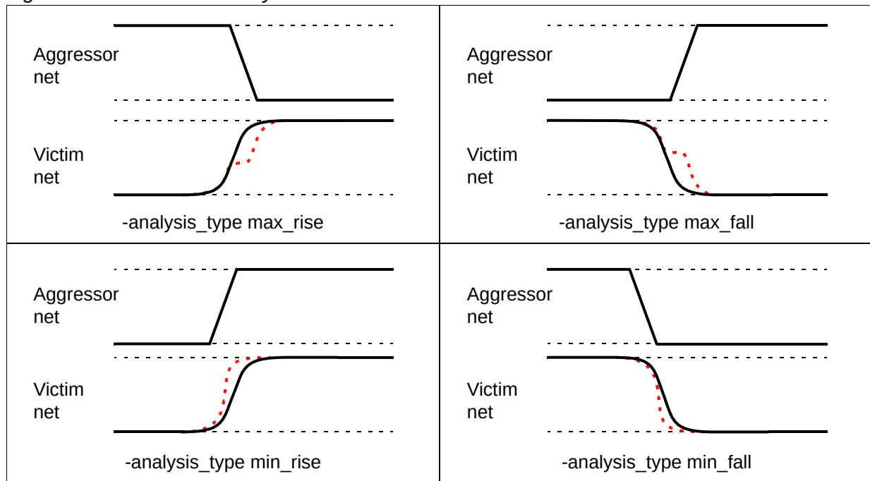
Figure 21-2 Crosstalk delay transitions for arcs
