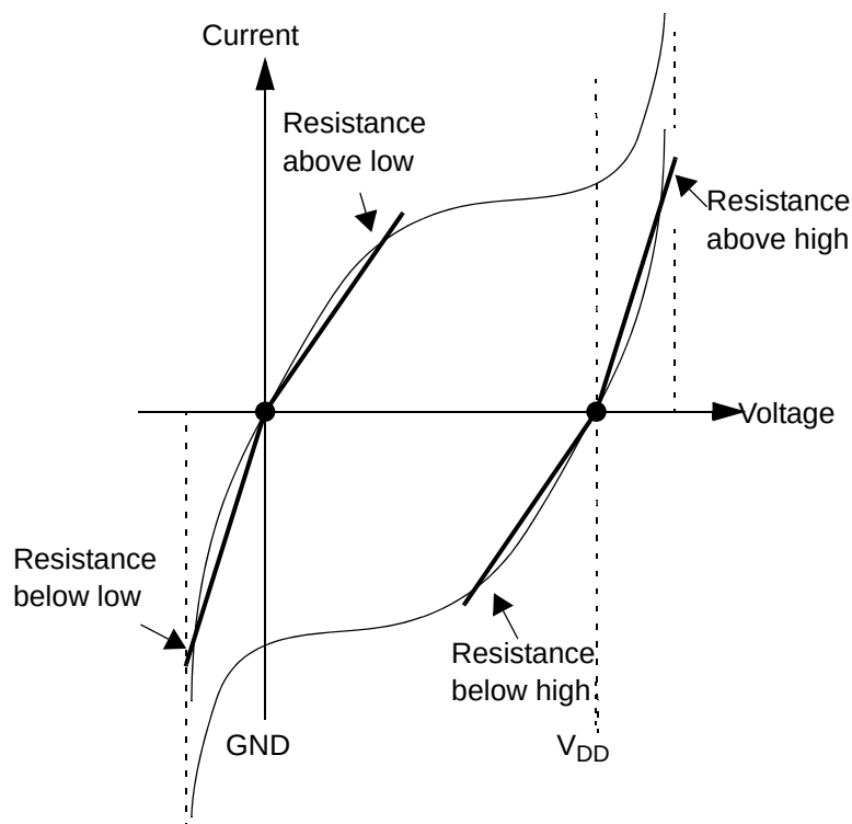
Figure 14-44 Resistance approximation of steady-state I-V characteristics
