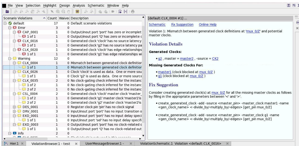
Figure 16-34 Violation Browser
