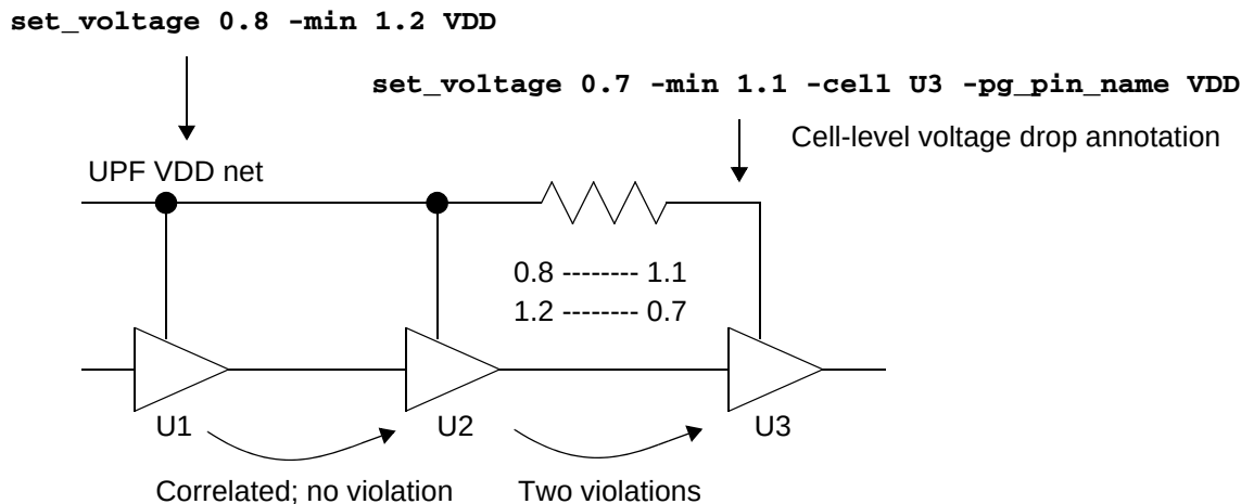
Figure 13-9 Signal level checking with cell-level voltage annotation
