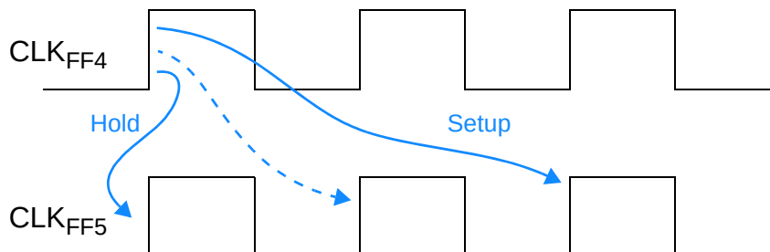
Figure 7-15 Multicycle path hold set correctly
