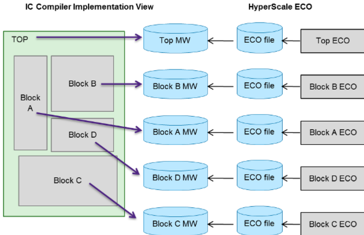
Figure 20-39 Exact Mapping From HyperScale to Physical Implementation
