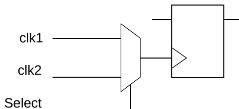
Figure 5-10 Multiple clock fanin
