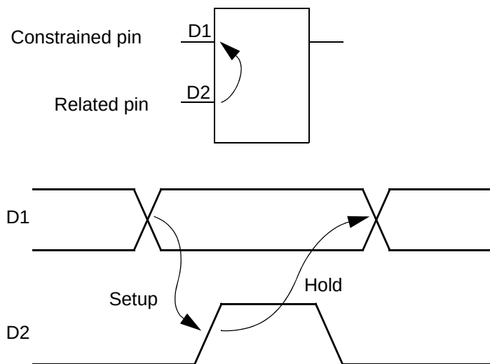
Figure 15-9 Simple data check example
