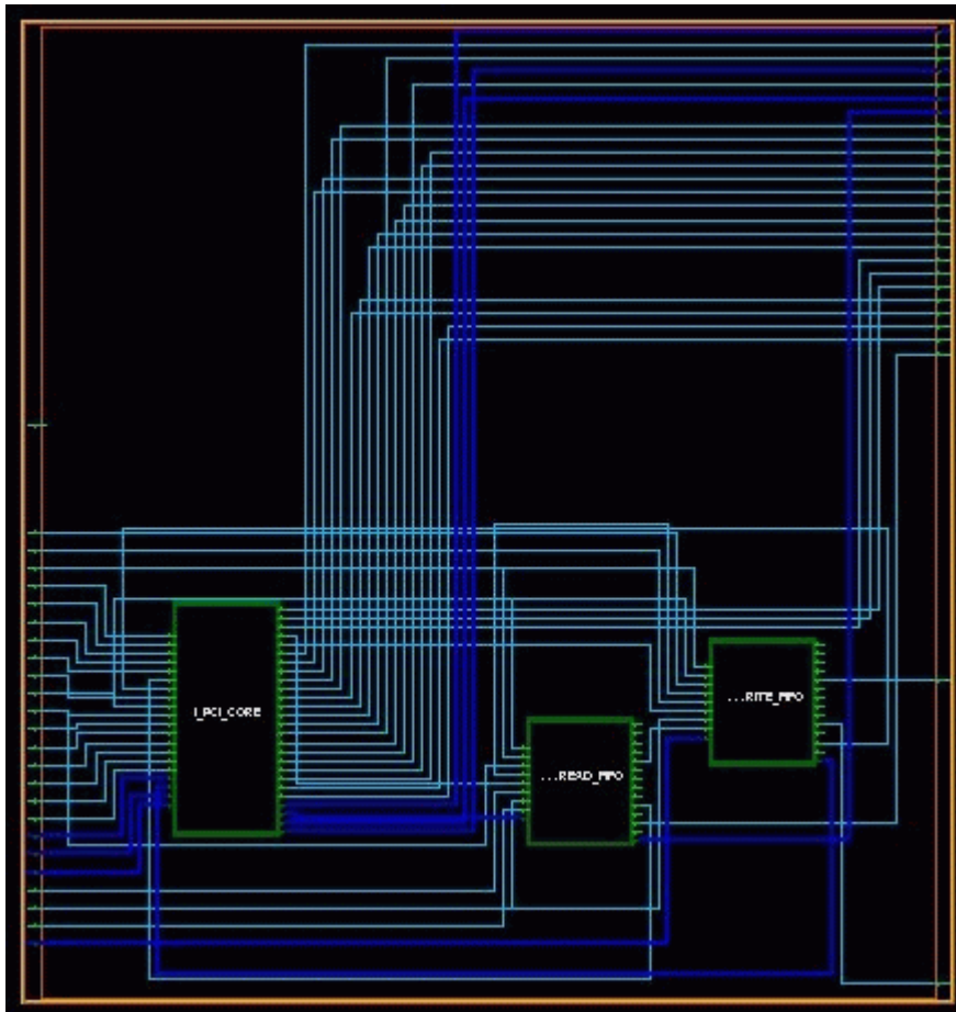
Figure 18-29 Collapsed View of Bus Nets and Pins
