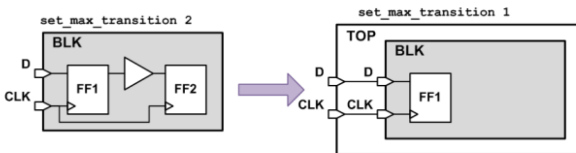
Figure 20-25 Another Manually Fixable Block Boundary Violation
