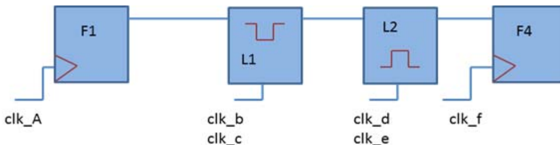
Figure 15-28 Circuit with multiple clocks at latches
