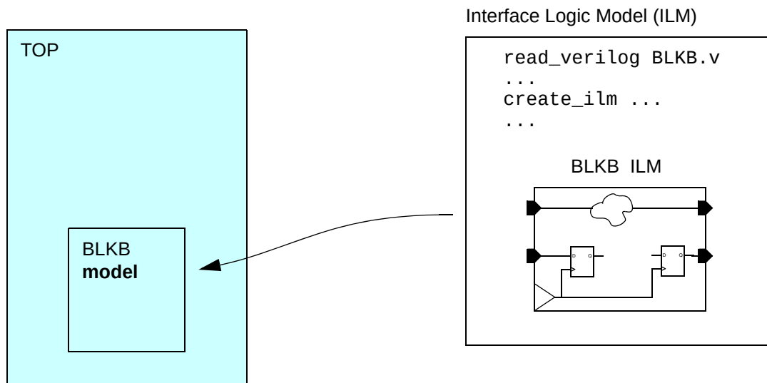
Figure A-1 Interface Logic Model Usage
