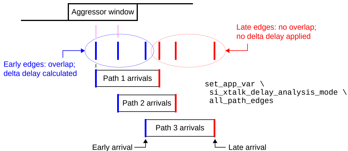
Figure 14-14 “All Path Edges” Overlap Mode
