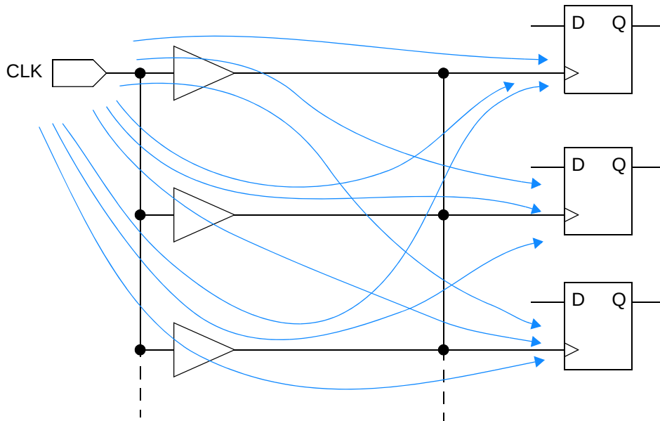
Figure 9-8 Parallel driver reduction
