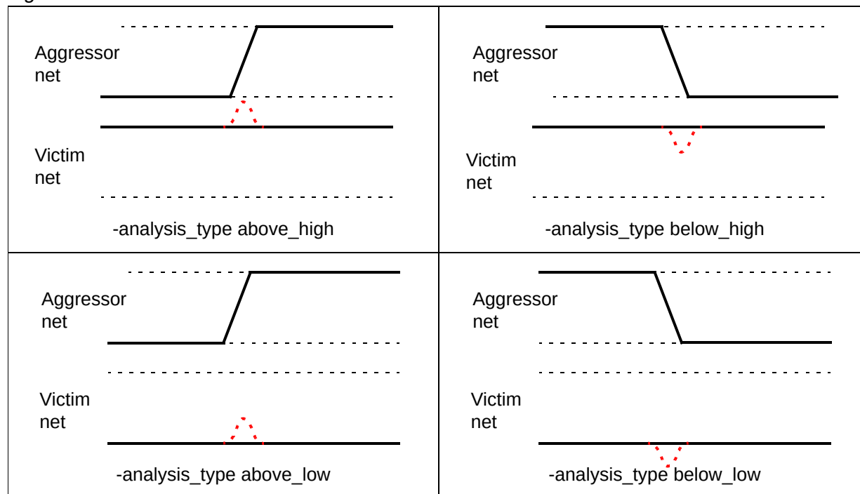
Figure 21-3 Crosstalk noise transitions for arcs
