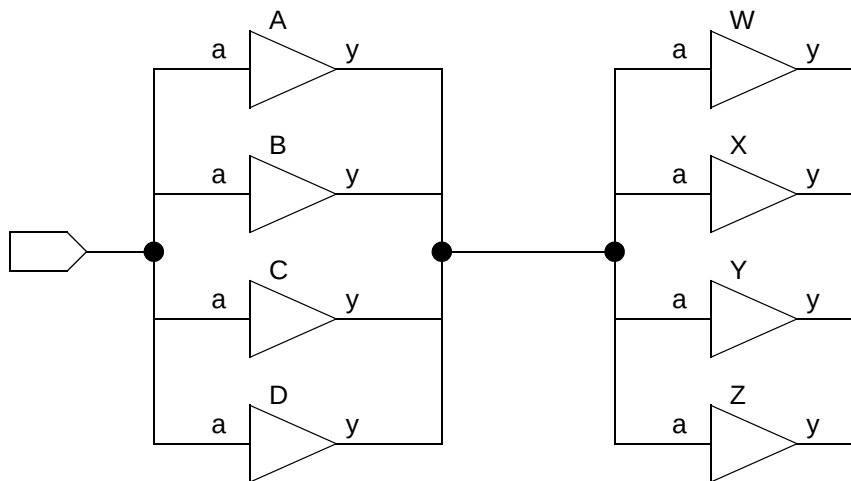
Figure 10-4 Parallel buffers driving parallel buffers
