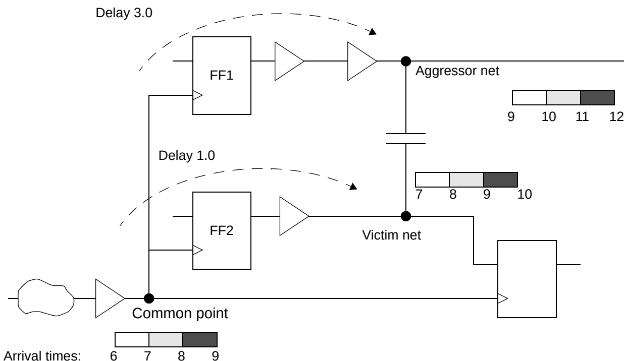
Figure 8-15 Clock reconvergence pessimism in crosstalk arrival windows
