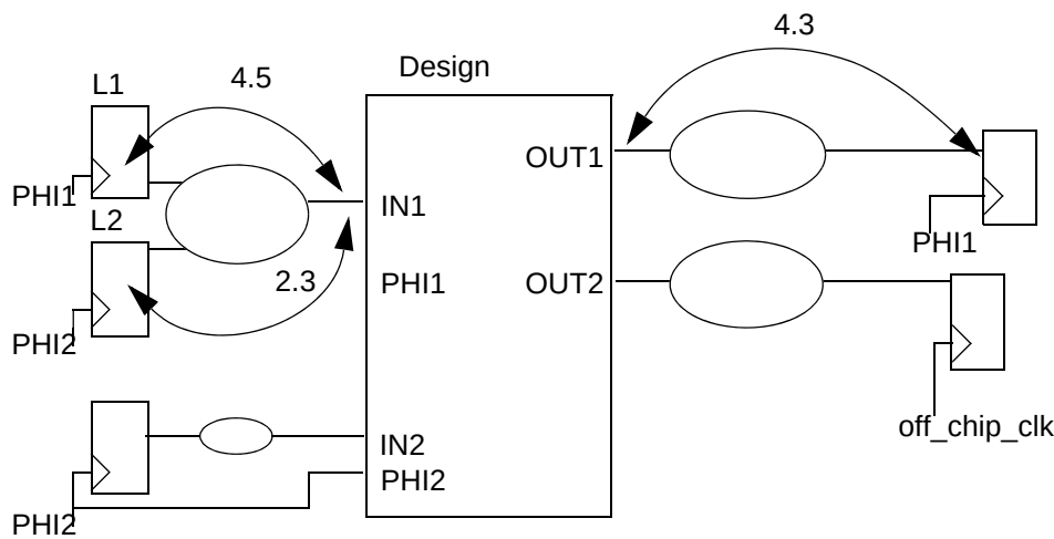
Figure 5-3 Two-phase clocking example for setting port delays
