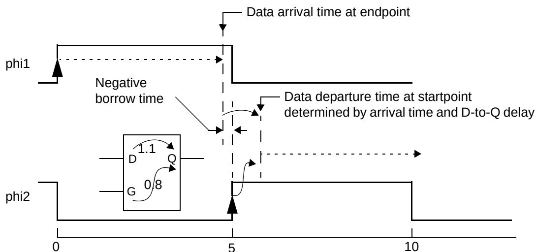
Figure 15-24 Negative borrow time
