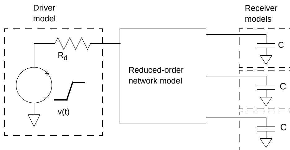
Figure 9-2 NLDM driver and receiver models
