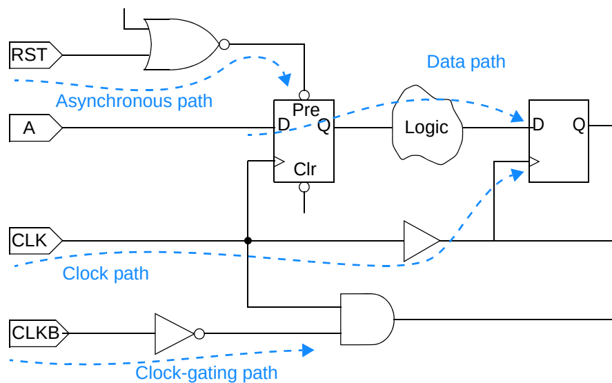
Figure 1-4 Types of paths considered for timing analysis
