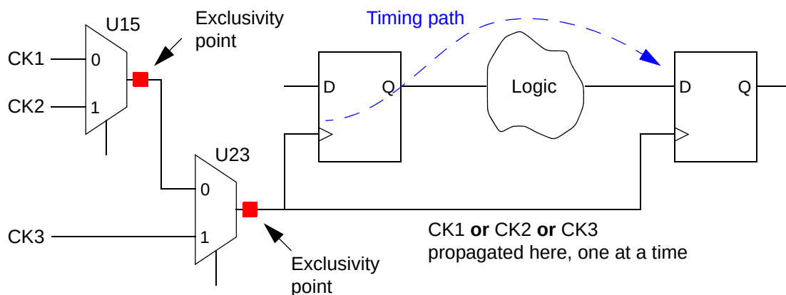
Figure 6-14 Multiplexed Clocks With Exclusivity Points
