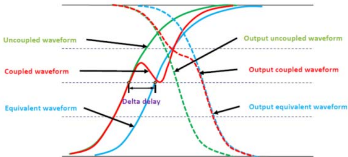
Figure 14-24 Signal integrity effect with CCS noise library or forward timing arc
