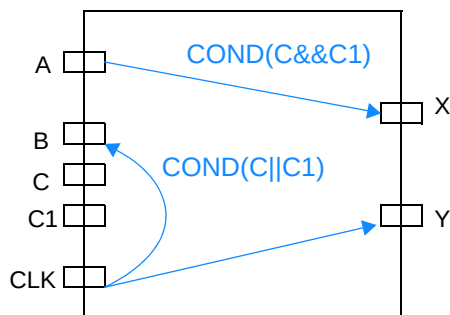
Figure 11-4 Conditional and nonconditional arcs in a Liberty Model
