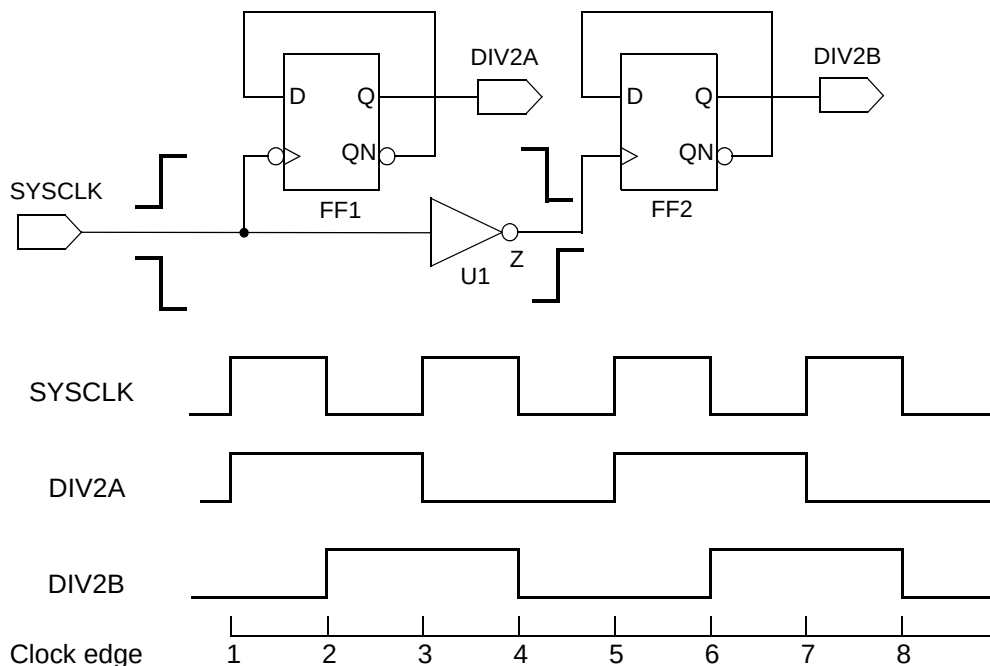
Figure 6-28 Generated divide-by-2 clocks based on different edges
