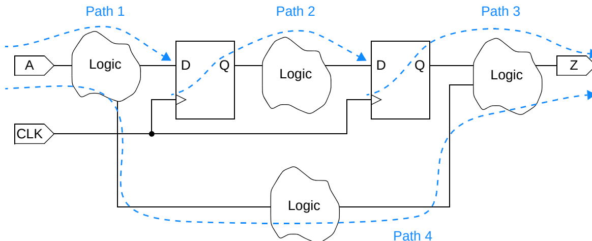
Figure 1-2 Timing paths
