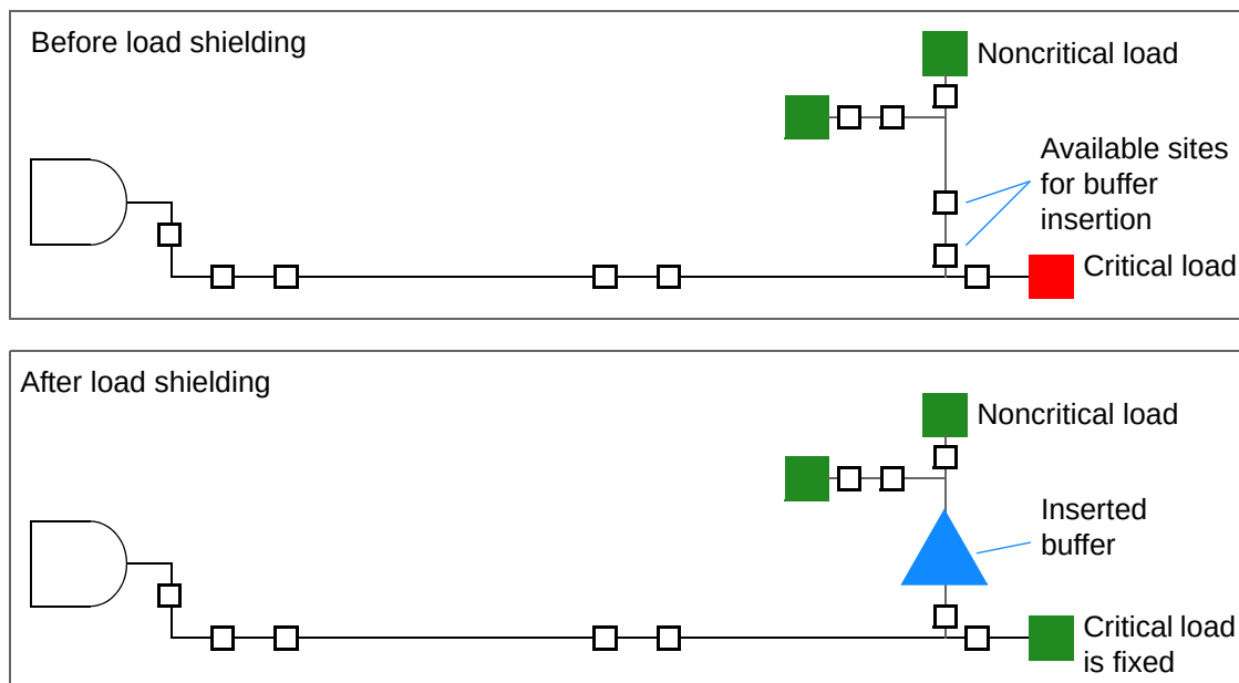
Figure 19-4 Load Shielding Example
