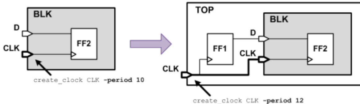
Figure 20-24 A Manually Fixable Block Boundary Violation
