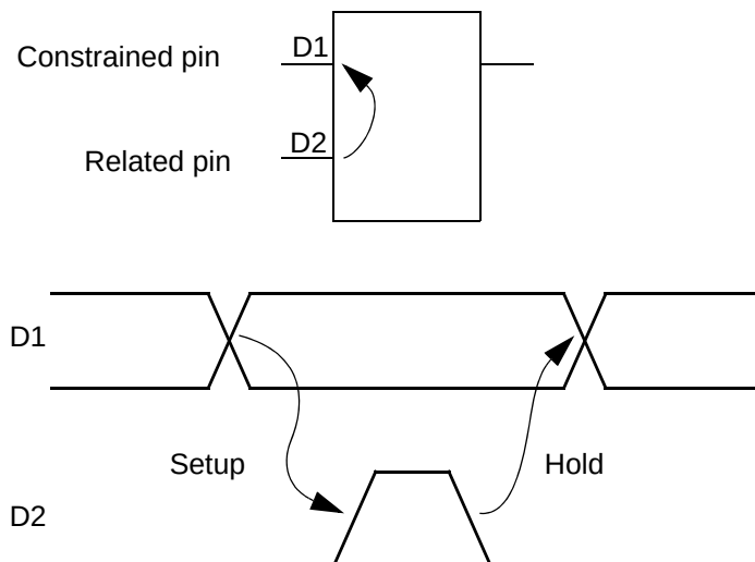
Figure 15-11 No-change data check
