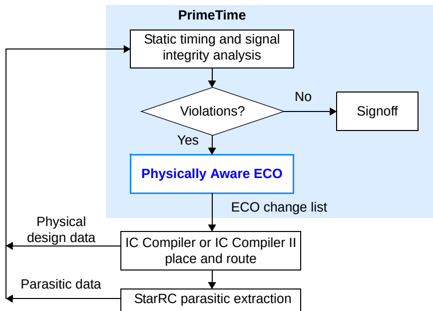
Figure 19-1 Synopsys Galaxy Physically Aware ECO Flow
