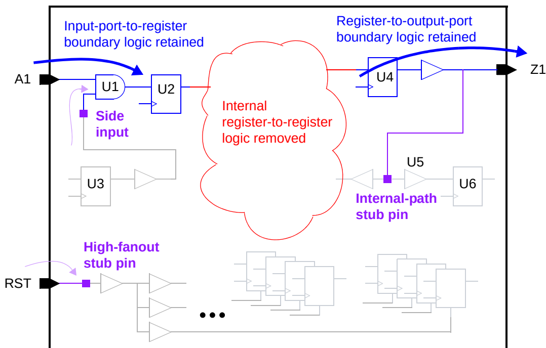
Figure 20-42 HyperScale Block Model
