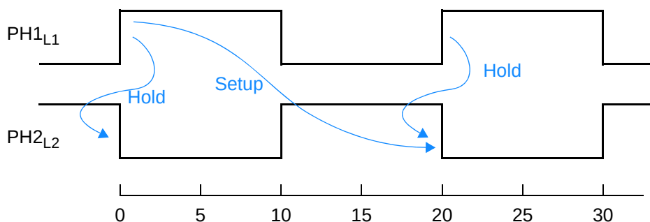
Figure 1-7 Hold checks in latch-based paths
