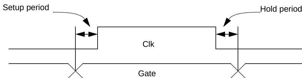
Figure 20-70 No-change arc
