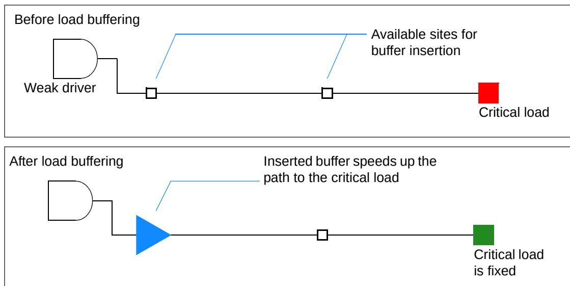
Figure 19-3 Load Buffering Example
