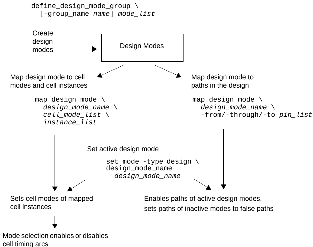
Figure 11-7 Defining, mapping, and setting design modes
