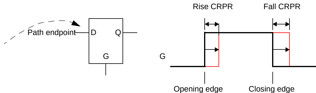
Figure 8-14 CRPR for latches
