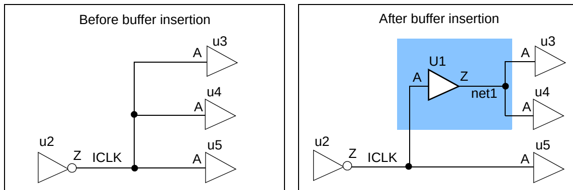
Figure 19-14 Buffer Insertion Example
