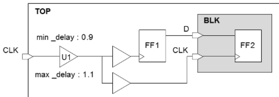
Figure 20-45 CRPR advanced boundary modeling
