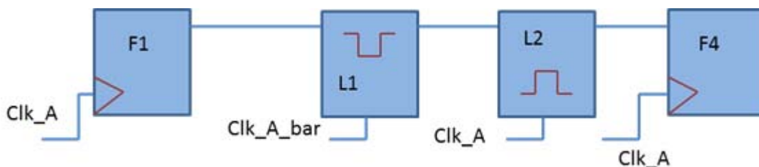
Figure 15-29 Incorrectly specified exceptions on throughpaths
