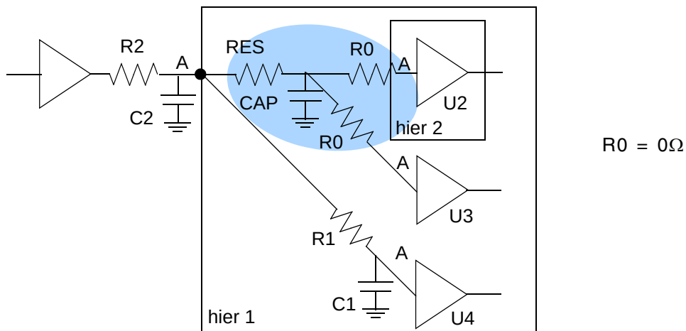
Figure 10-13 Missing segment completed using the fanout of two
