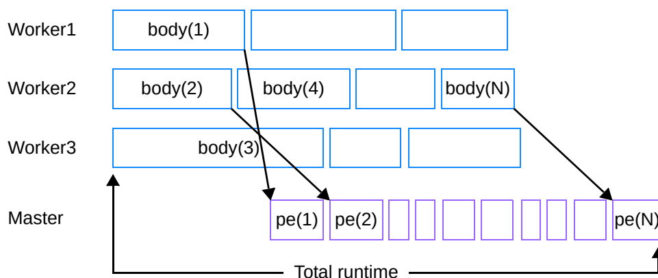
Figure 3-3 Execution of parallel_foreach_in_collection
