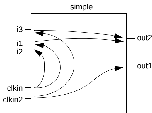
Figure 20-55 Extracted Library Cell Model
