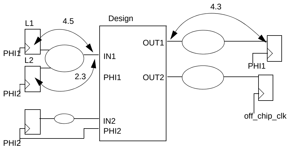
Figure 5-2 Two-phase clocking example for setting port delays
