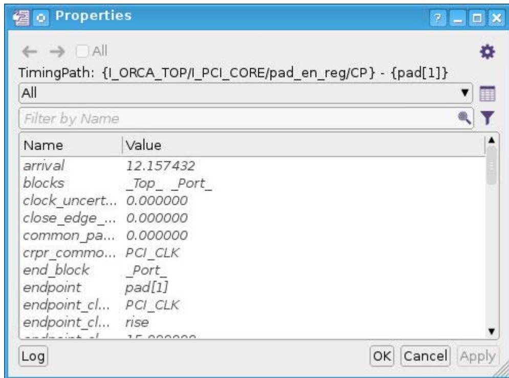
Figure 18-42 Properties Dialog Box
