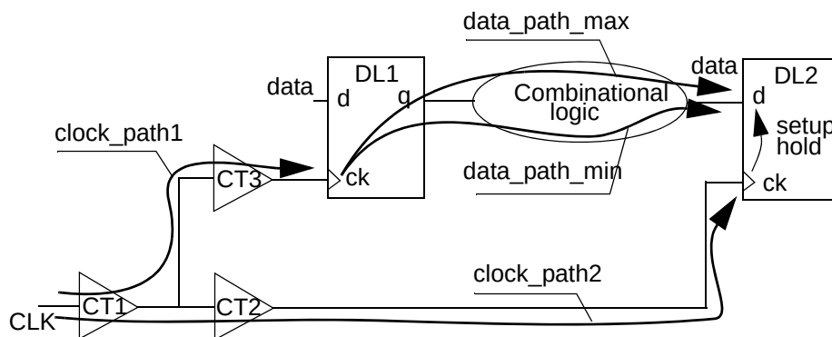
Figure 8-2 Design example
