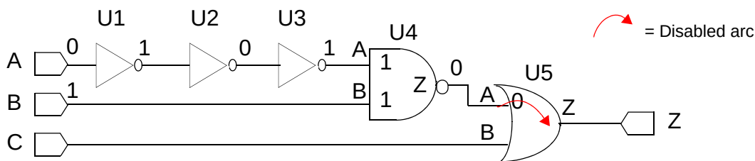
Figure 11-6 Arc from U5/A to U5/Z is disabled
