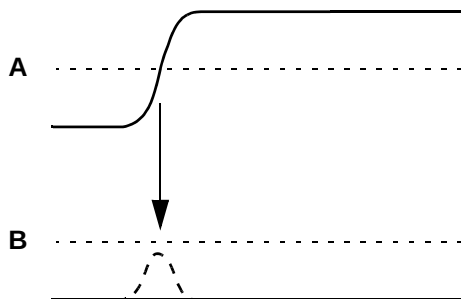
Figure 14-3 Noise bump due to crosstalk
