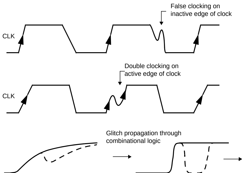
Figure 14-27 Undesirable effects of double-switching errors
