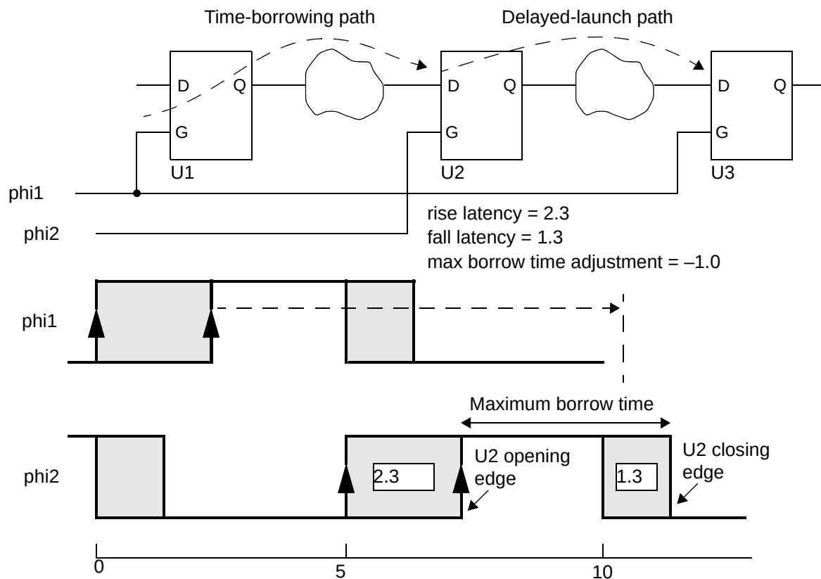
Figure 15-20 Maximum borrow time adjustment for latency
