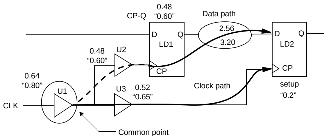
Figure 8-10 Clock reconvergence pessimism example
