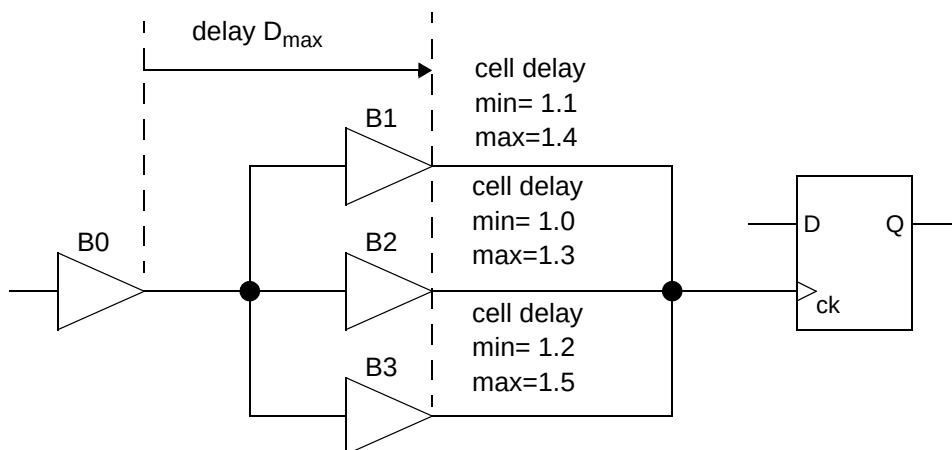
Figure 10-5 Cell delays in a parallel driver network
