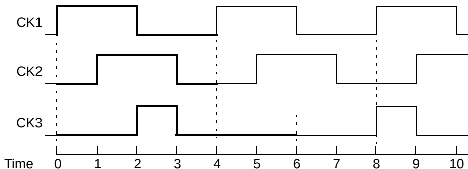
Figure 6-8 Synchronous clock waveforms
