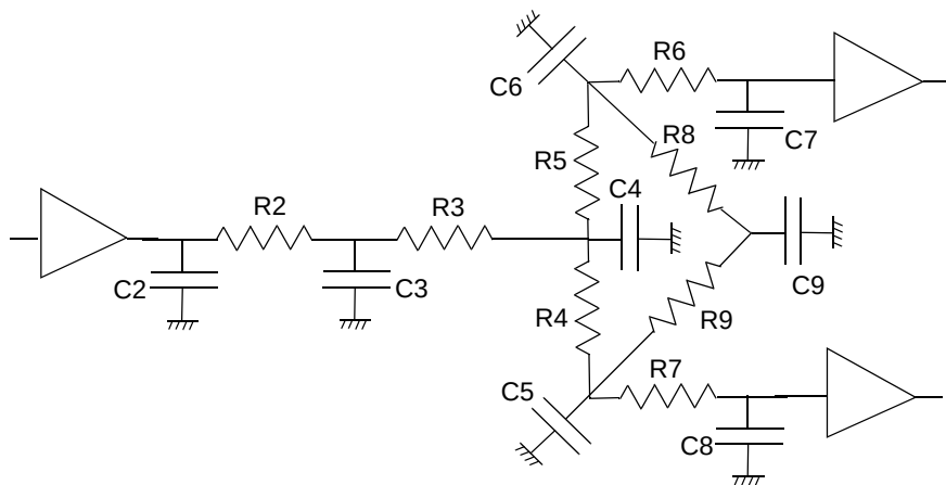
Figure 10-8 Meshed RC
