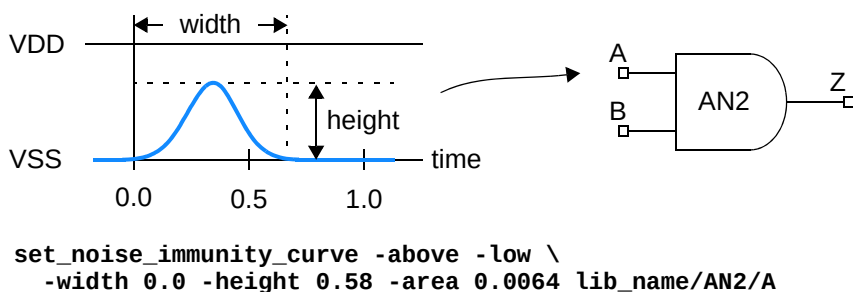
Figure 14-38 User-defined noise immunity curve
