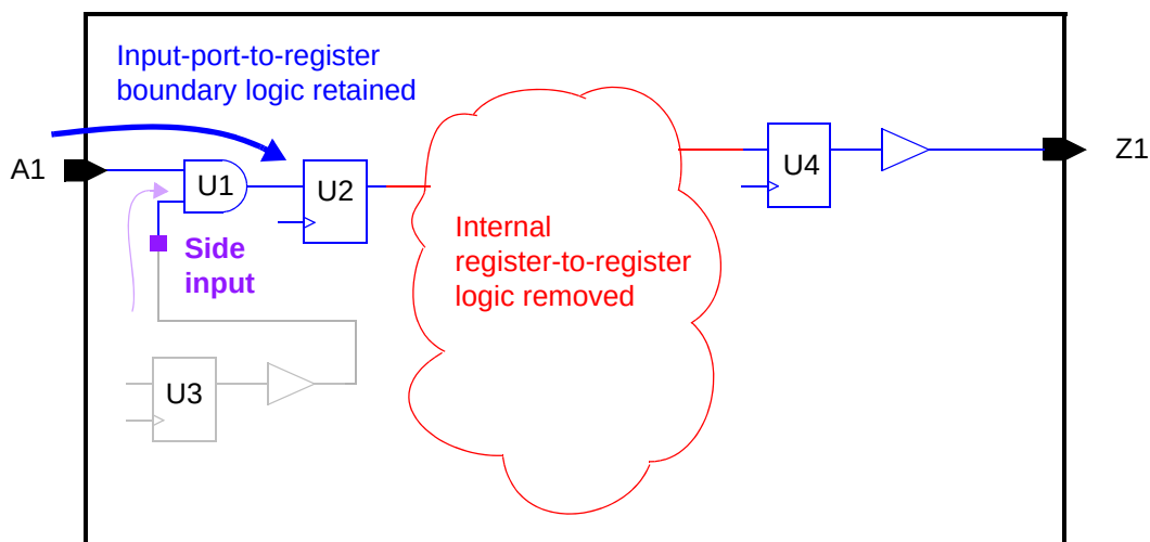
Figure 20-43 Side Input in Block Model
