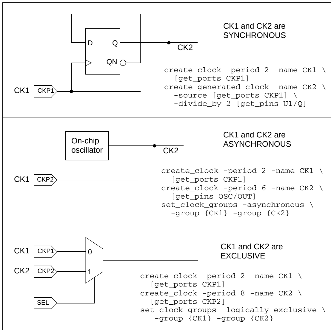
Figure 6-7 Synchronous, asynchronous, and exclusive clocks
