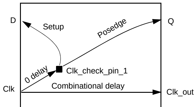
Figure 20-67 Model with check pin
