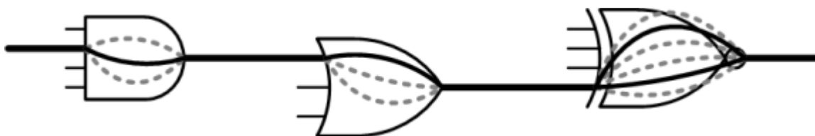
Figure 15-1 Worst arc used for path tracing
