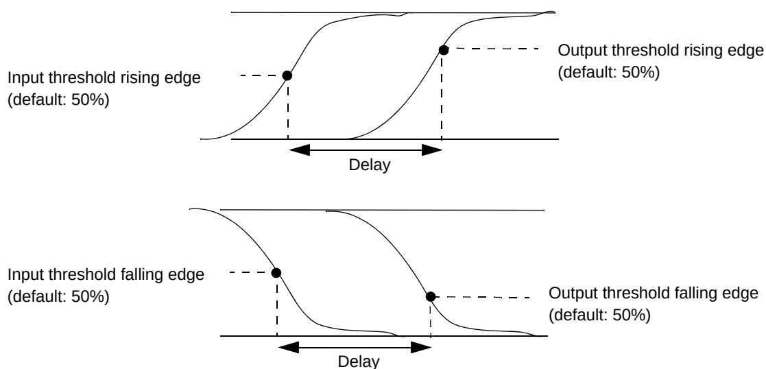
Figure 9-7 Input/output transition points
