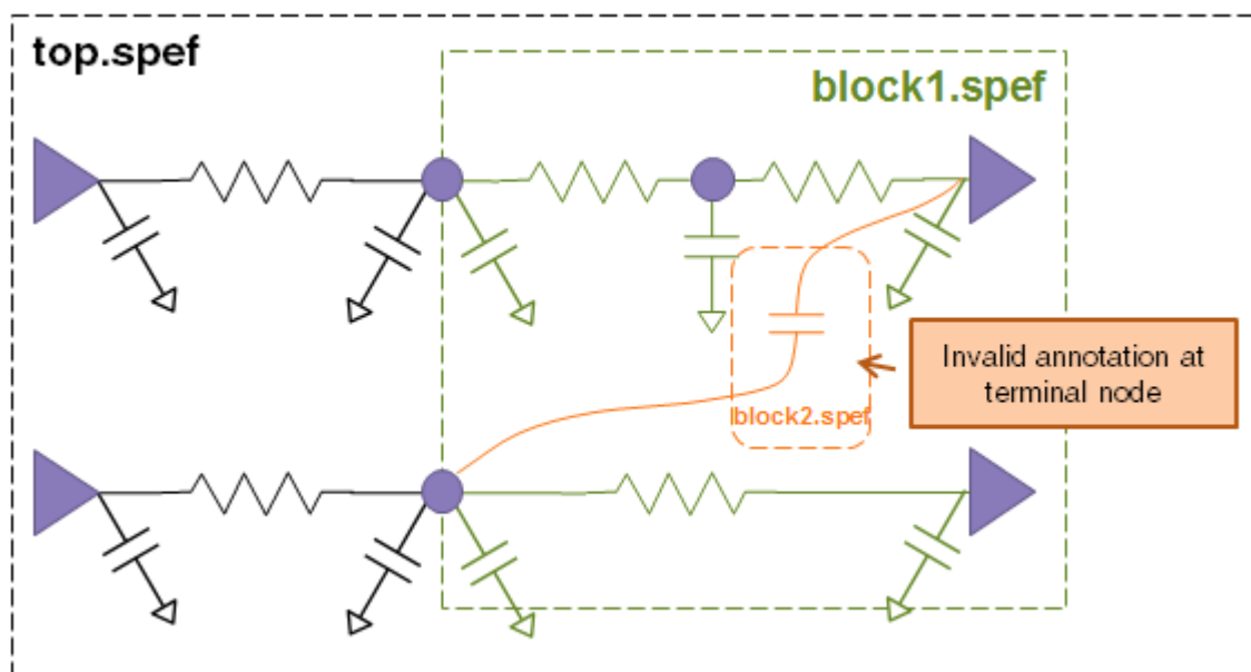
Figure 10-11 Second annotation is invalid
