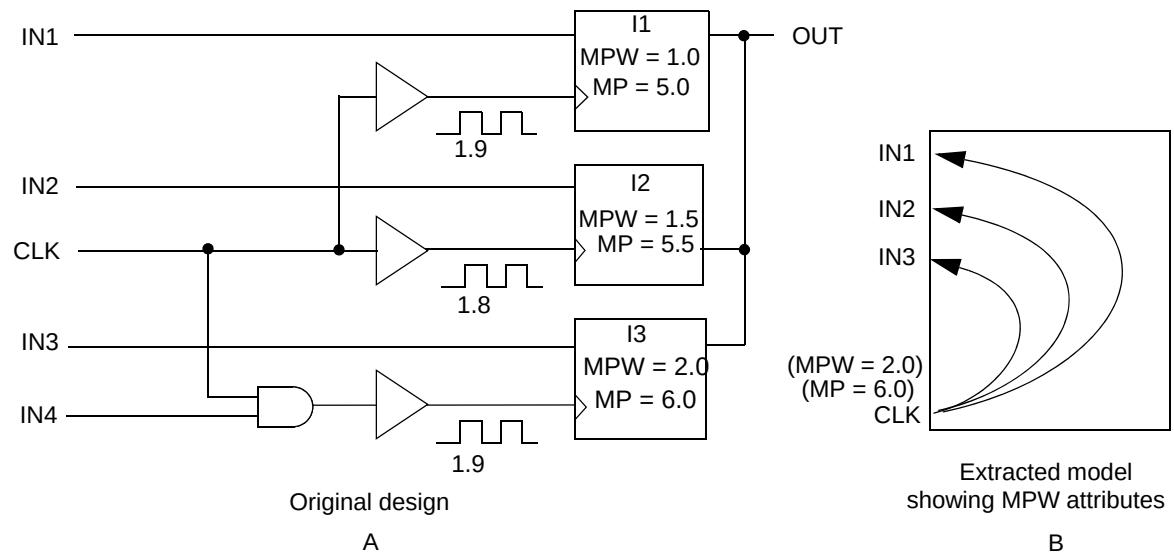
Figure 20-56 Minimum pulse width and minimum period extraction
