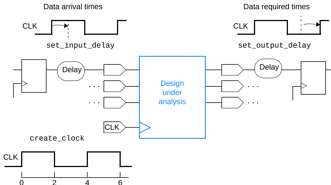
Figure 5-1 Design-level timing constraints
