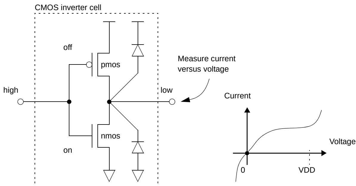
Figure 14-42 I-V characterization of a steady-state low output
