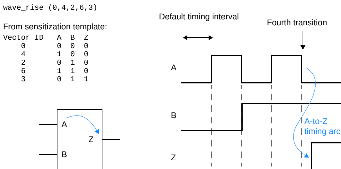
Figure 21-4 Usage of wave_rise in library sensitization definition
