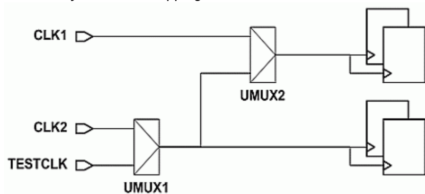
Figure 6-18 Physical clock stopping
