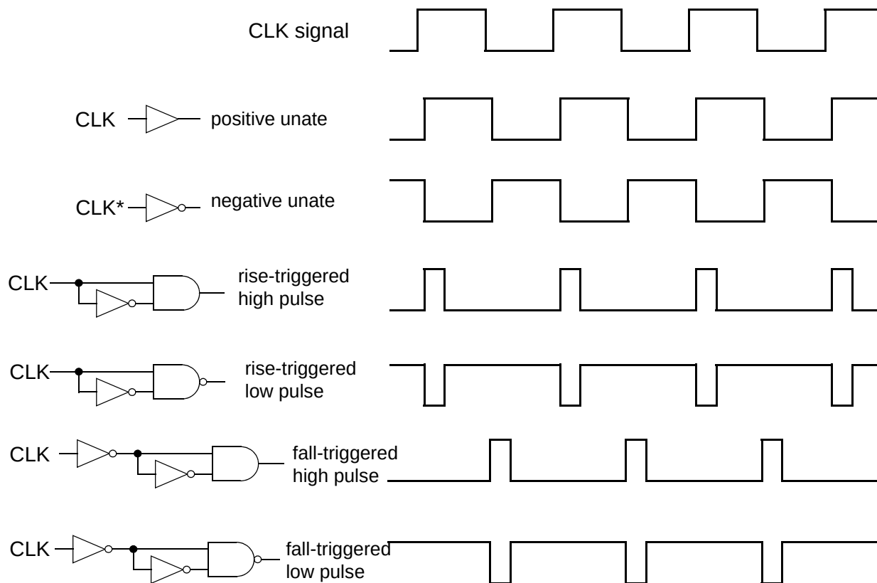
Figure 6-17 Clock sense examples
