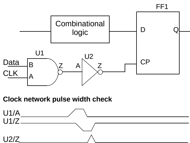
Figure 6-6 Clock network pulse width check
