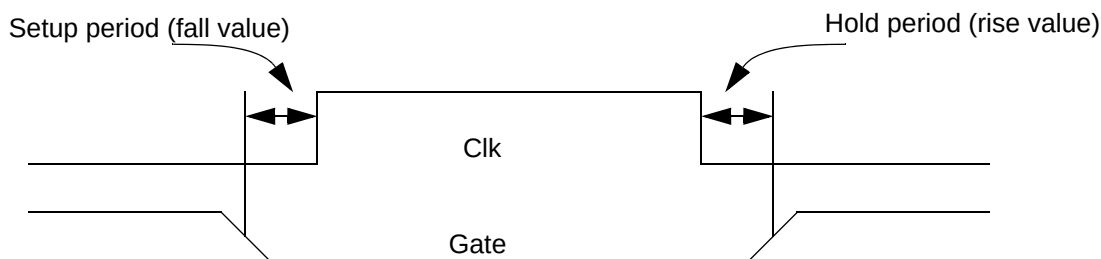
Figure 20-72 NOCHANGE_LOW_HIGH arc
