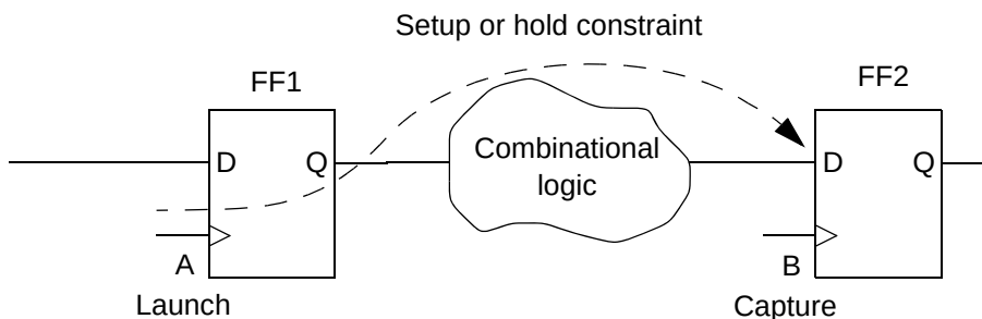
Figure 17-4 Clock skew calculation
