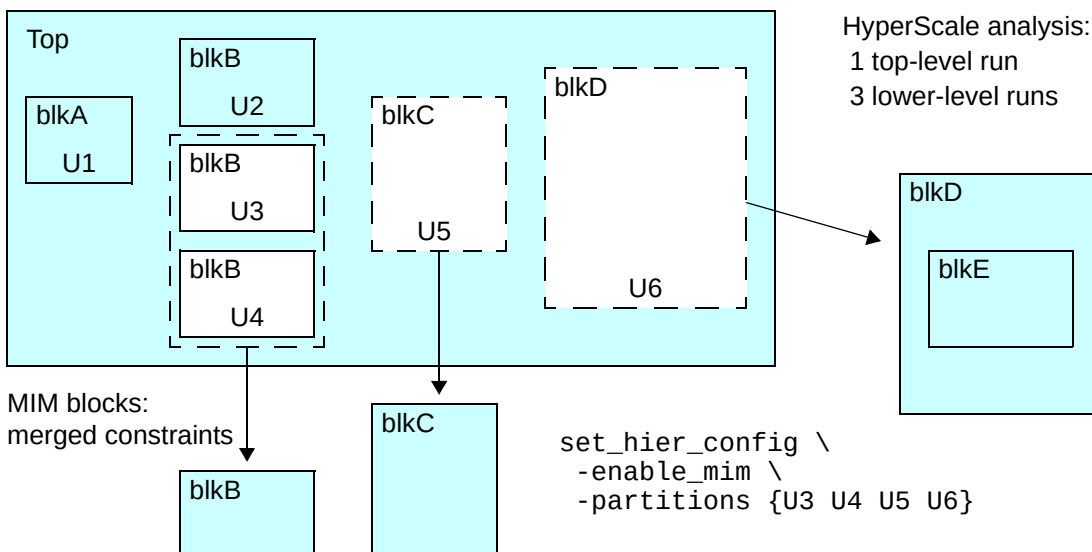
Figure 20-12 User-Directed Partitioning Example 3
