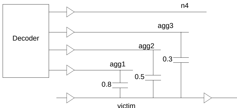
Figure 14-9 One-hot decoder multiple aggressor example
