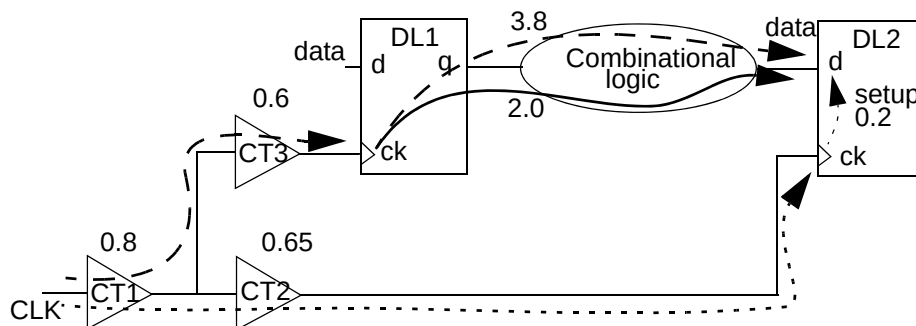
Figure 8-3 Setup check using worst-case conditions
