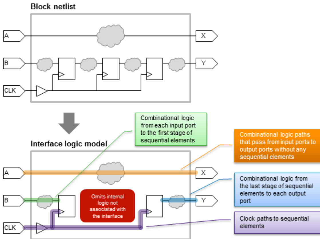
Figure A-2 Generated interface logic model from block netlist
