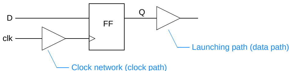
Figure 5-9 Restrict constraints
