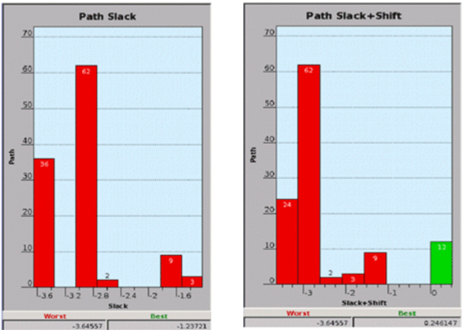
Figure 18-48 Path Slack and Path Slack+Shift
