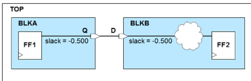
Figure 20-33 ECO fixing across multiple blocks
