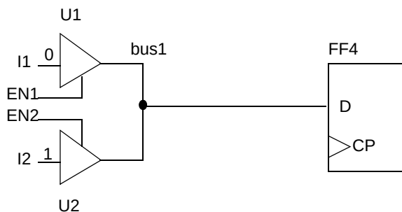
Figure 15-6 Circuit example
