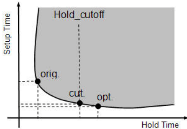
Figure 15-16 Setup slack improvement stops in cutoff hold slack
