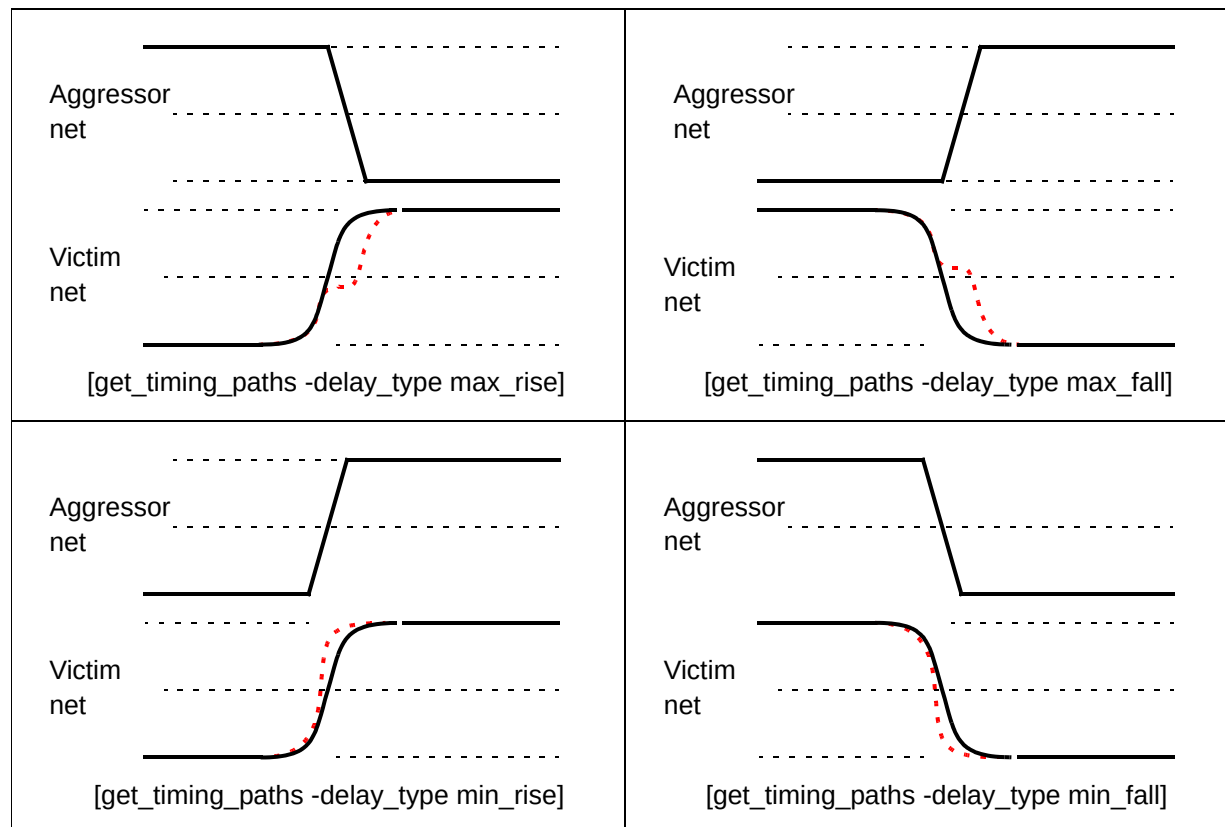
Figure 21-1 Specifying crosstalk delay transitions for paths
