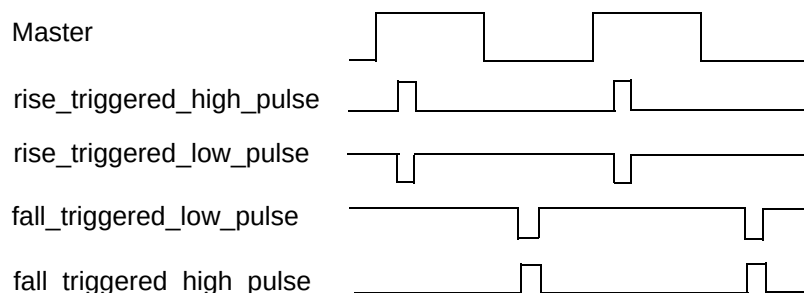
Figure 6-26 Pulse clock types that do not change frequency
