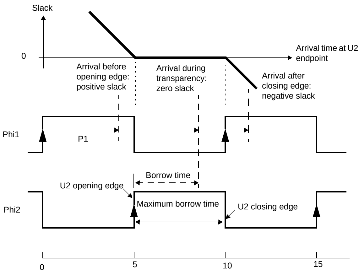
Figure 15-18 Latch-based timing path slack calculation
