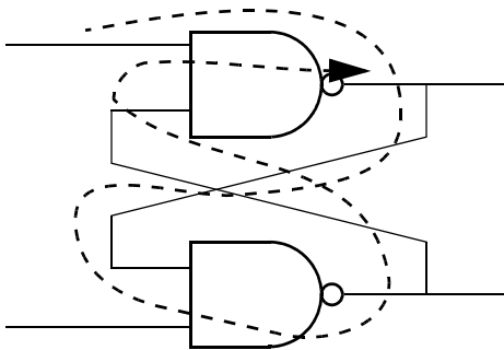
Figure 15-3 Combinational feedback loop
