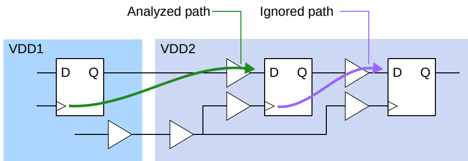
Figure 13-6 Analyzing only paths affected by domain crossings
