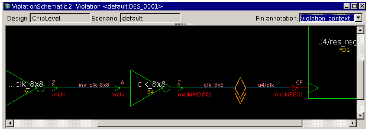
Figure 16-5 Schematic Viewer With Full Violation Context
