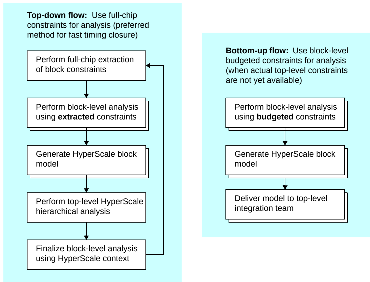
Figure 20-13 HyperScale Top-Down and Bottom-Up Hierarchical Analysis Flows
