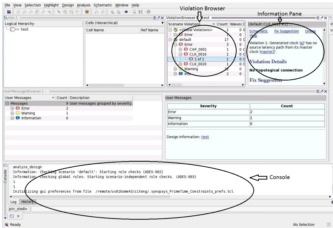
Figure 16-31 Constraint Consistency Window on Startup
