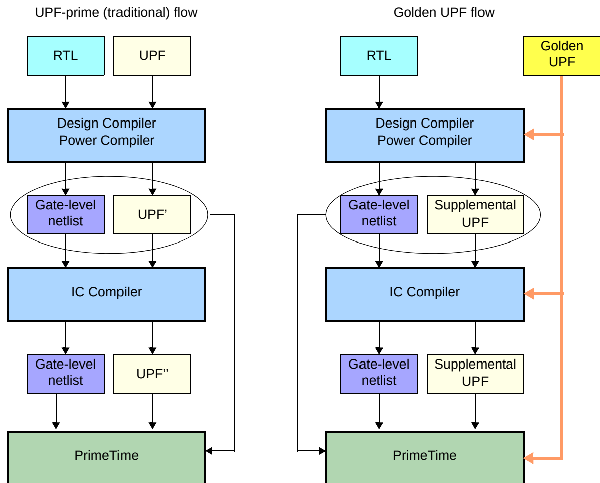
Figure 13-3 UPF-prime (traditional) and golden UPF flows
