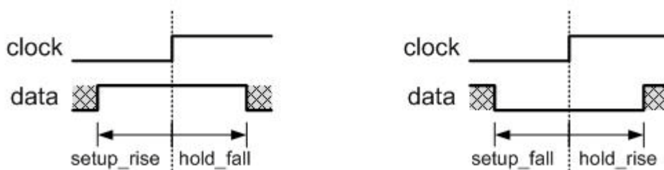
Figure 15-13 Two setup and hold tradeoff scenarios
