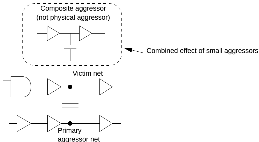
Figure 14-21 Composite aggressor mode enabled
