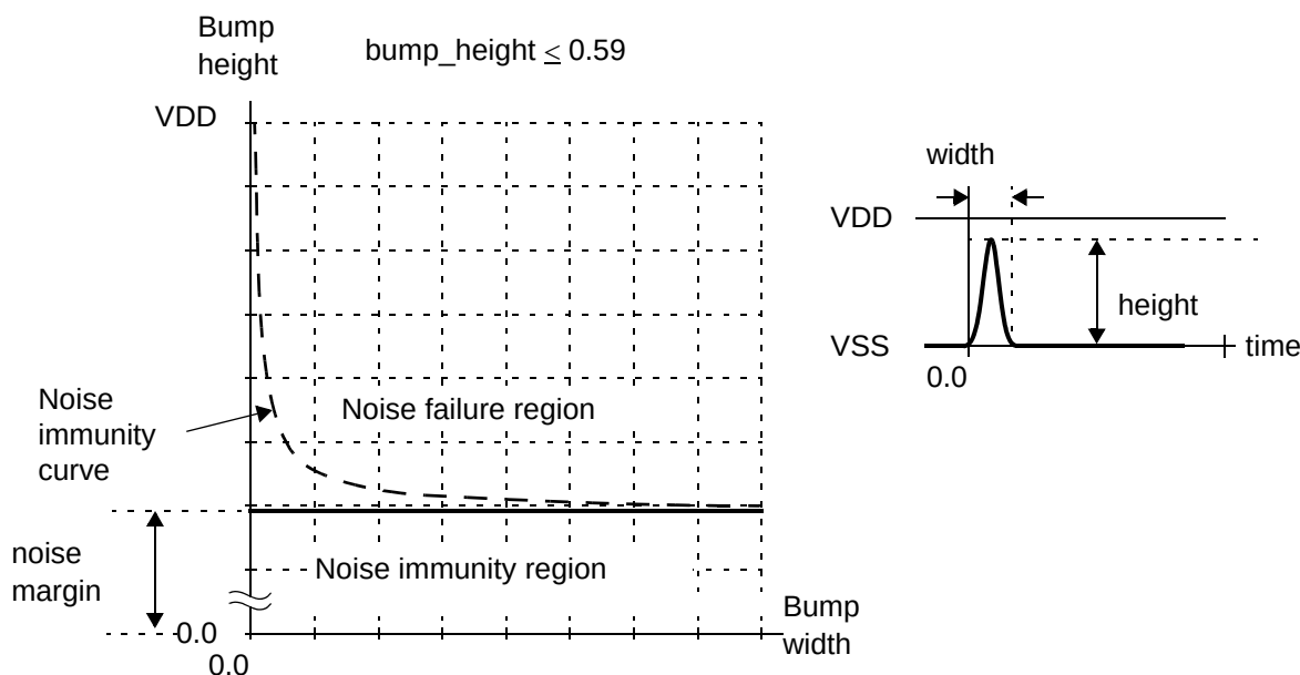
Figure 14-49 Height-only noise margin versus noise immunity curve
