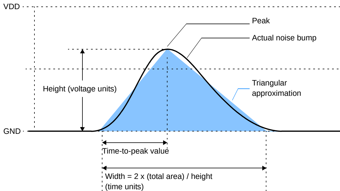
Figure 14-31 Noise bump characteristics
