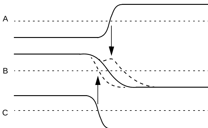
Figure 14-1 Transition slowdown or speedup caused by crosstalk
