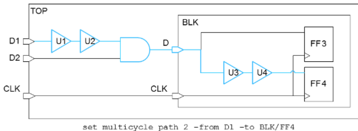
Figure 20-46 Path-specific exception modeling
