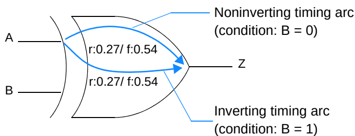
Figure 10-2 Annotated delays when the Synopsys library contains no conditions
