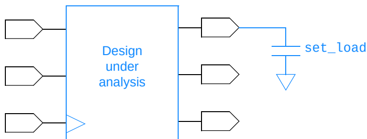
Figure 5-5 Output load
