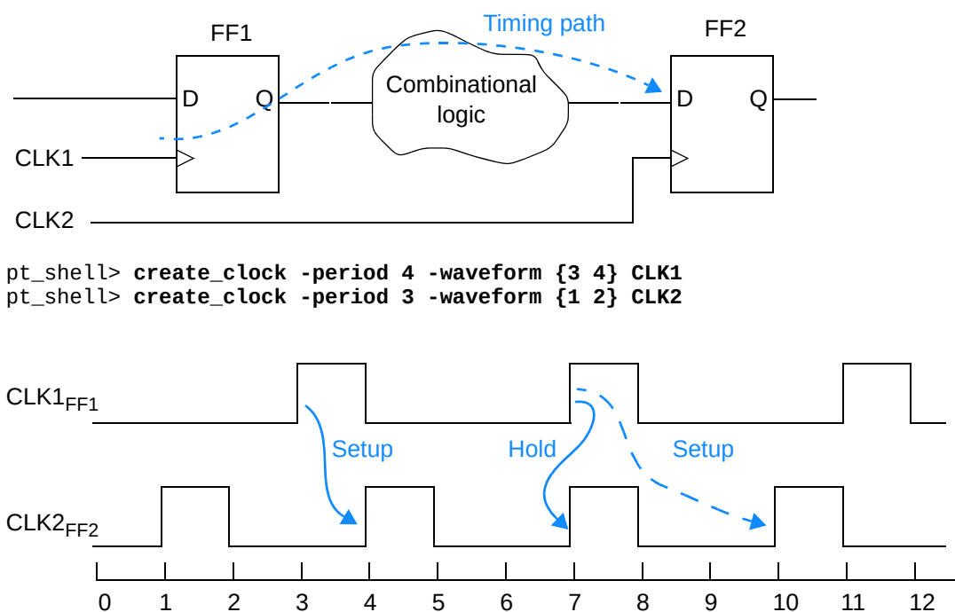
Figure 7-11 Delay requirements with 4ns/3ns clocks
