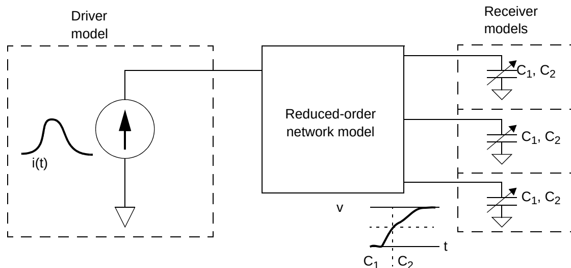
Figure 9-3 CCS timing driver and receiver models
