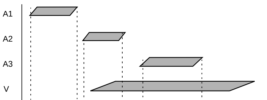
Figure 14-12 Multiple aggressor alignment
