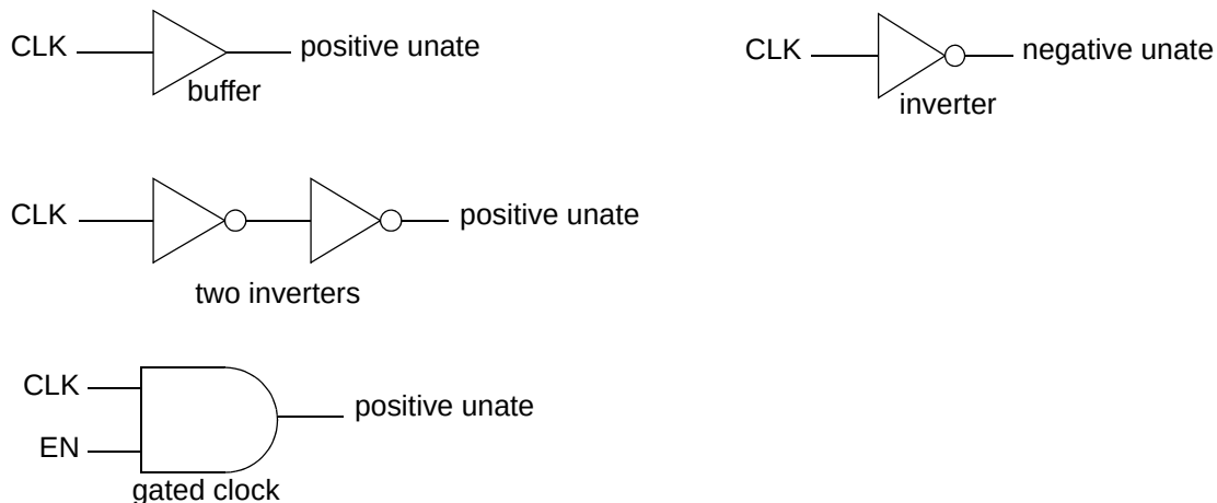
Figure 6-15 Positive and negative unate clock signals
