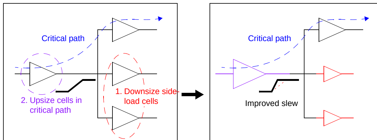
Figure 19-5 Side-Load Cell Sizing Example
