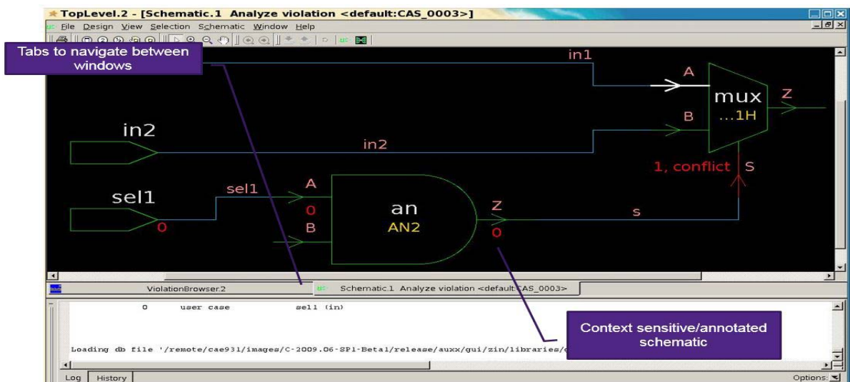
Figure 16-4 Schematic Viewer Shows Violation Circuit Path
