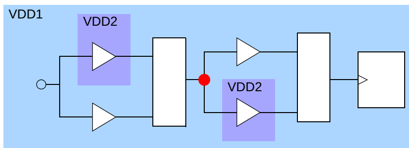
Figure 13-7 Clock path reconverges
