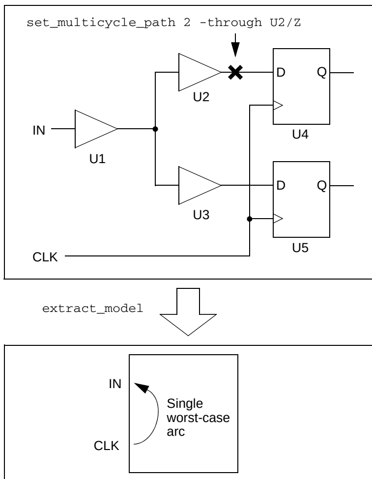
Figure 20-65 Multicycle path extraction without an output_mcp.pt file
