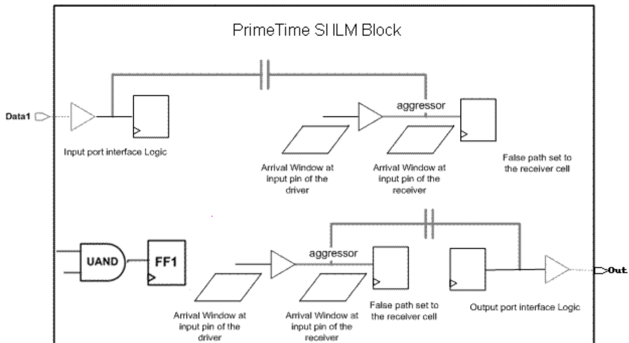
Figure A-3 PrimeTime SI ILM block
