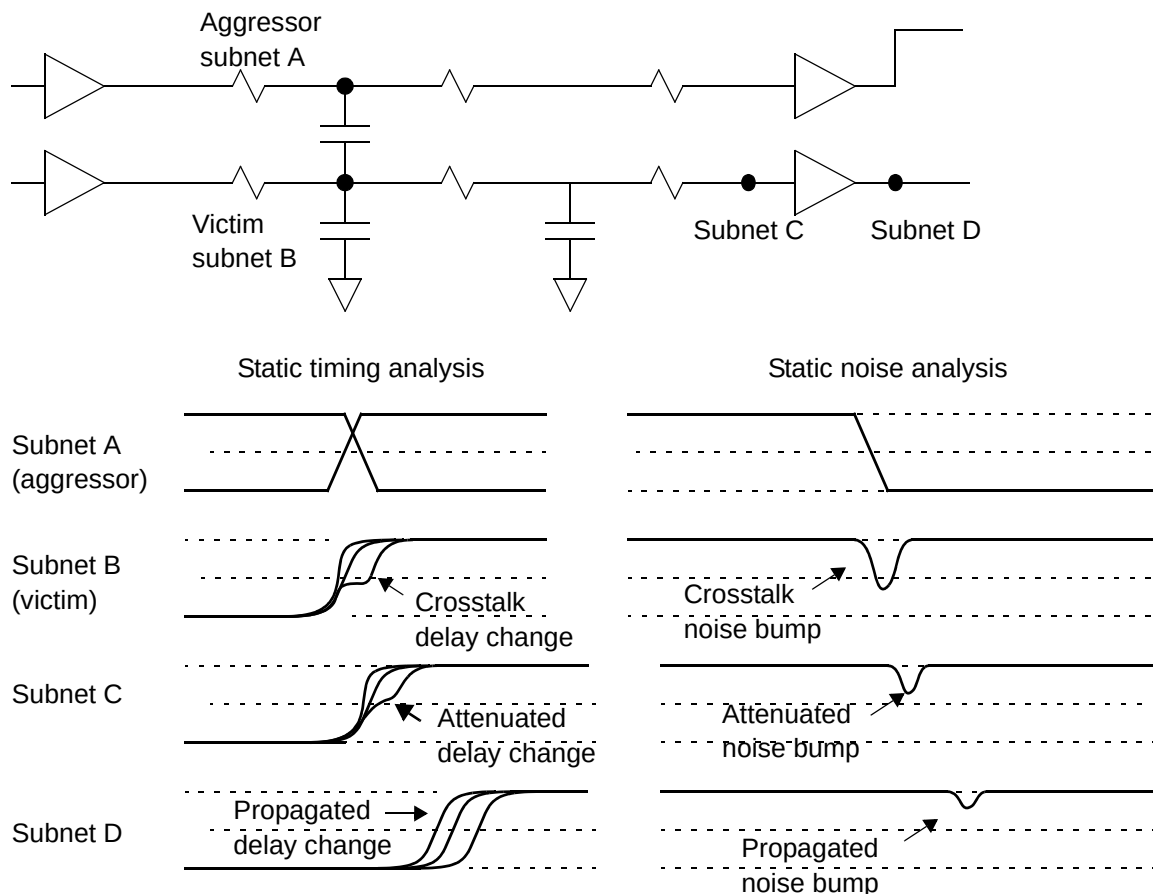
Figure 14-28 Crosstalk effects on timing and steady-state voltage
