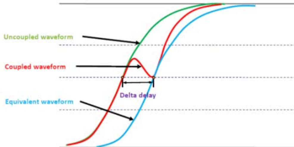
Figure 14-25 Signal integrity effect without CCS noise library and forward timing arc
