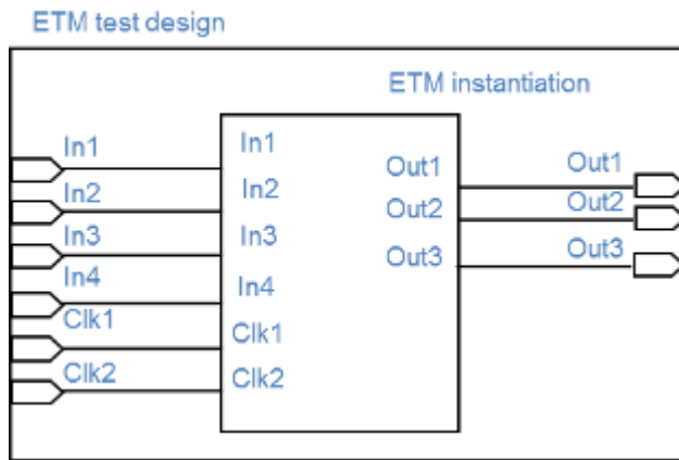
Figure 20-74 Test design with ETM instance
