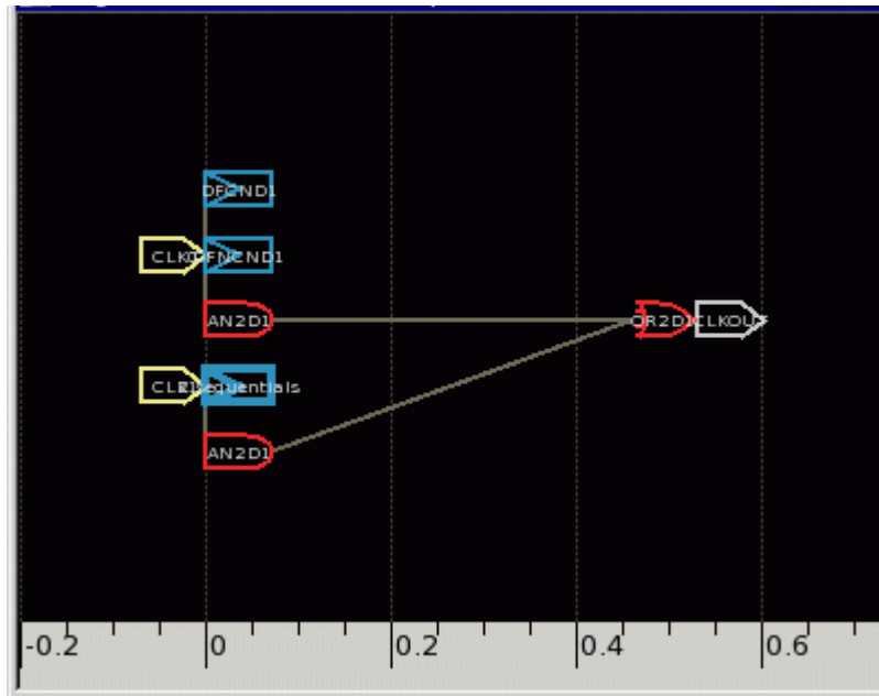
Figure 18-18 Clock Latency Layout in an Abstract Clock Graph View
