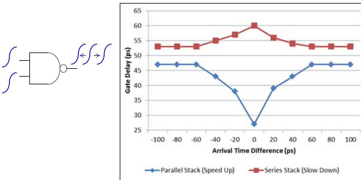
Figure 9-9 Multi-input switching affects the output delay and transition time
