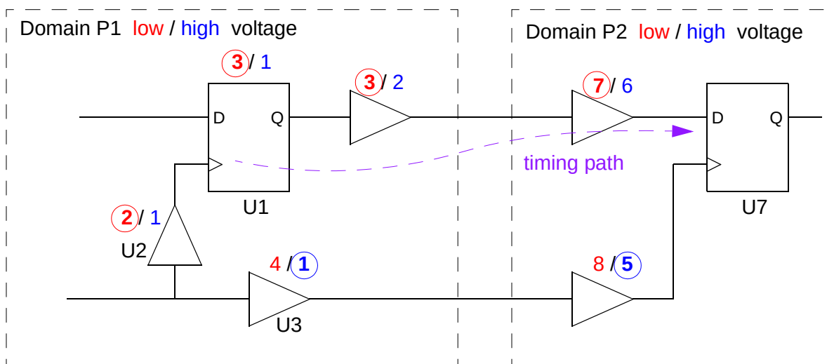
Figure 13-4 Timing path through two power domains
