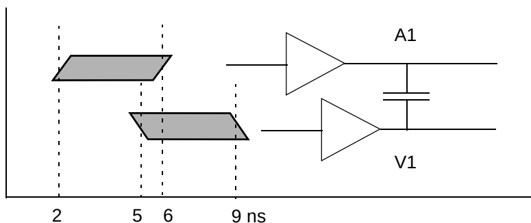
Figure 14-11 Victim-aggressor switching time alignment
