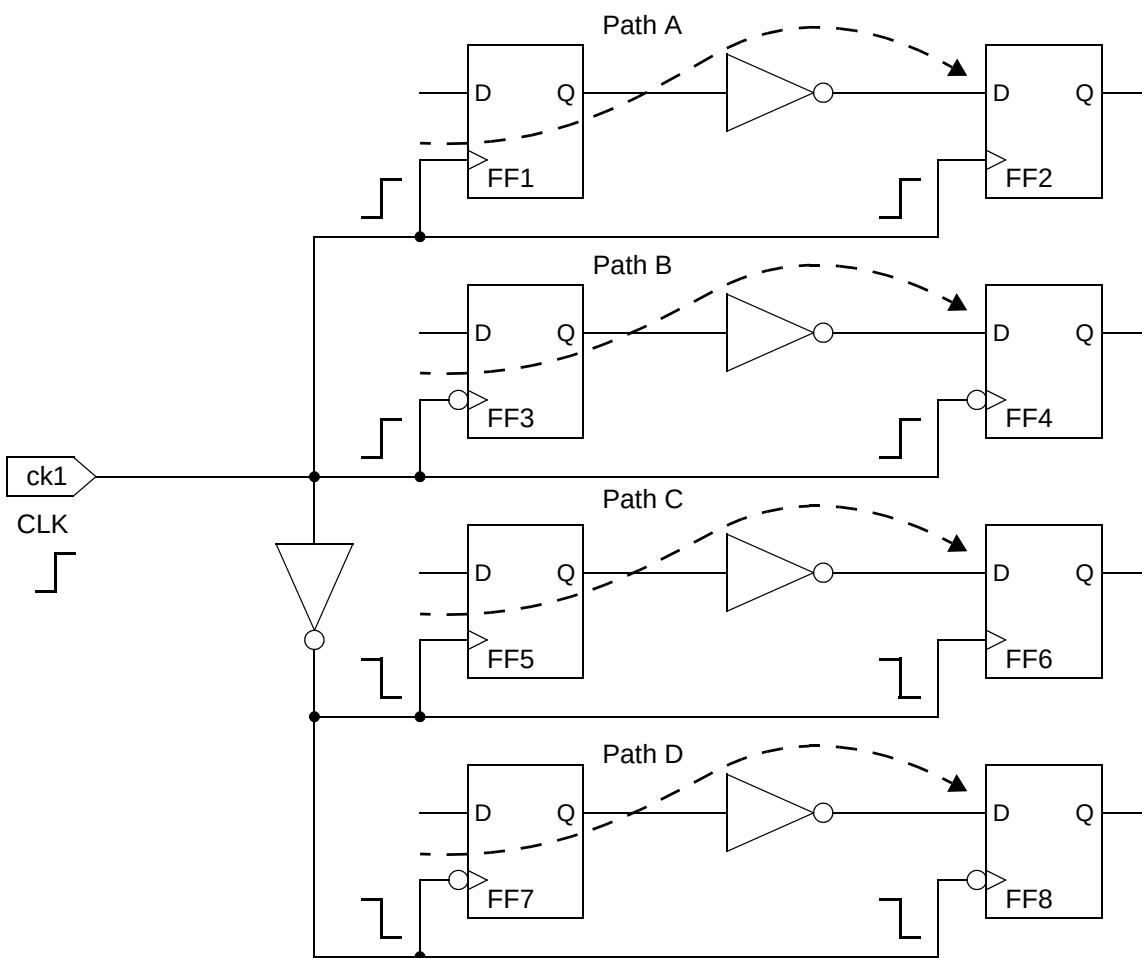
Figure 7-1 Circuit for path specification in examples 1 to 3
