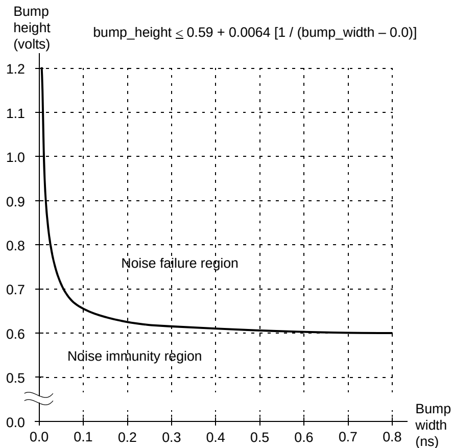
Figure 14-39 Plot of user-defined noise immunity curve
