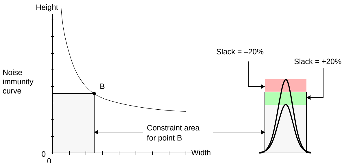
Figure 14-51 Area percent slack calculation
