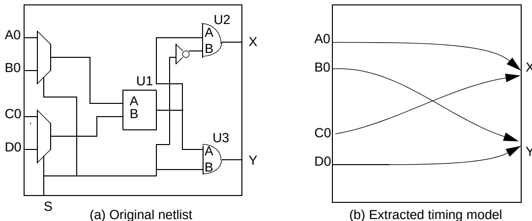
Figure 20-63 Original design with false paths and extracted model
