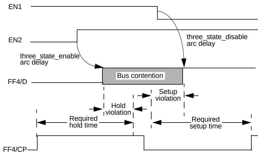
Figure 15-7 Transient bus contention check
