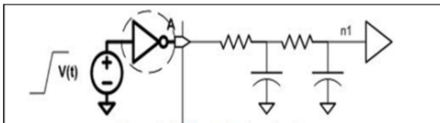
Figure 20-73 Driving cell set at the input port
