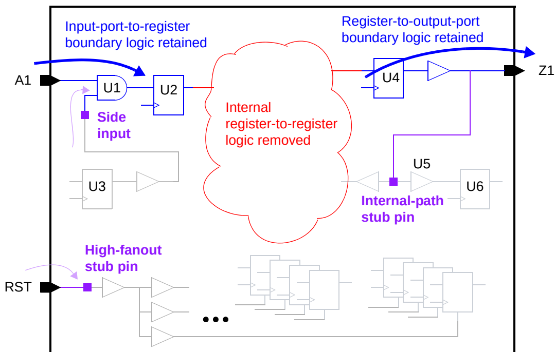
Figure 20-4 HyperScale Block Model
