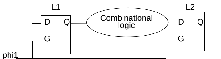
Figure 5-12 Latch fanout to another latch of the same clock
