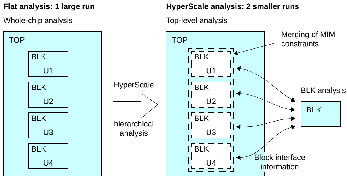
Figure 20-6 Context Merging for Multiply Instantiated Modules
