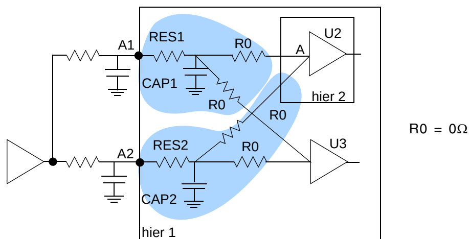
Figure 10-14 Multidrive segments
