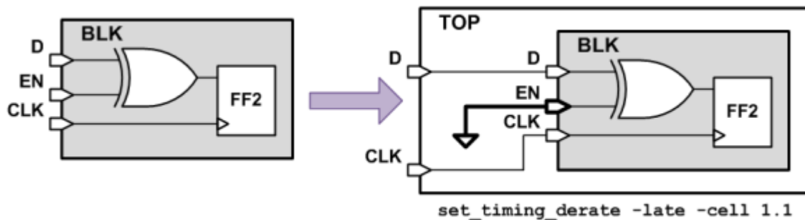
Figure 20-23 A fixable block boundary violation
