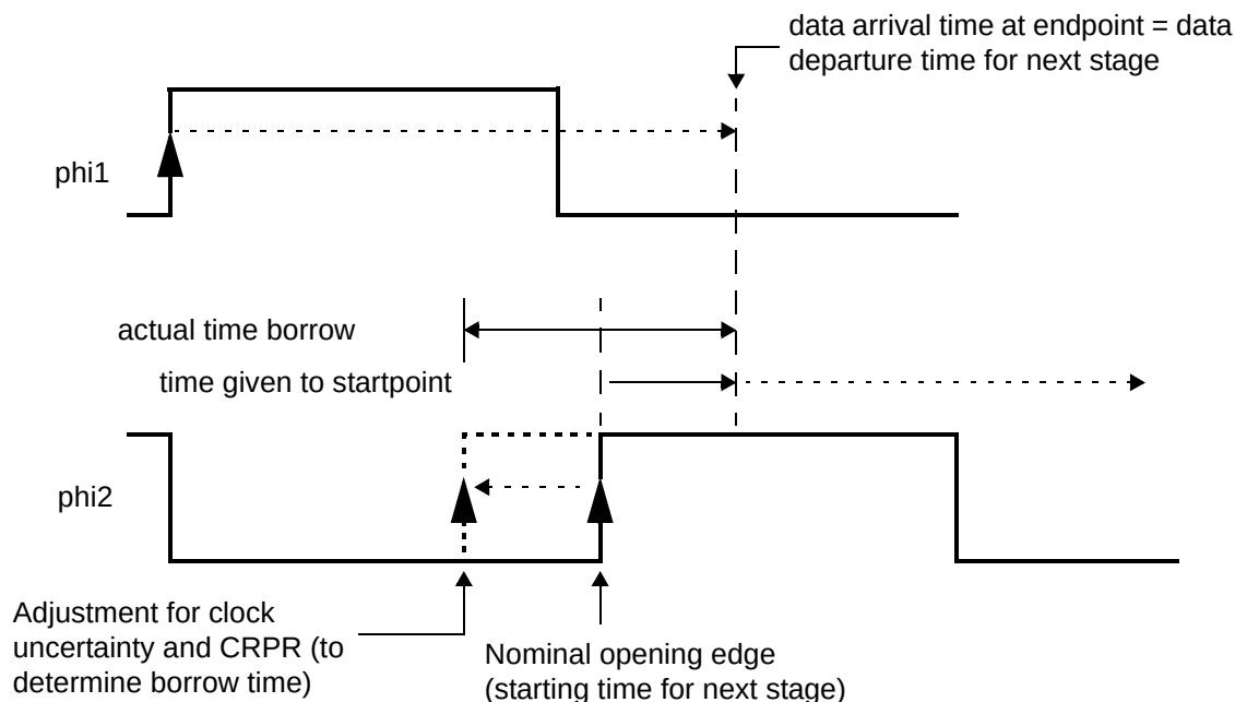
Figure 15-23 Borrow time and time given to startpoint in transparent mode
