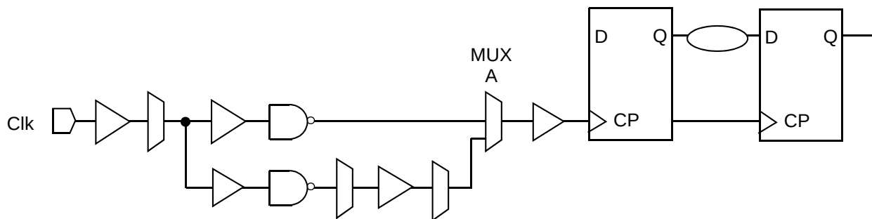
Figure 8-11 Reconvergent logic in a clock network
