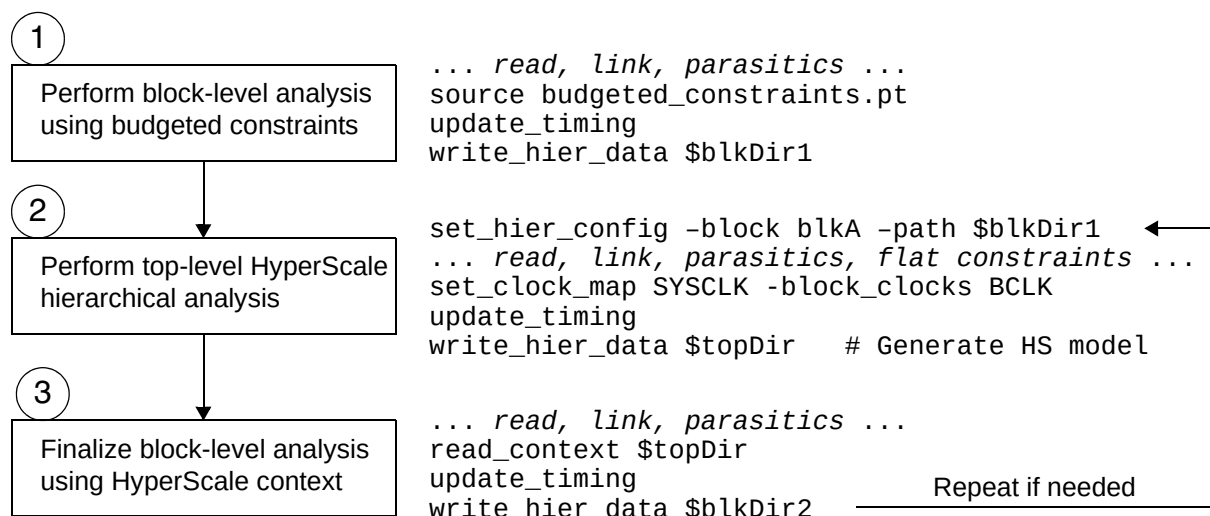
Figure 20-15 HyperScale Bottom-Up Hierarchical Analysis Flow
