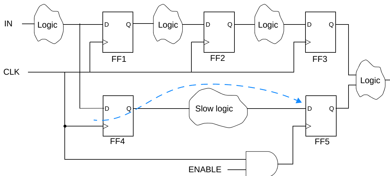
Figure 7-12 Multicycle path example
