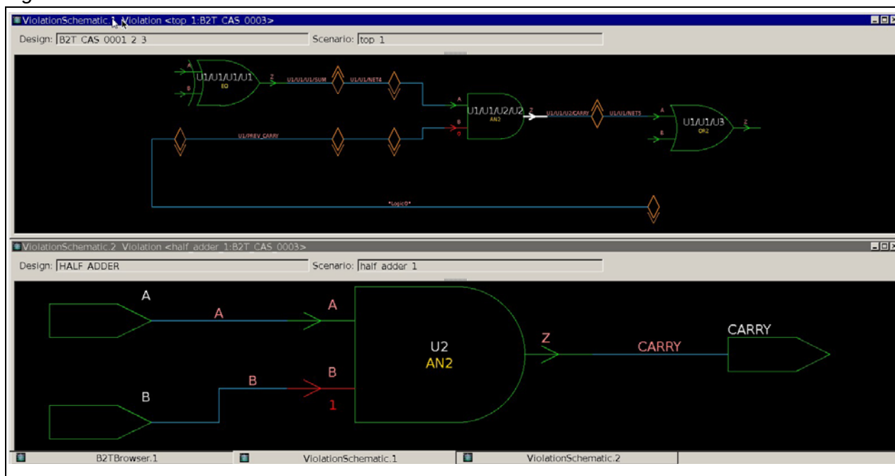
Figure 16-20 Dual Schematic
