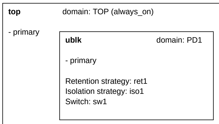
Figure 13-1 Design example using supply set handles
