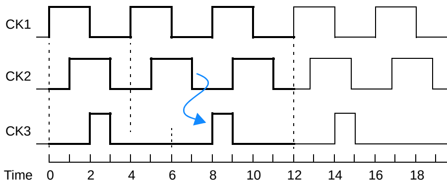
Figure 6-9 Expanded clock waveforms
