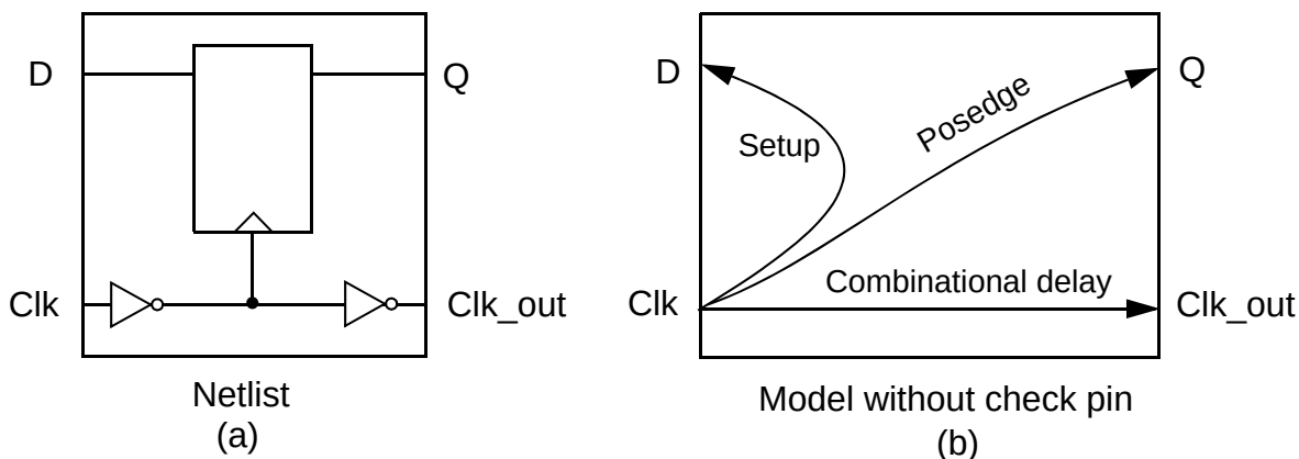
Figure 20-66 Original circuit and extracted model without check pins
