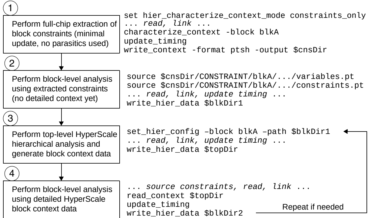
Figure 20-14 HyperScale Top-Down Hierarchical Analysis Flow
