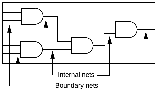
Figure 20-57 Boundary nets and internal nets
