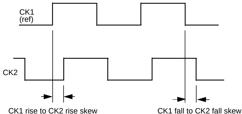
Figure 17-3 Timing diagram for skew constraint
