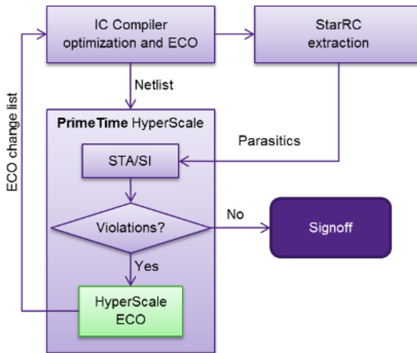
Figure 20-40 Flow links from HyperScale ECO to IC Compiler and StarRC
