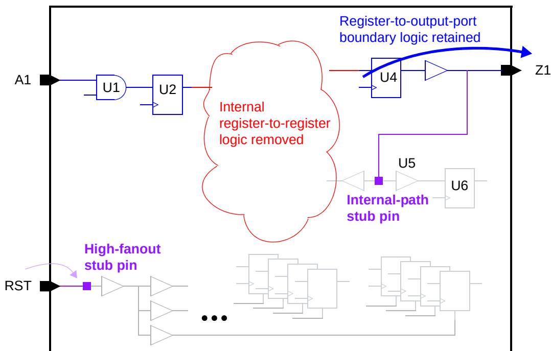
Figure 20-44 HyperScale Block Model
