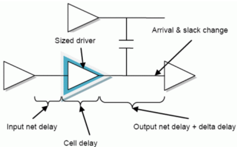
Figure 19-13 Parameters Considered by ECO Timing Estimation
