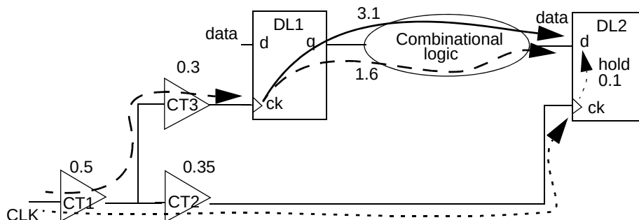
Figure 8-4 Hold check using best-case conditions
