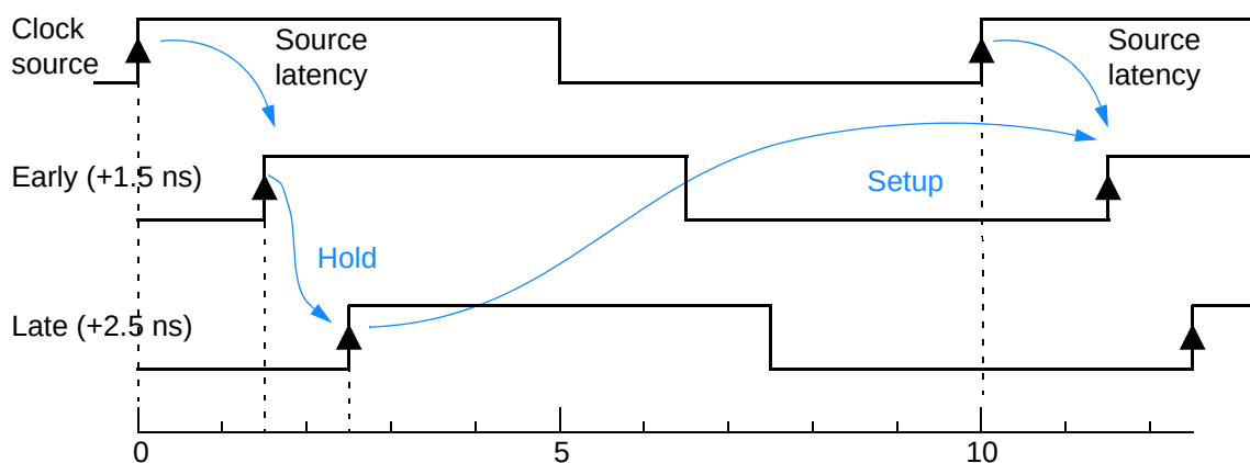
Figure 6-4 Early and late source latency waveforms
