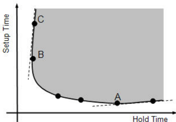
Figure 15-14 Interdependent setup and hold value curve
