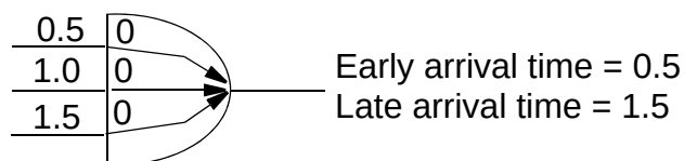
Figure 8-9 Early and late arrival time
