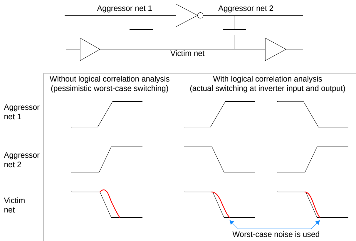
Figure 14-7 Logical correlation
