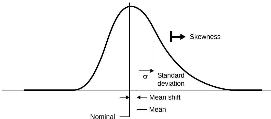
Figure 12-2 Moment-Based Asymmetric Delay Distribution
