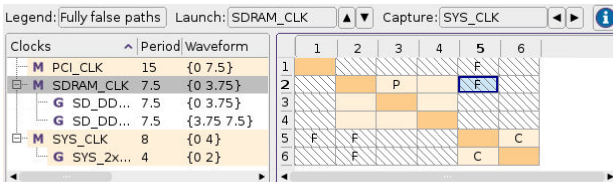
Figure 18-22 Clock Analyzer Matrix
