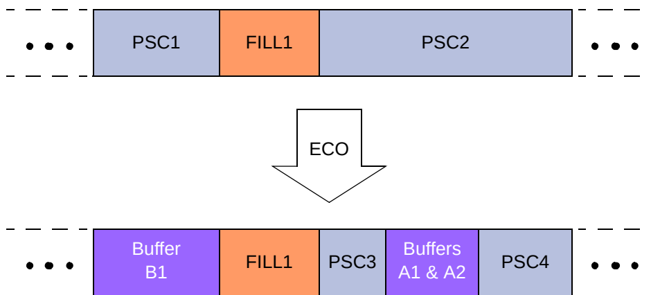
Figure 19-12 Freeze Silicon Site Row Cell Replacement
