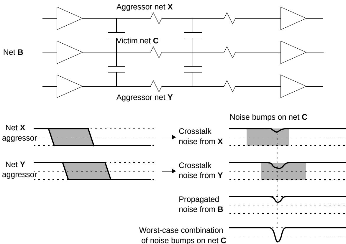
Figure 14-29 Combined effects of crosstalk and propagated noise
