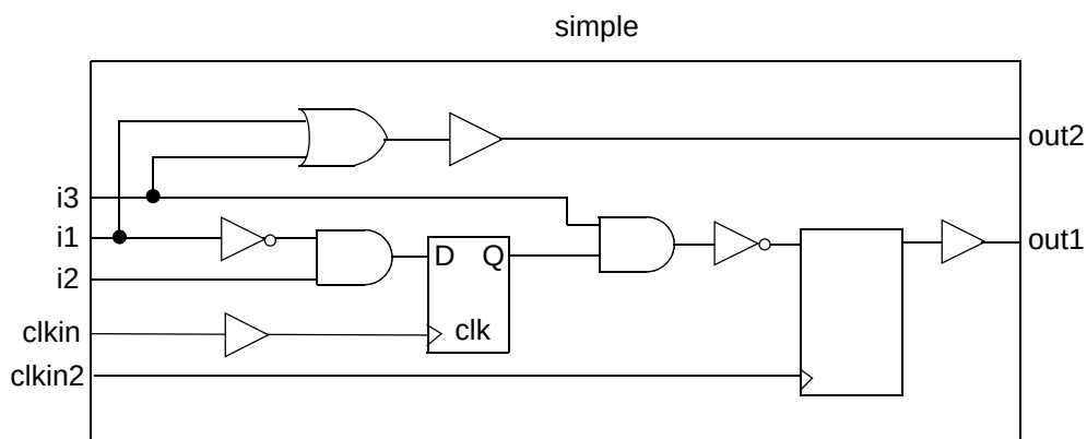
Figure 20-54 Gate-Level Netlist
