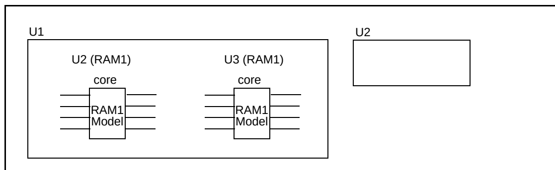
Figure 11-8 Mapping a design mode to a cell mode and cell instance
