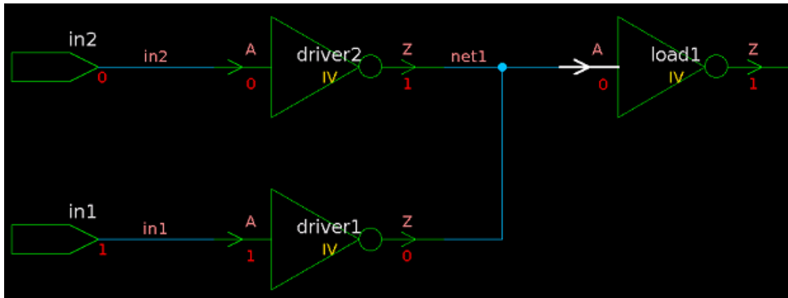
Figure 16-28 Schematic Showing Case Propagation
