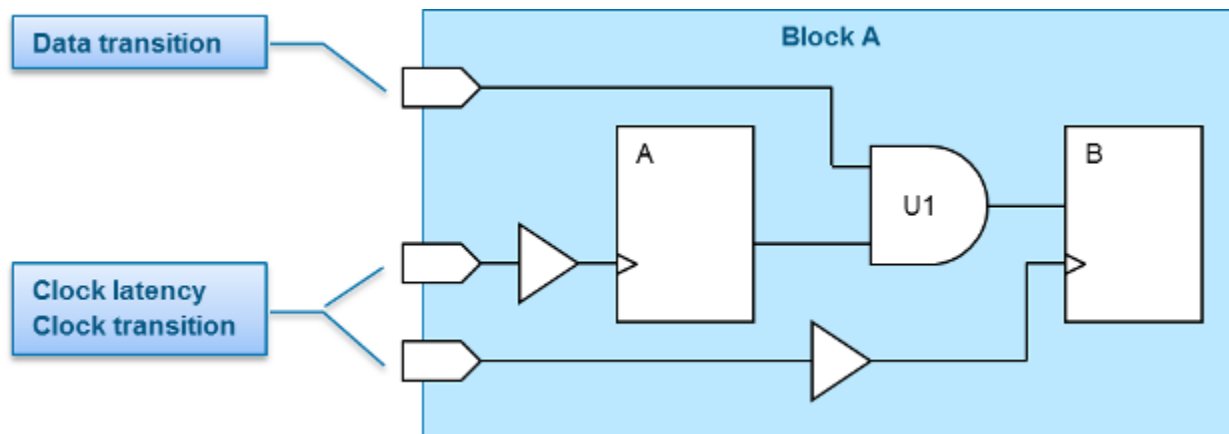
Figure 20-32 Top Context for Accurate Register-to-Register Path ECO Fixing
