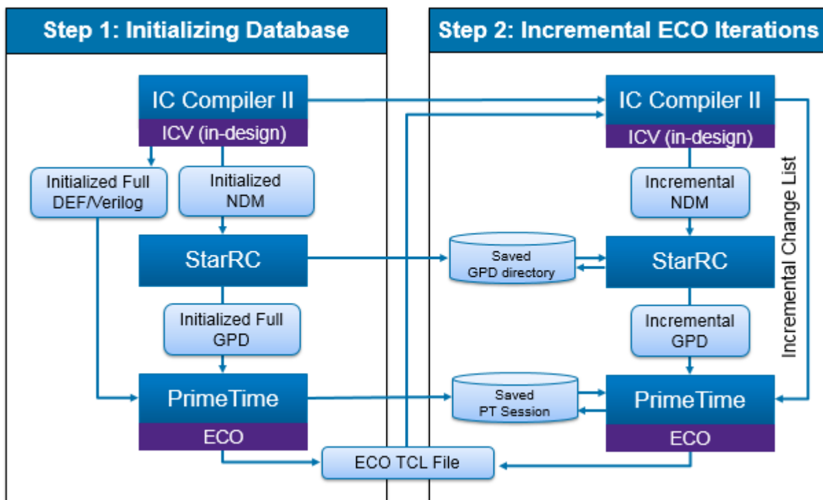
Figure 19-8 Galaxy Incremental ECO Flow Steps
