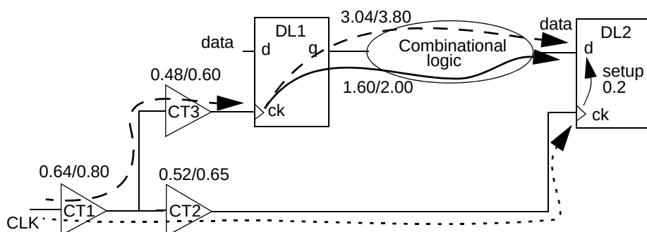
Figure 8-5 OCV for worst-case conditions
