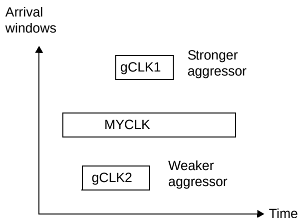
Figure 14-18 Crosstalk alignment diagram
