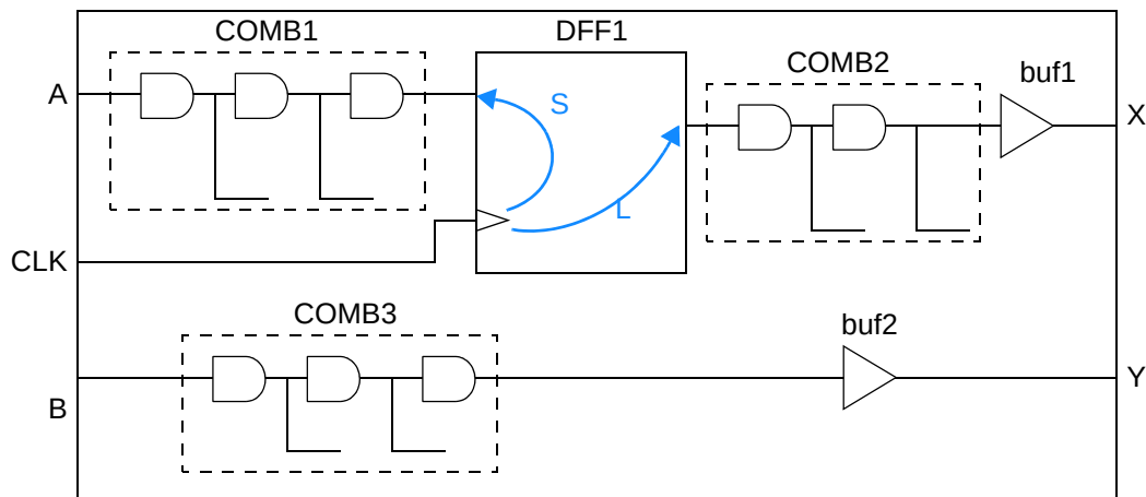
Figure 20-78 Quick timing model example
