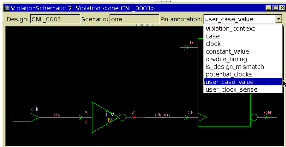
Figure 16-6 Schematic Viewer With Complete Pin Annotation List
