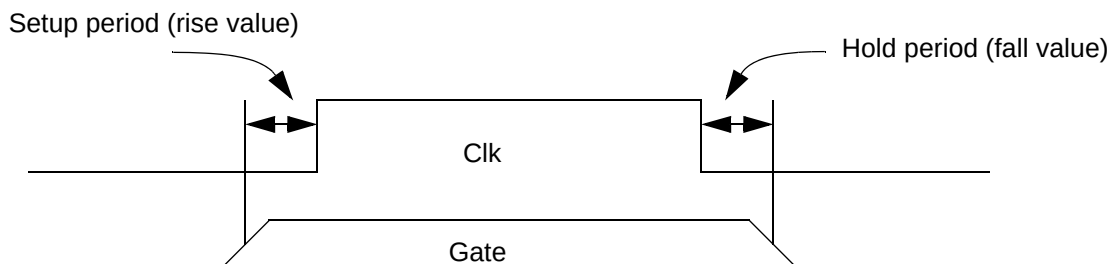
Figure 20-71 NOCHANGE_HIGH_HIGH arc
