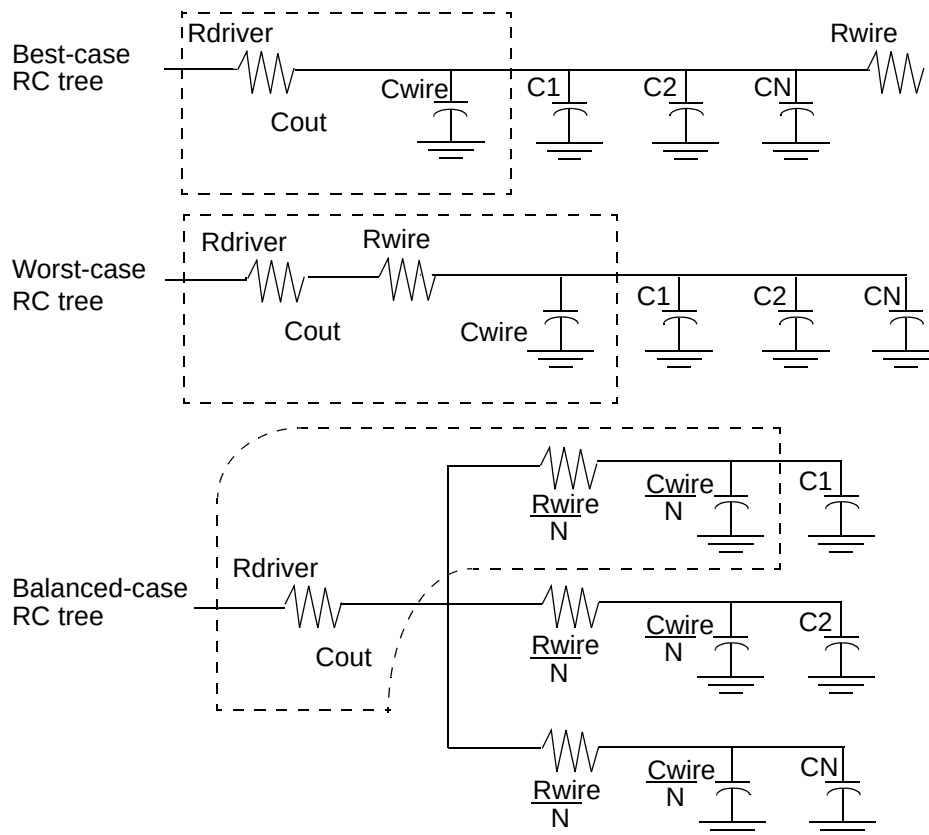
Figure 8-1 RC interconnect topologies for fanout of N
