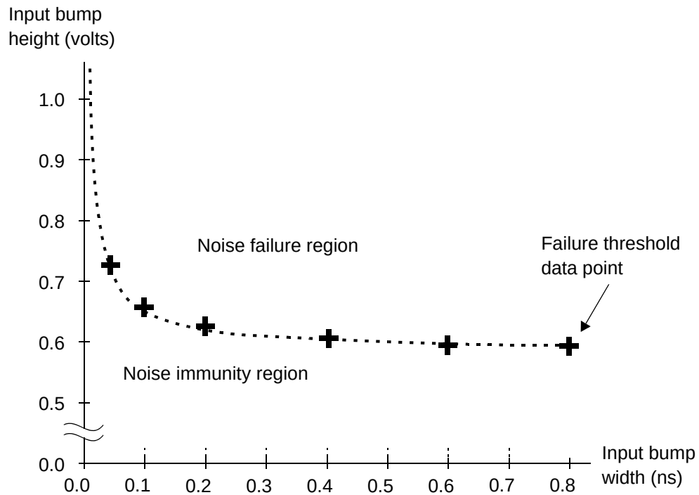
Figure 14-47 Input bump width versus height at failure thresholds
