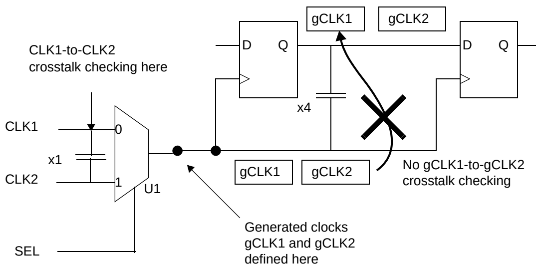
Figure 14-17 Circuit with multiplexed clocks
