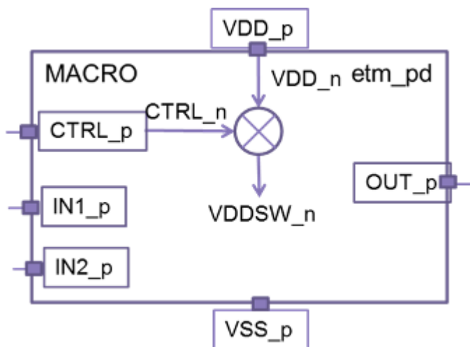
Figure 20-60 Simple multivoltage test design
