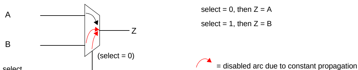
Figure 11-1 Constant propagation disables timing arcs
