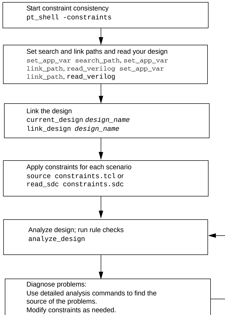
Figure 16-1 Typical Constraint Consistency Flow
