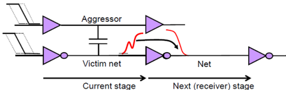
Figure 14-22 Crosstalk effect modeled as delta delay for current stage and fanout
