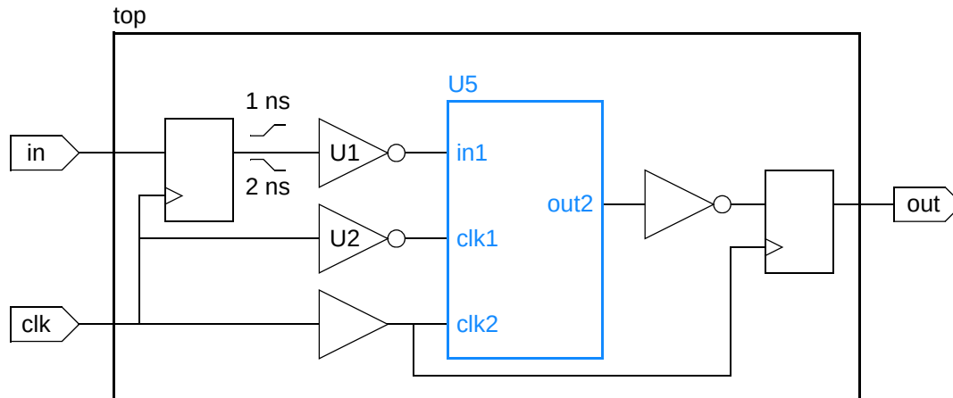
Figure 20-49 Context characterization example
