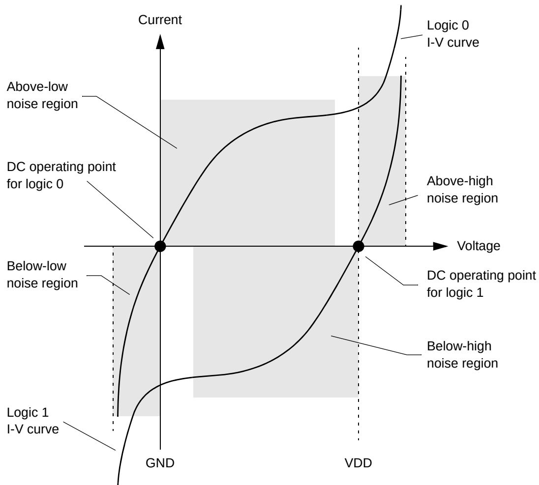
Figure 14-43 Steady-state I-V characteristics at a CMOS output
