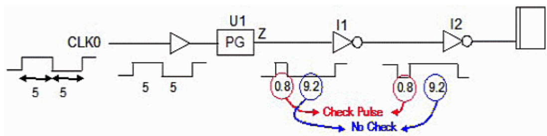
Figure 6-20 Sense propagation affects high and low pulse width propagation
