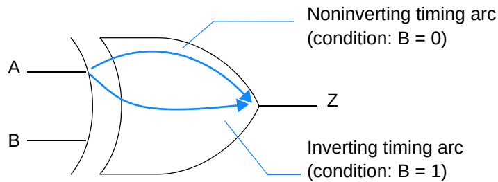
Figure 10-1 Example of state-dependent timing arcs
