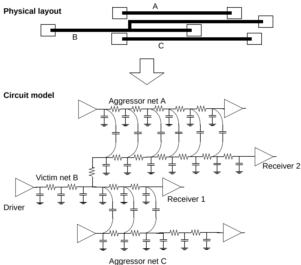
Figure 14-5 Detailed model of cross-coupled nets
