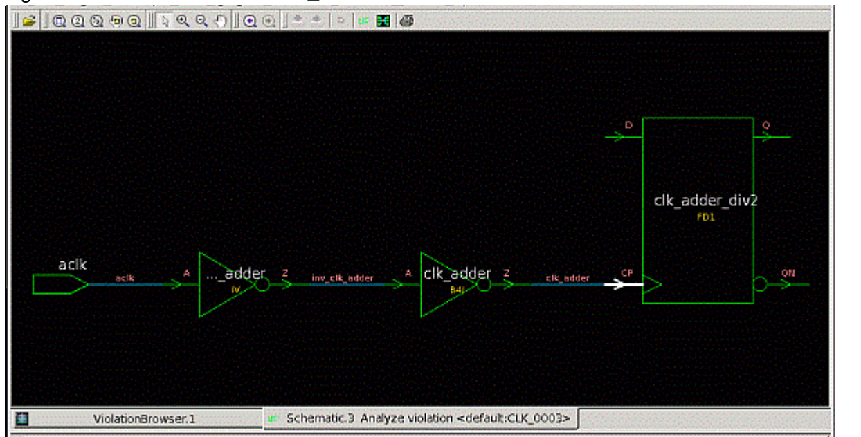
Figure 16-59 Schematic for CLK_0003 Rule Violation
