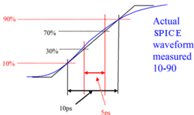
Figure 5-8 SPICE waveform
