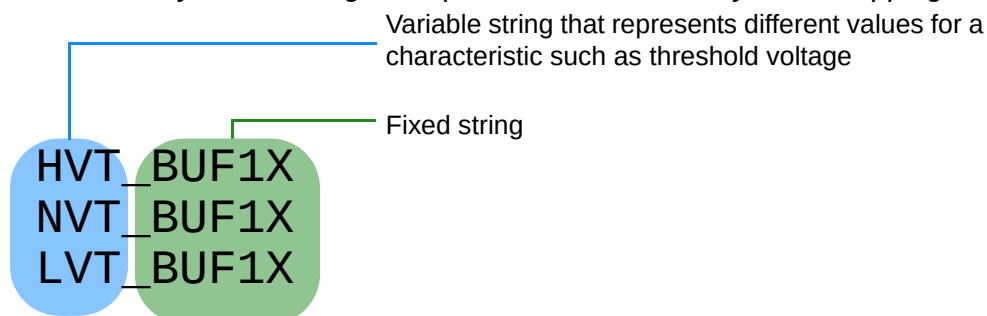
Figure 19-6 Library Cell Naming Example for Power Recovery Cell Swapping
