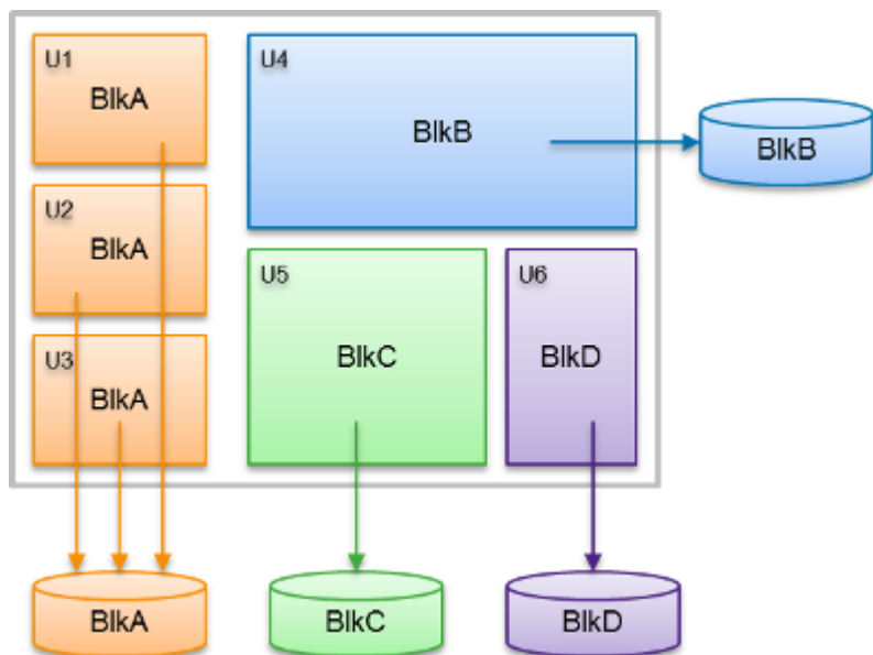
Figure 20-19 Design with multiply instantiated modules
