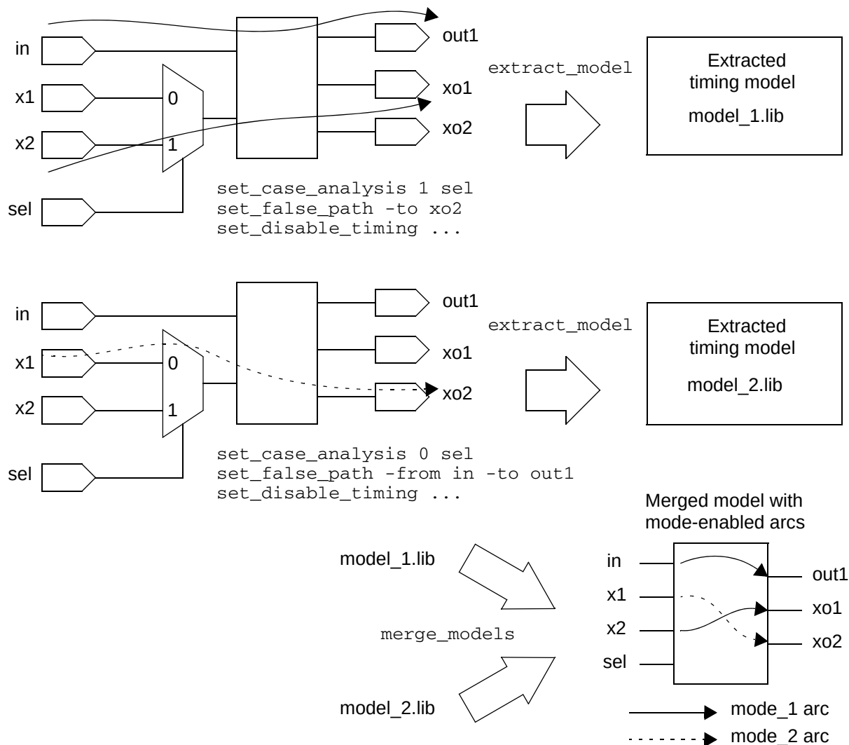
Figure 20-68 Model extraction and merging example
