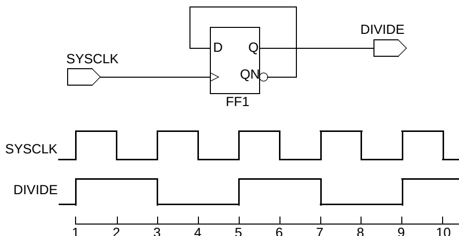
Figure 6-24 Divide-by-2 clock generator
