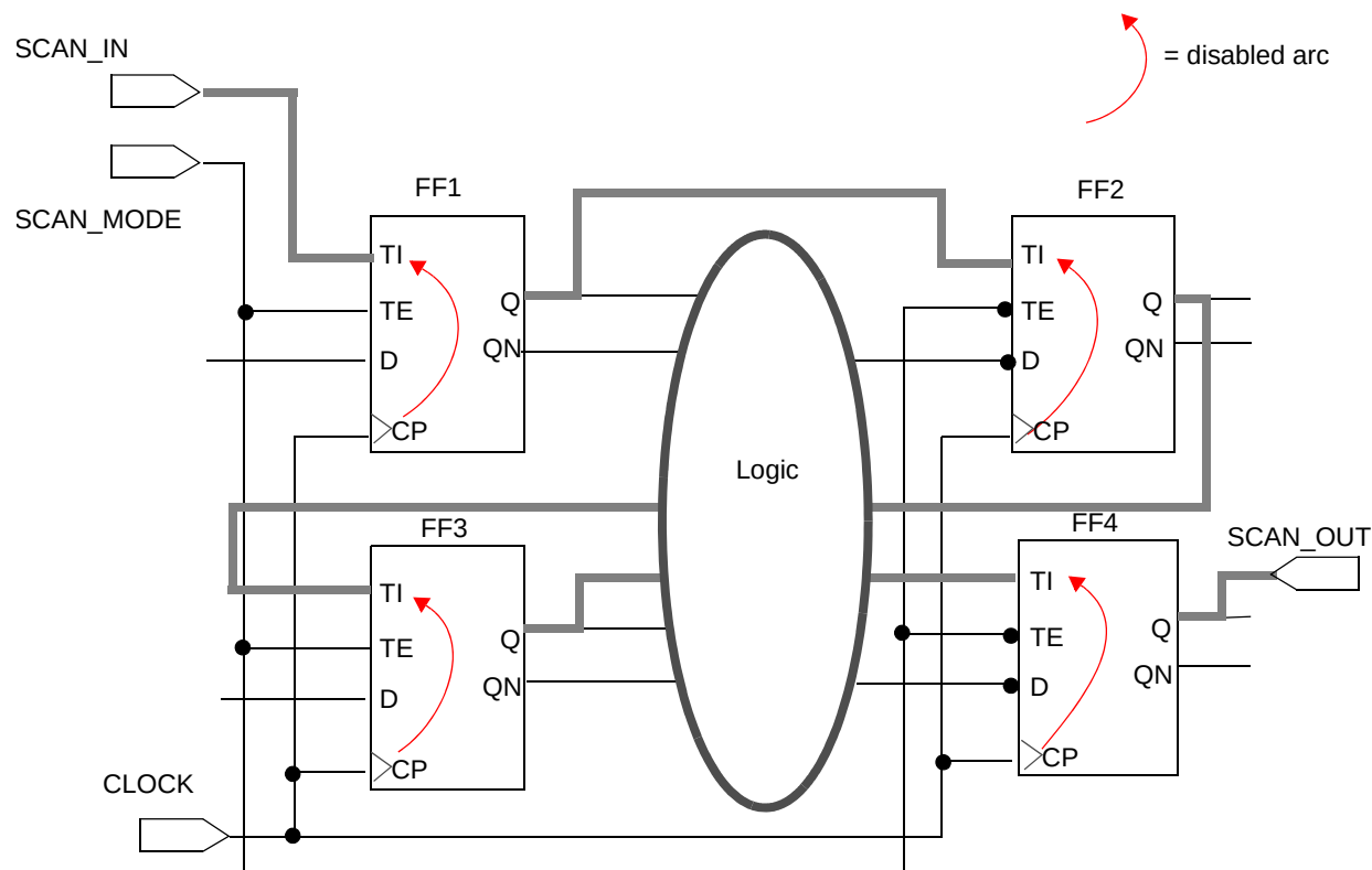
Figure 11-5 Scan chain that starts at SCAN_IN and ends at SCAN_OUT
