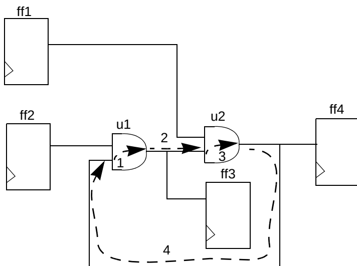
Figure 15-4 Loop breaking example
