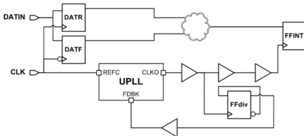
Figure 6-21 Circuit example
