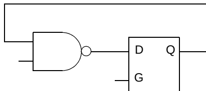
Figure 5-11 Self-looping latch
