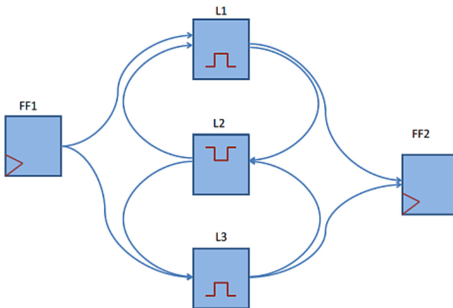
Figure 15-25 Single latch loop group with three latches
