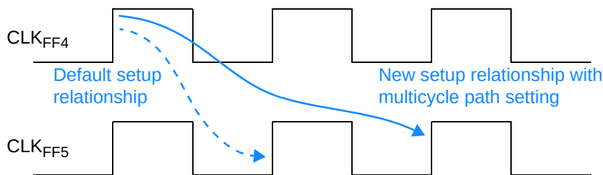
Figure 7-13 Multicycle path setup relationship
