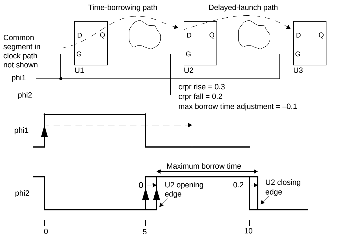
Figure 15-22 Maximum borrow time adjustment for CRPR
