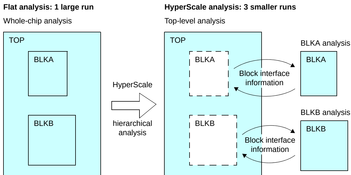
Figure 20-2 Flat Analysis Versus HyperScale Hierarchical Analysis
