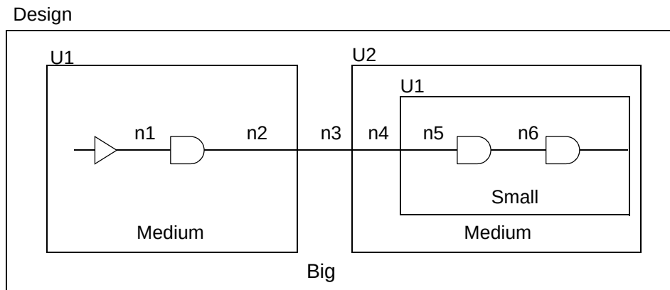
Figure 5-6 Design example for wire load mode settings
