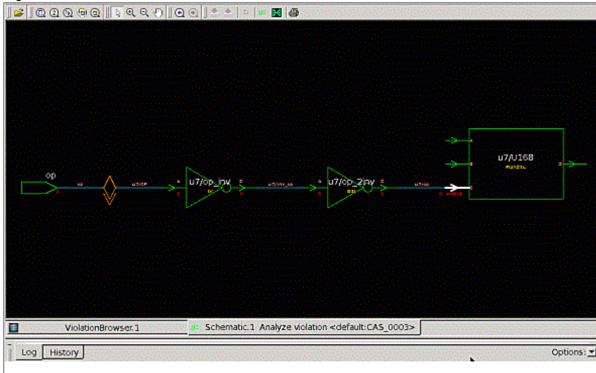
Figure 16-55 Schematic View of CAS_0003 Rule Violation
