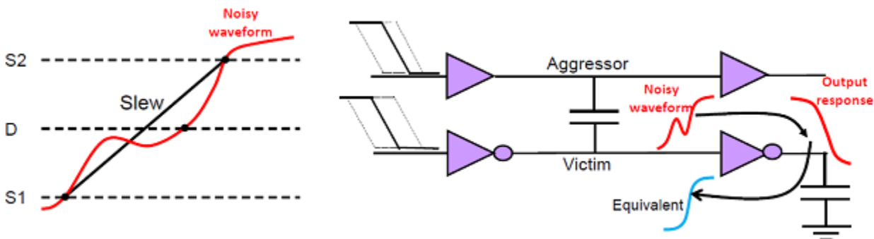
Figure 14-23 Equivalent waveform calculation
