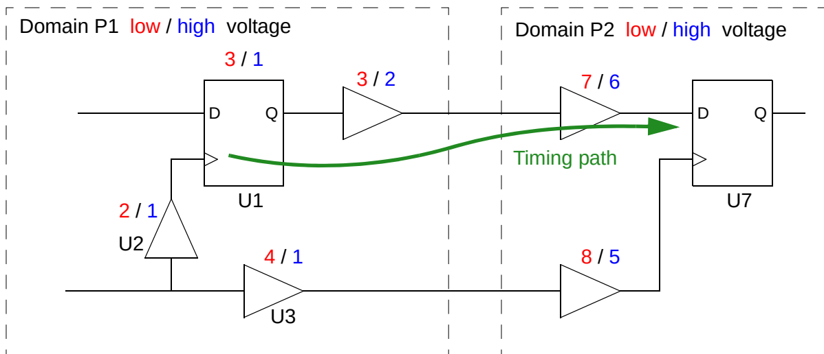
Figure 13-5 Simultaneous multivoltage slack calculation
