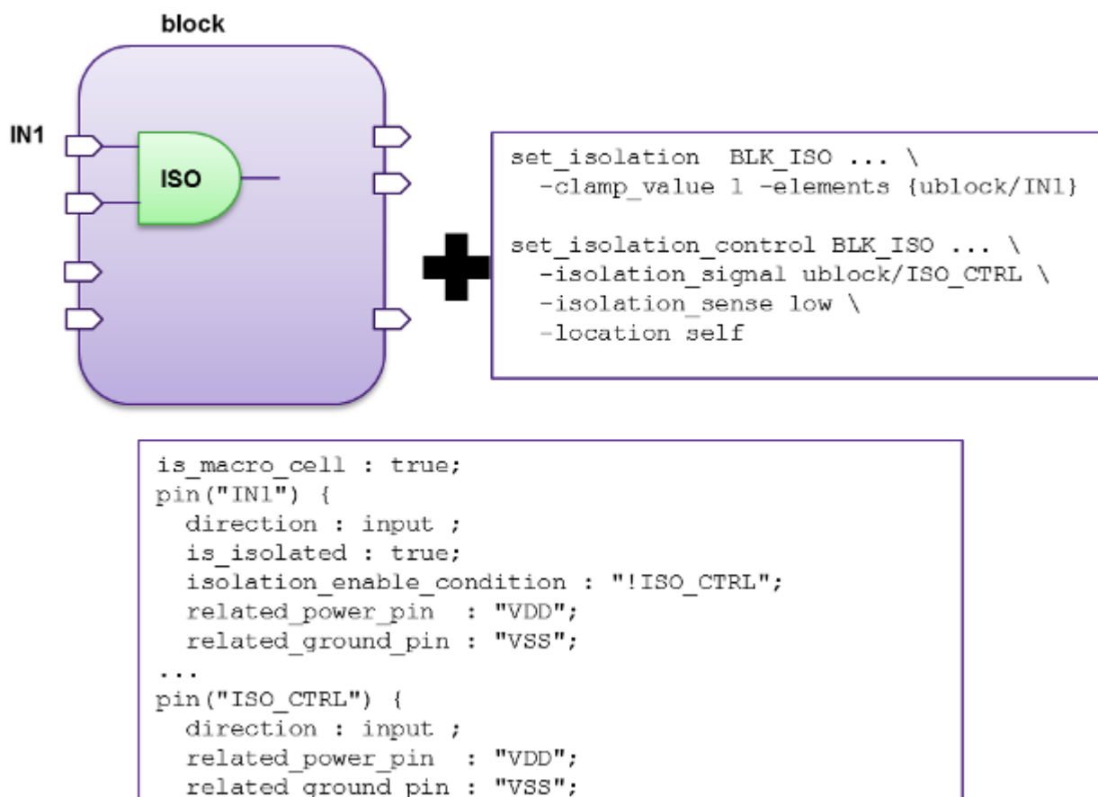
Figure 20-61 Isolation attributes
