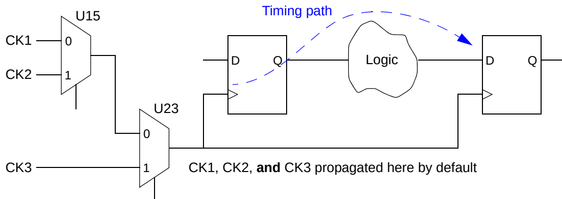
Figure 6-13 Multiplexed Clocks
