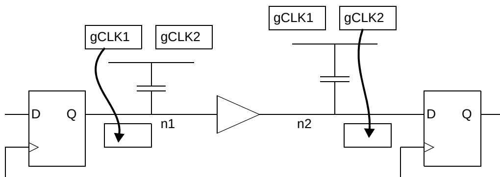
Figure 14-19 Different exclusive aggressors on a path
