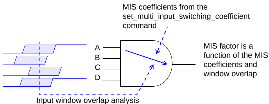
Figure 9-10 Actual MIS factor is determined by the window overlap and MIS coefficients
