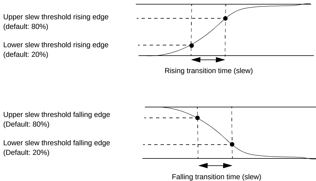
Figure 9-6 Slew transition points
