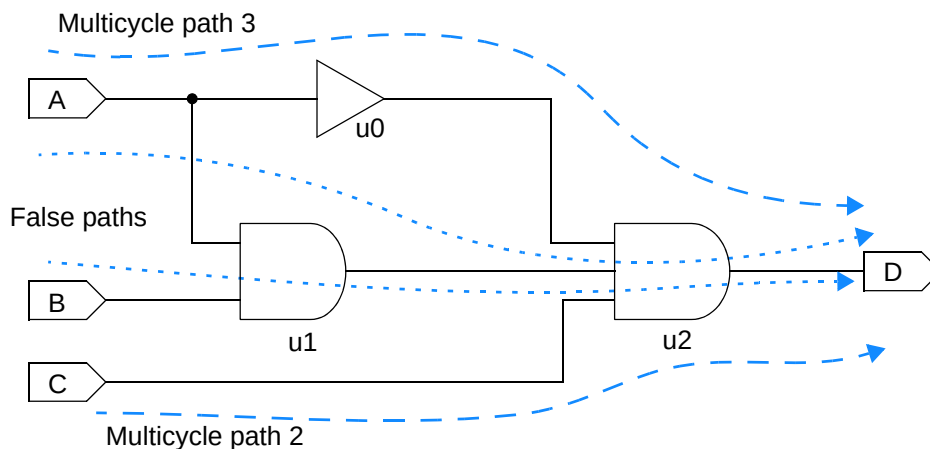
Figure 7-19 Design to demonstrate transformed exceptions
