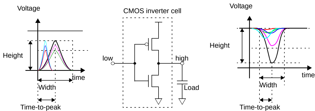
Figure 14-52 Noise propagation characterization
