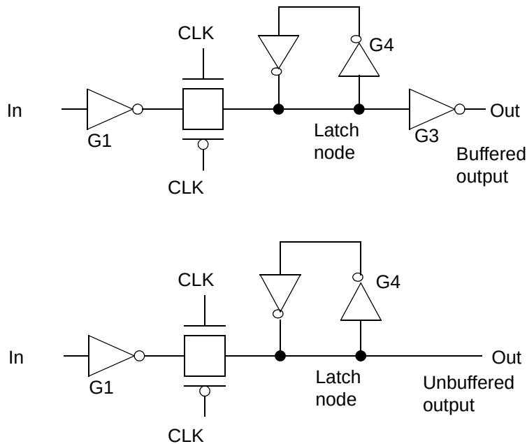
Figure 14-40 Latch circuits with buffered and unbuffered outputs
