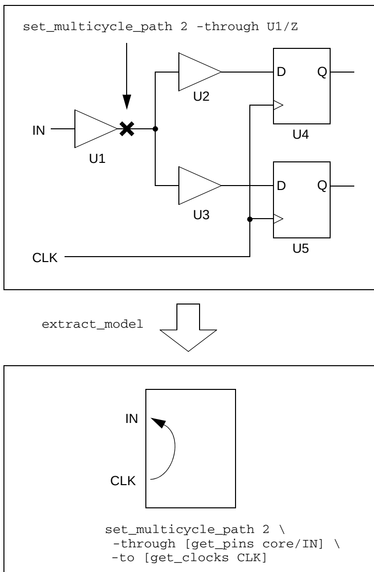
Figure 20-64 Multicycle path extraction with an output_mcp.pt file
