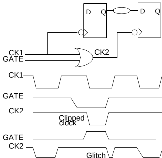
Figure 6-23 Clock-gating hold violations
