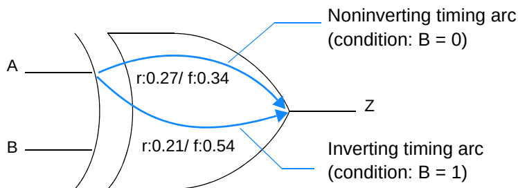
Figure 10-3 Annotated delays when the Synopsys Library contains conditions
