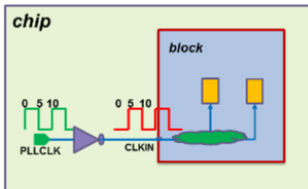
Figure 20-22 Sense-aware clock mapping and data capturing
