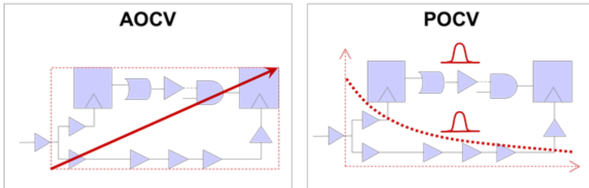
Figure 12-1 Comparison of AOCV and POCV
