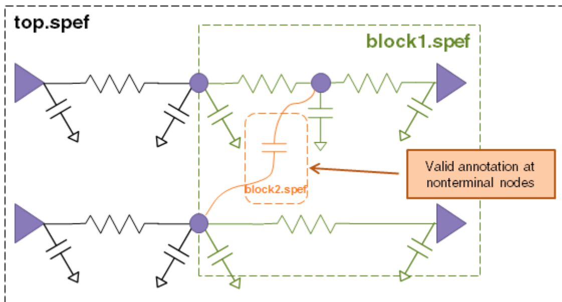
Figure 10-10 Second annotation is valid
