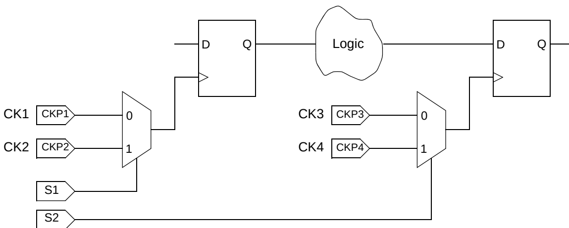
Figure 6-11 Four clocks and two selection signals
