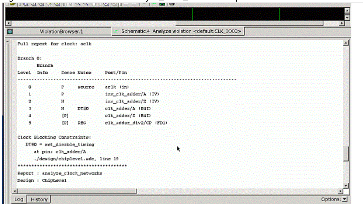
Figure 16-61 Partial View of the analyze_clock_networks Report in GUI Console
