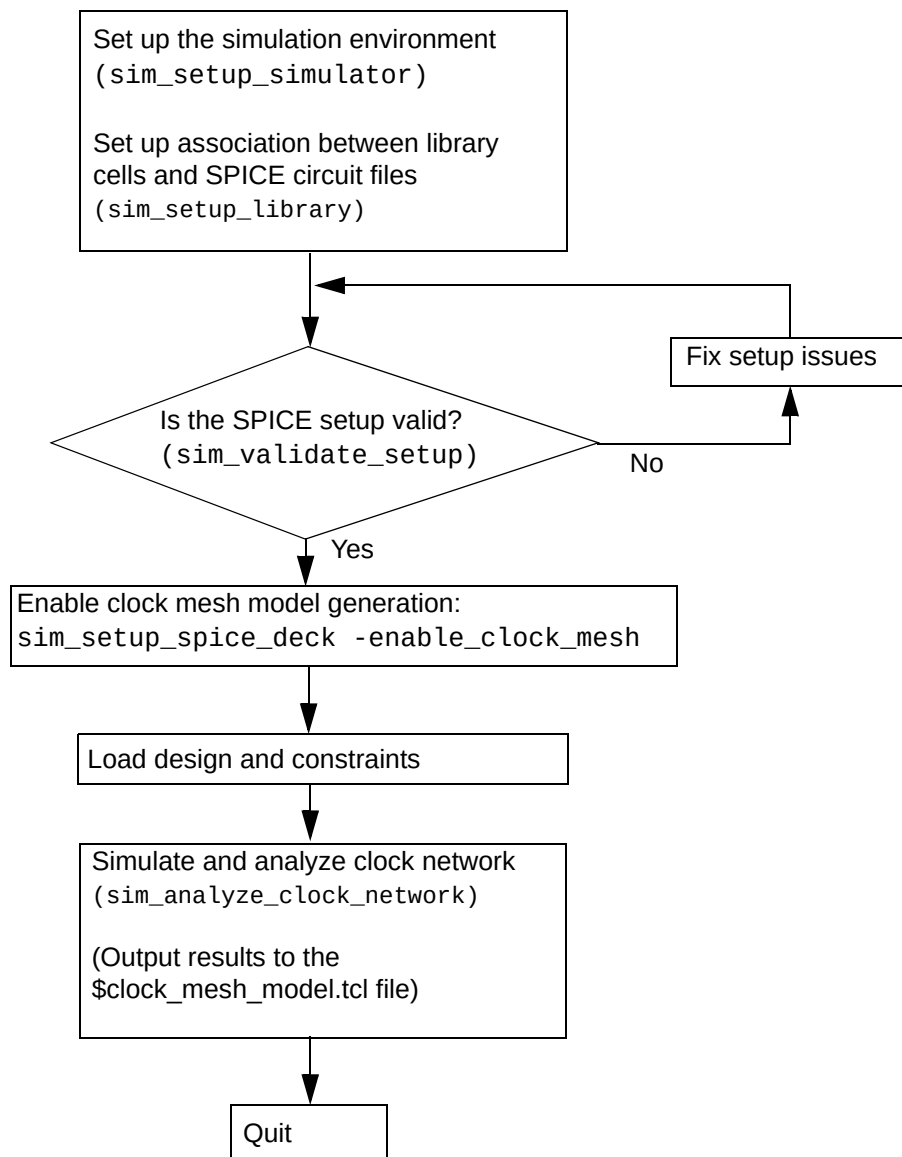
Figure 6-32 Generating the clock mesh model
