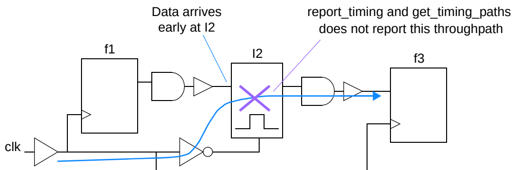
Figure 15-31 Filtering throughpaths with the timing_report_skip_early_paths_at_intermediate_latches variable
