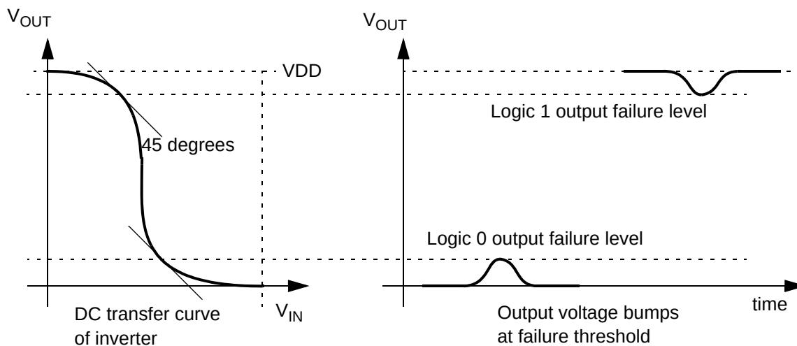
Figure 14-45 Noise immunity failure definition
