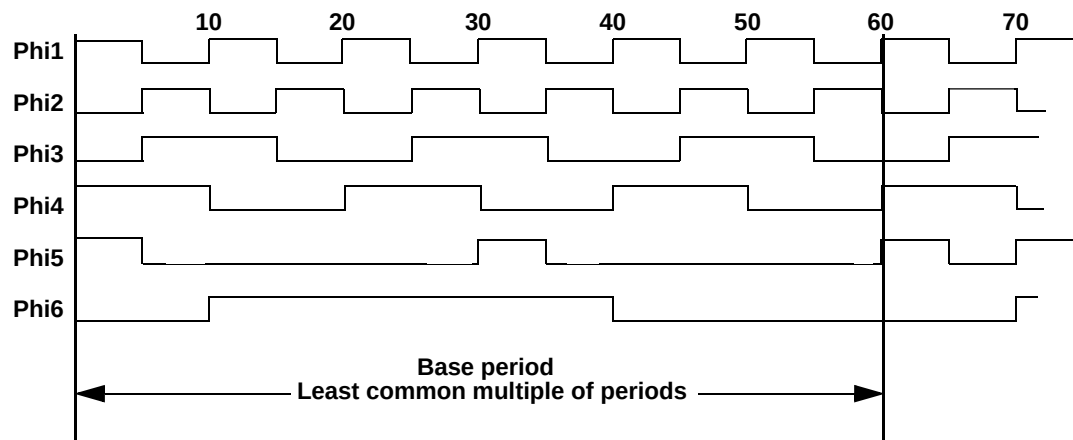
Figure 15-2 Base period of clocks
