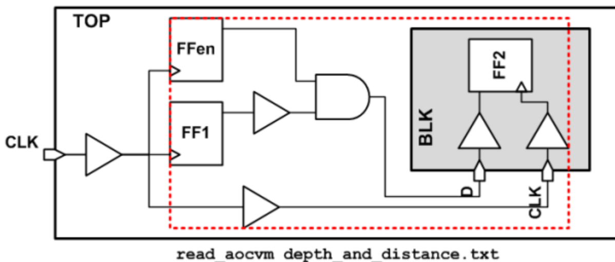
Figure 20-47 AOCV modeling
