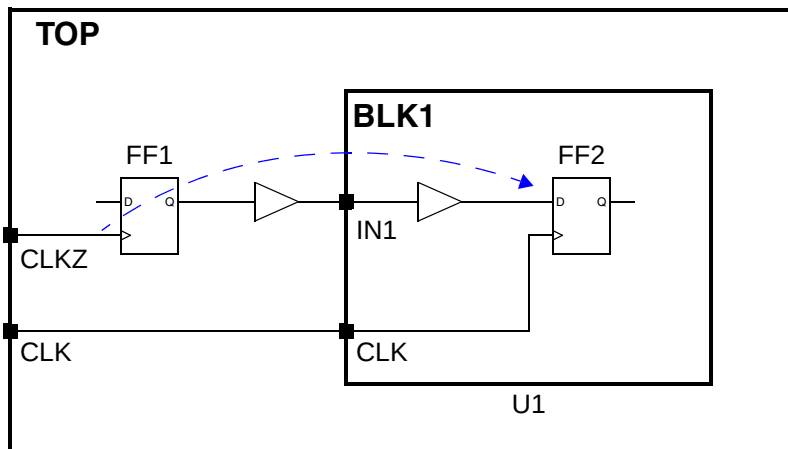
Figure 20-16 Clock Matching Issue in a Bottom-Up Flow
