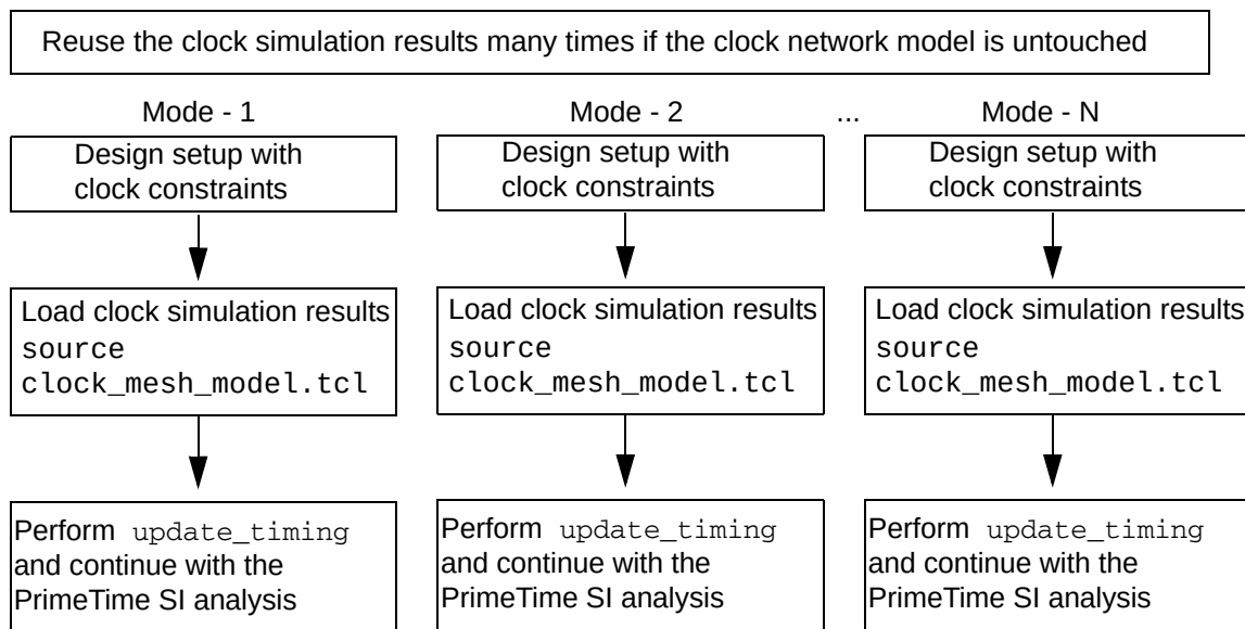
Figure 6-33 Reusing the clock mesh model in PrimeTime analysis
