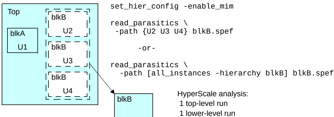
Figure 20-20 MIM Merging for All Instances of a Block
