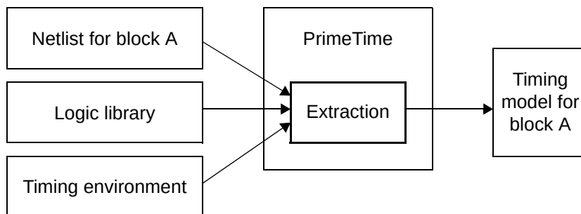
Figure 20-53 Timing model extraction process
