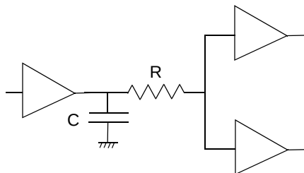
Figure 10-6 Lumped RC
