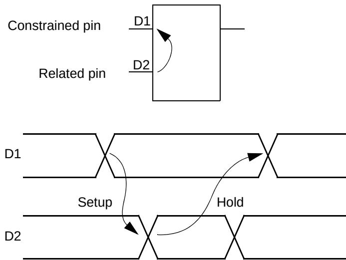
Figure 15-10 Data checks on rising and falling edges
