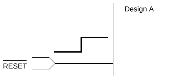
Figure 11-3 Setting case analysis with a rising transition
