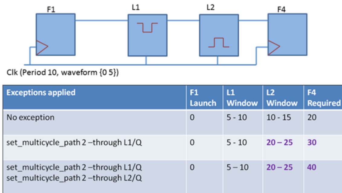
Figure 15-27 Multicycle path exceptions affect the downstream latch windows
