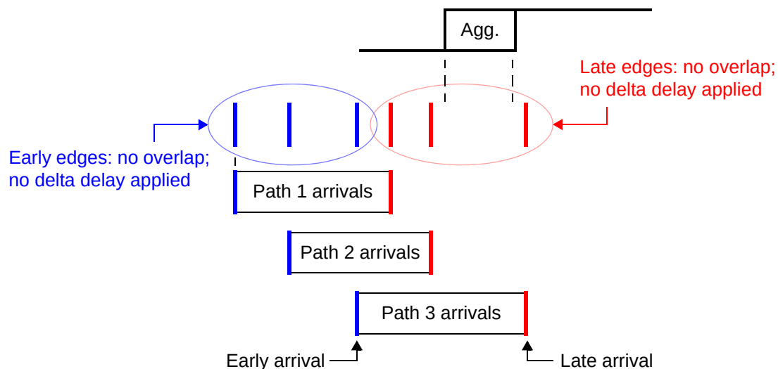
Figure 14-15 “All Path Edges” Overlap Mode, Aggressor Window Between Edges
