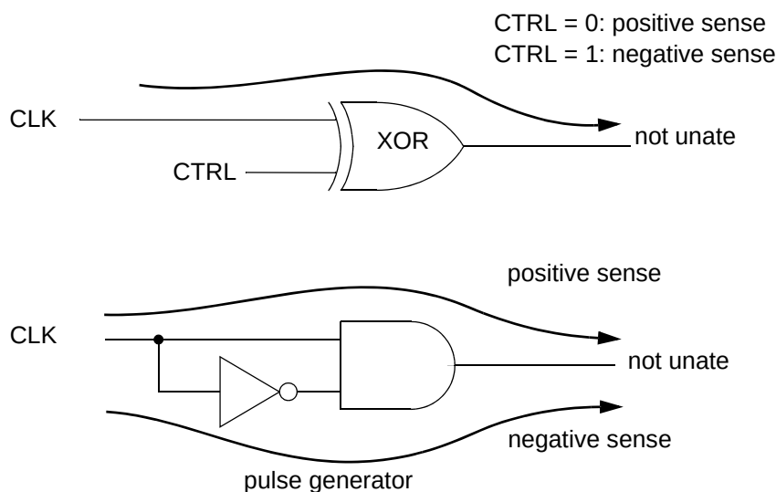
Figure 6-16 Non-unate clock signals
