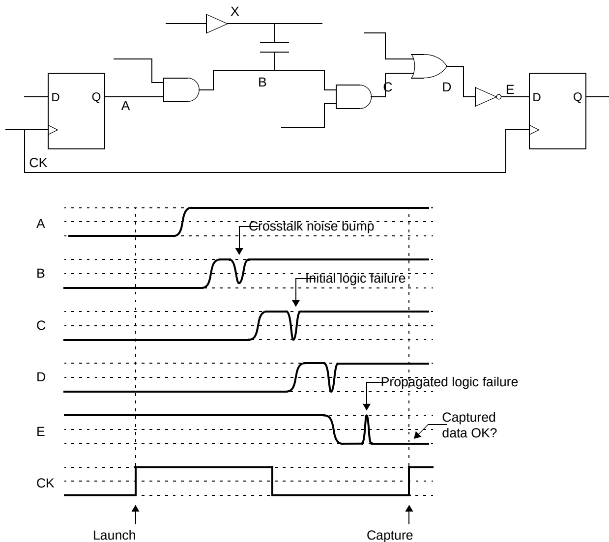
Figure 14-32 Propagated logic failure
