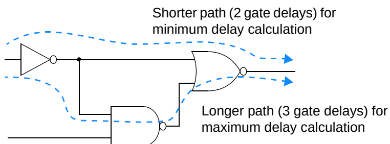
Figure 1-3 Multiple paths through combinational logic
