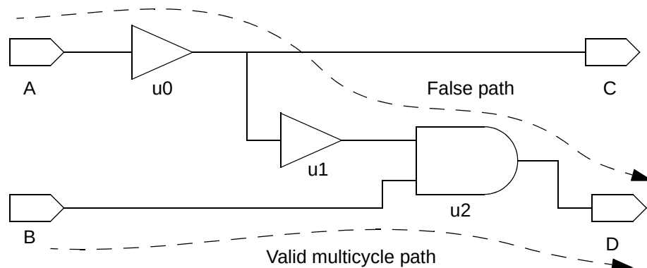
Figure 7-18 Design to demonstrate ignored exceptions
