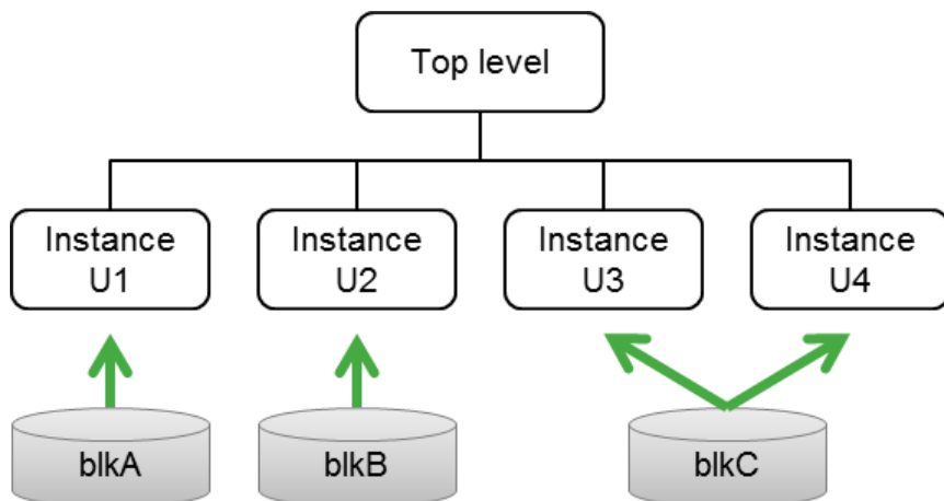
Figure 20-17 Design example with two levels of hierarchy
