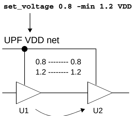
Figure 13-2 Signal level checking with supply correlation
