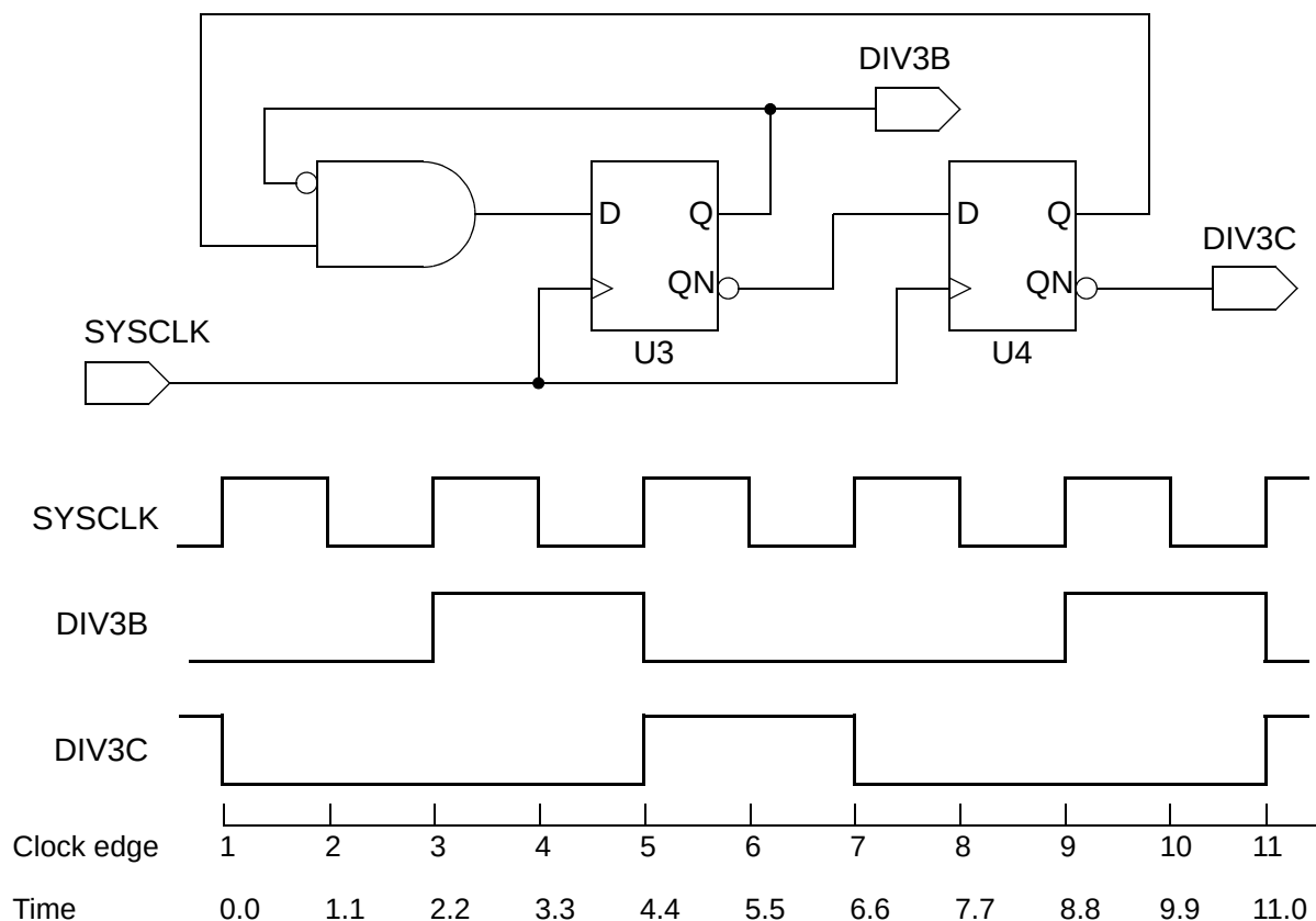
Figure 6-29 Generated divide-by-3 clock with shifted edges
