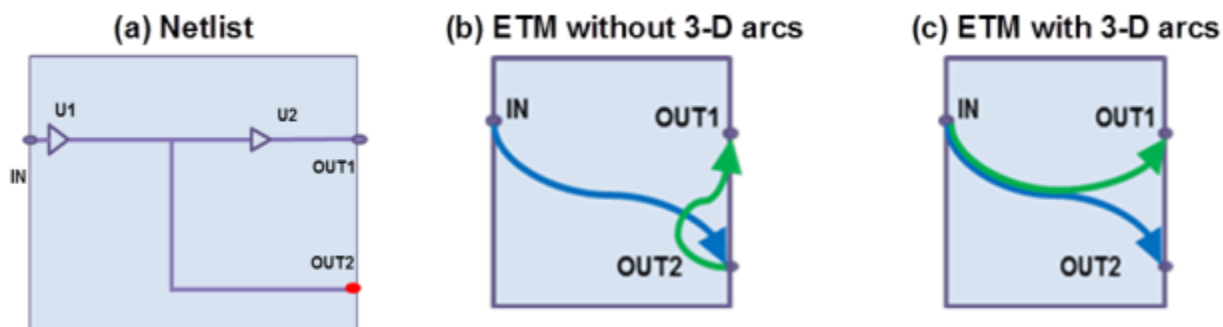
Figure 20-62 ETM extraction on a netlist with tapped output ports
