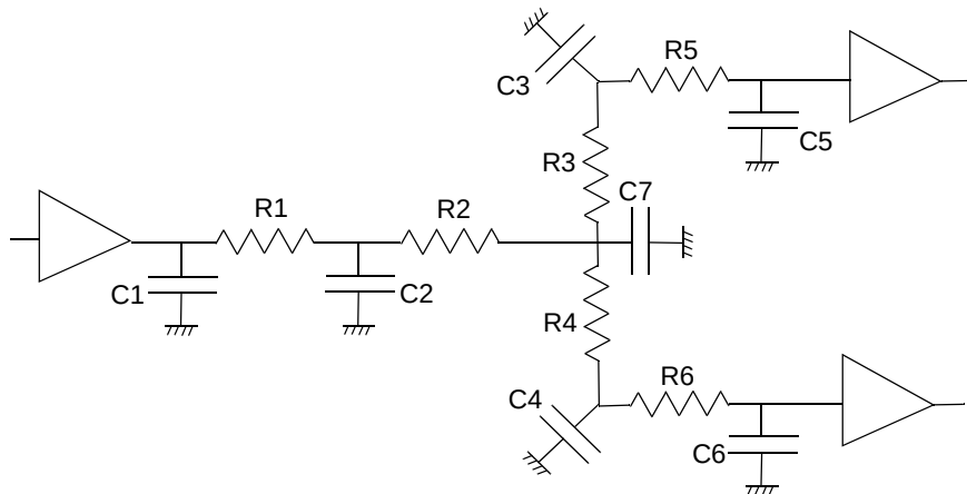
Figure 10-7 Detailed RC
