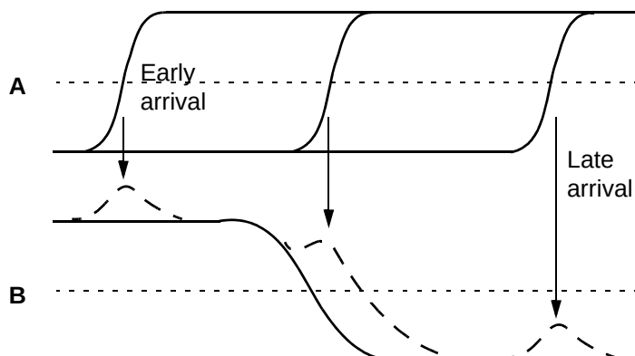
Figure 14-4 Effects of crosstalk at different arrival times
