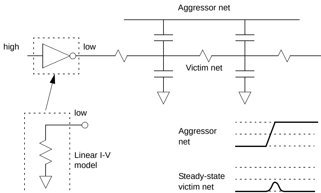
Figure 14-41 Linear I-V model for a cell with steady-state low output
