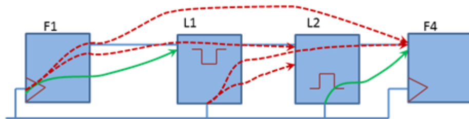
Figure 15-26 False path exceptions on throughpaths
