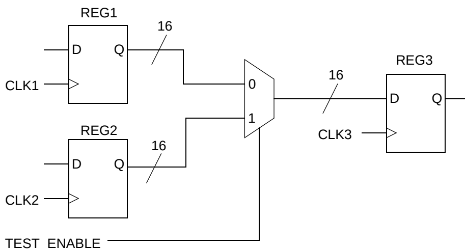
Figure 7-17 Multiplexed register paths
