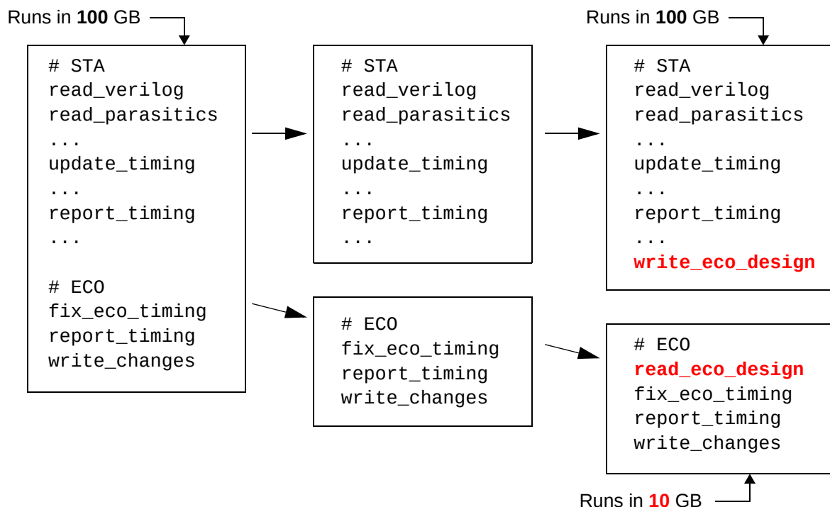
Figure 19-9 Single-Scenario Reduced-Resource ECO Flow
