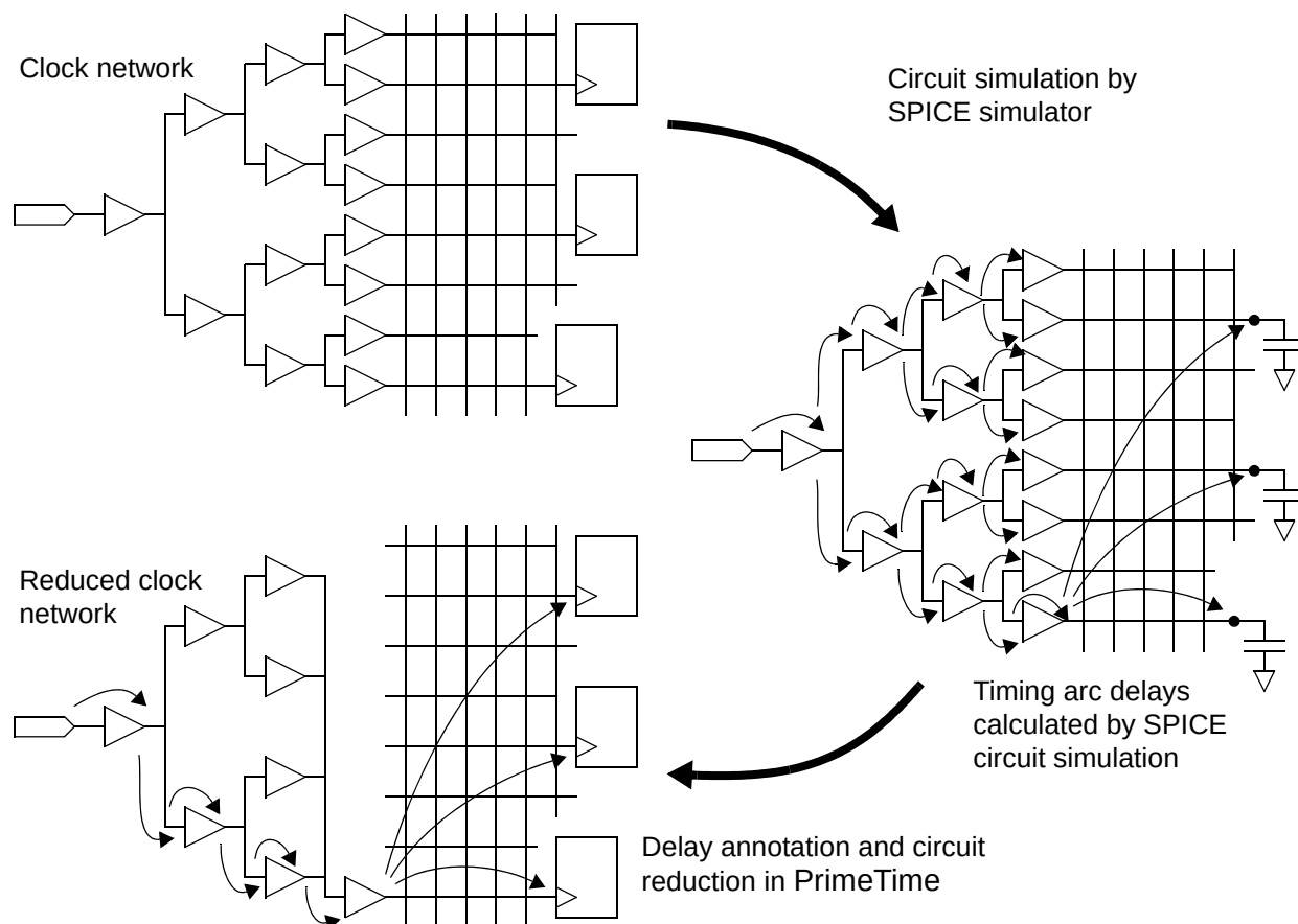
Figure 6-30 Clock mesh analysis and circuit reduction
