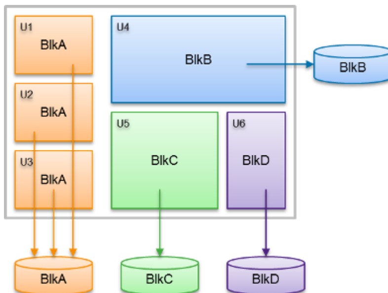
Figure 20-18 Design with multiply instantiated modules
