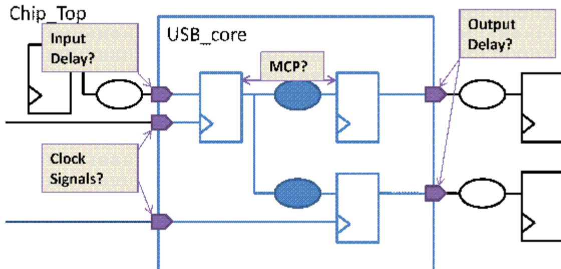
Figure 16-23 Block Design USB_core Inside Design Chip_Top
