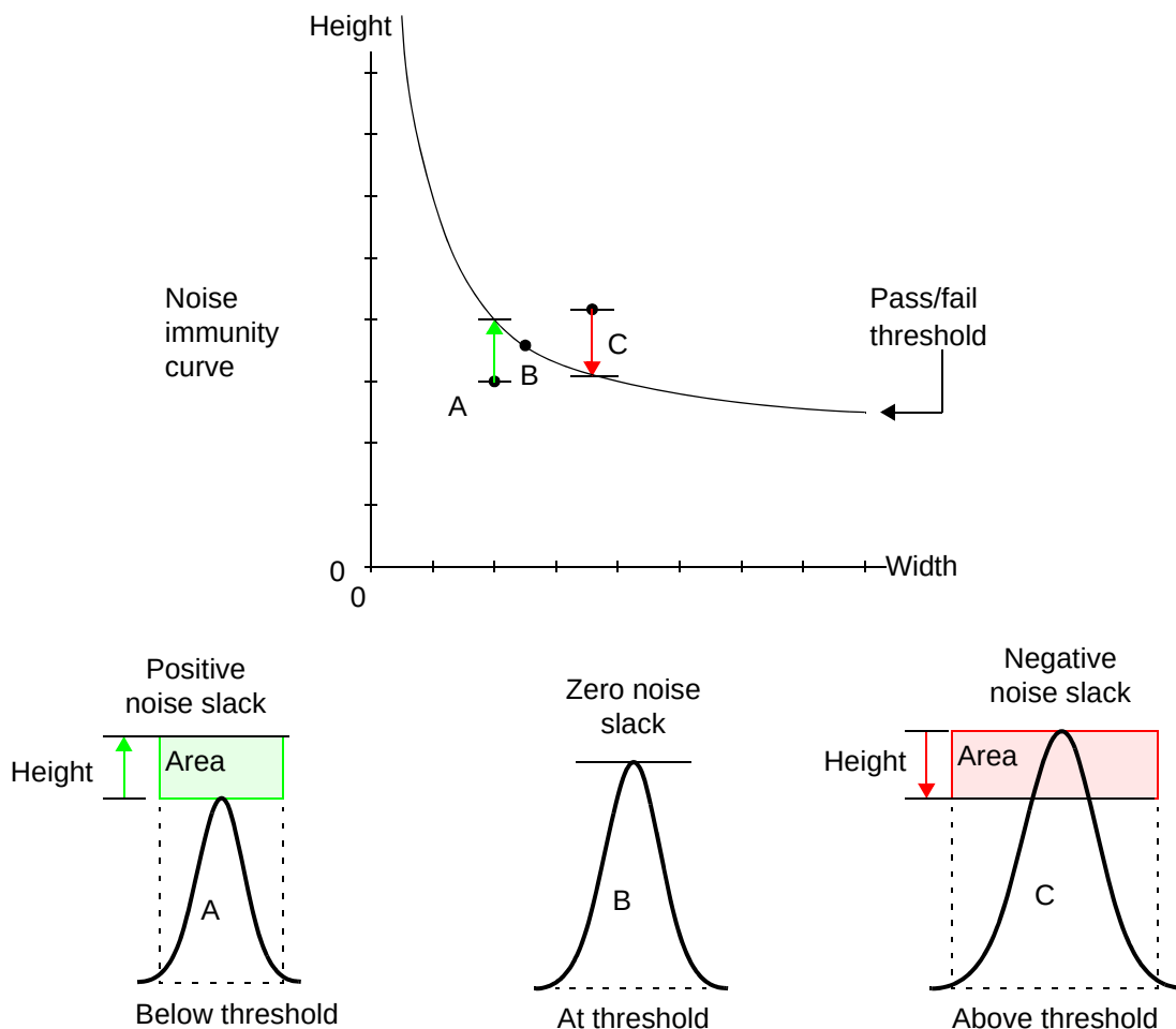
Figure 14-50 Noise slack calculation
