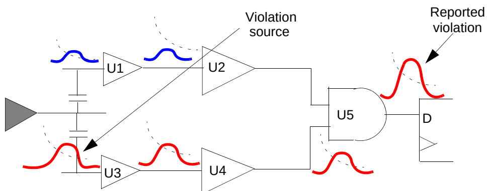
Figure 14-35 Report at endpoint
