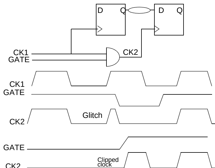
Figure 6-22 Clock-gating setup violations
