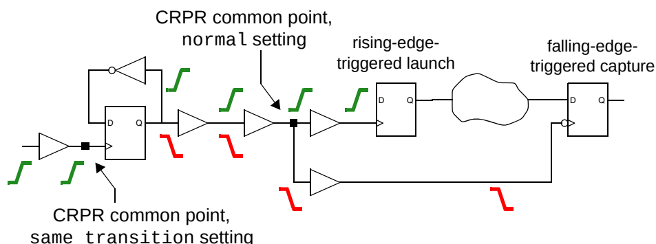
Figure 8-13 Common Point for Different timing_clock_reconvergence_pessimism Settings
