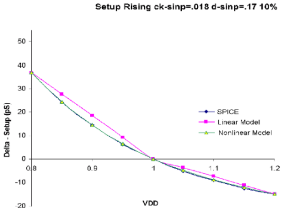
Figure 9-5 Nonlinear interpolation of timing constraint
