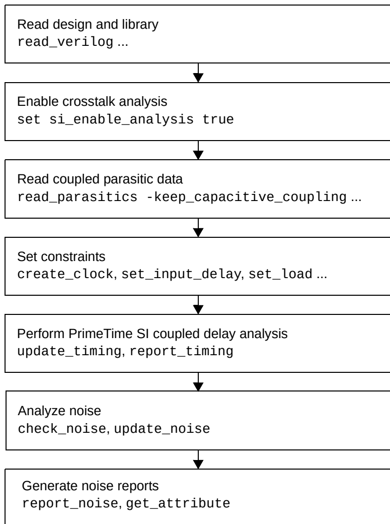
Figure 14-33 Noise analysis flows
