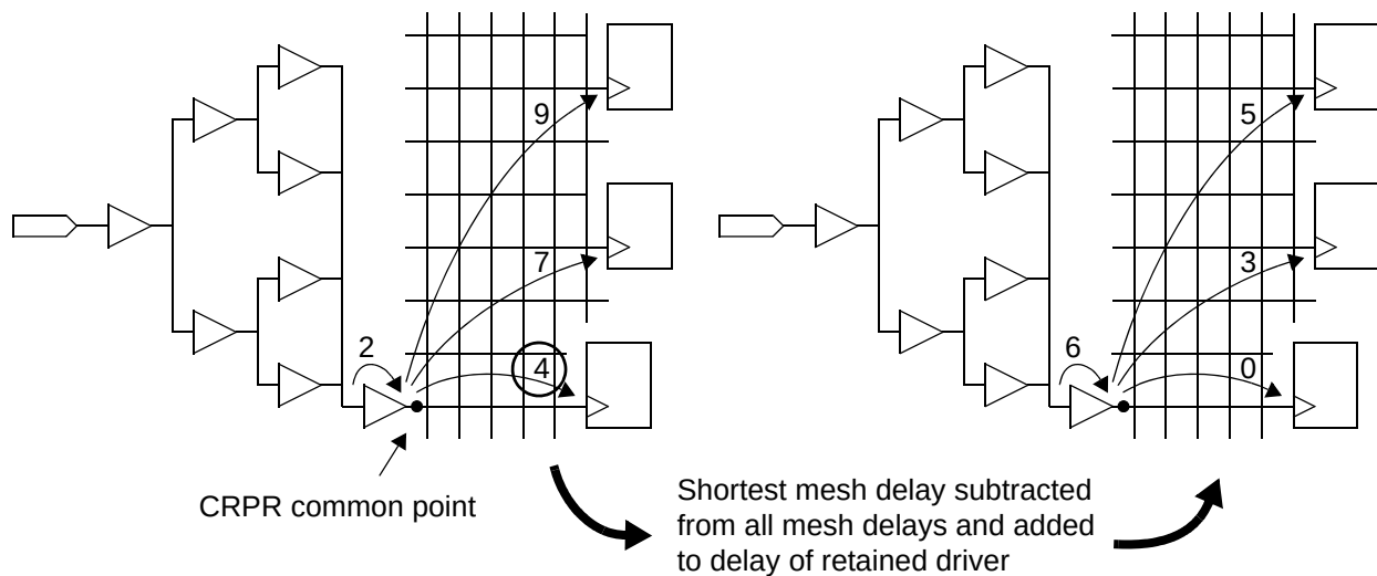
Figure 6-31 Clock reconvergence pessimism removal from mesh
