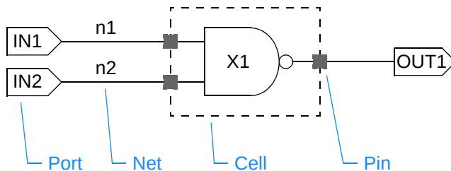
Figure 4-1 Typical design objects
