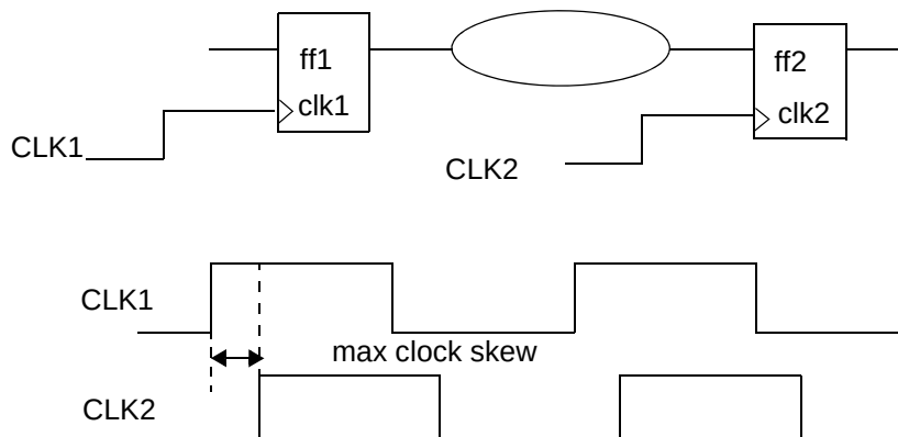
Figure 6-5 Example of interclock uncertainty
